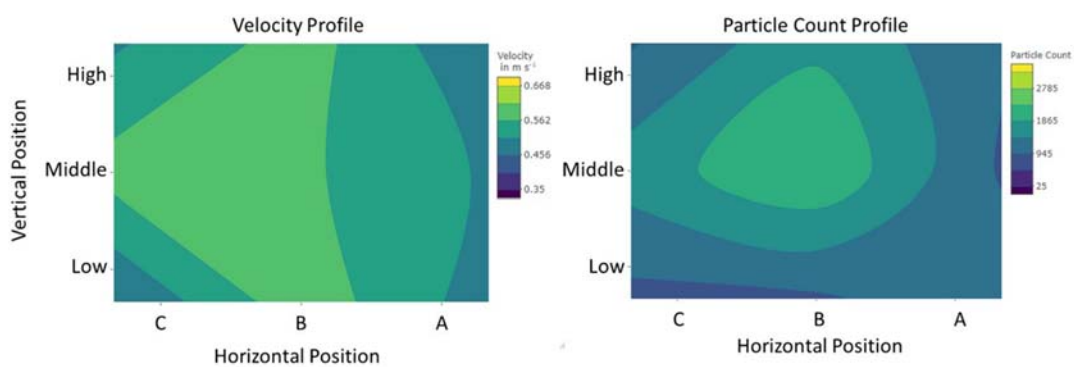
Figure S34. Velocity and Particle Count Profiles in Plane 10 at 0.5 \text{ m s}^{-1}
