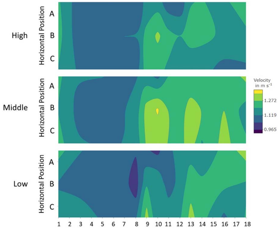
Figure S16. Vertical Velocity Profile of the Chamber at 1.0 \text{ m s}^{-1} (60 Hz), no Flow Straightener
