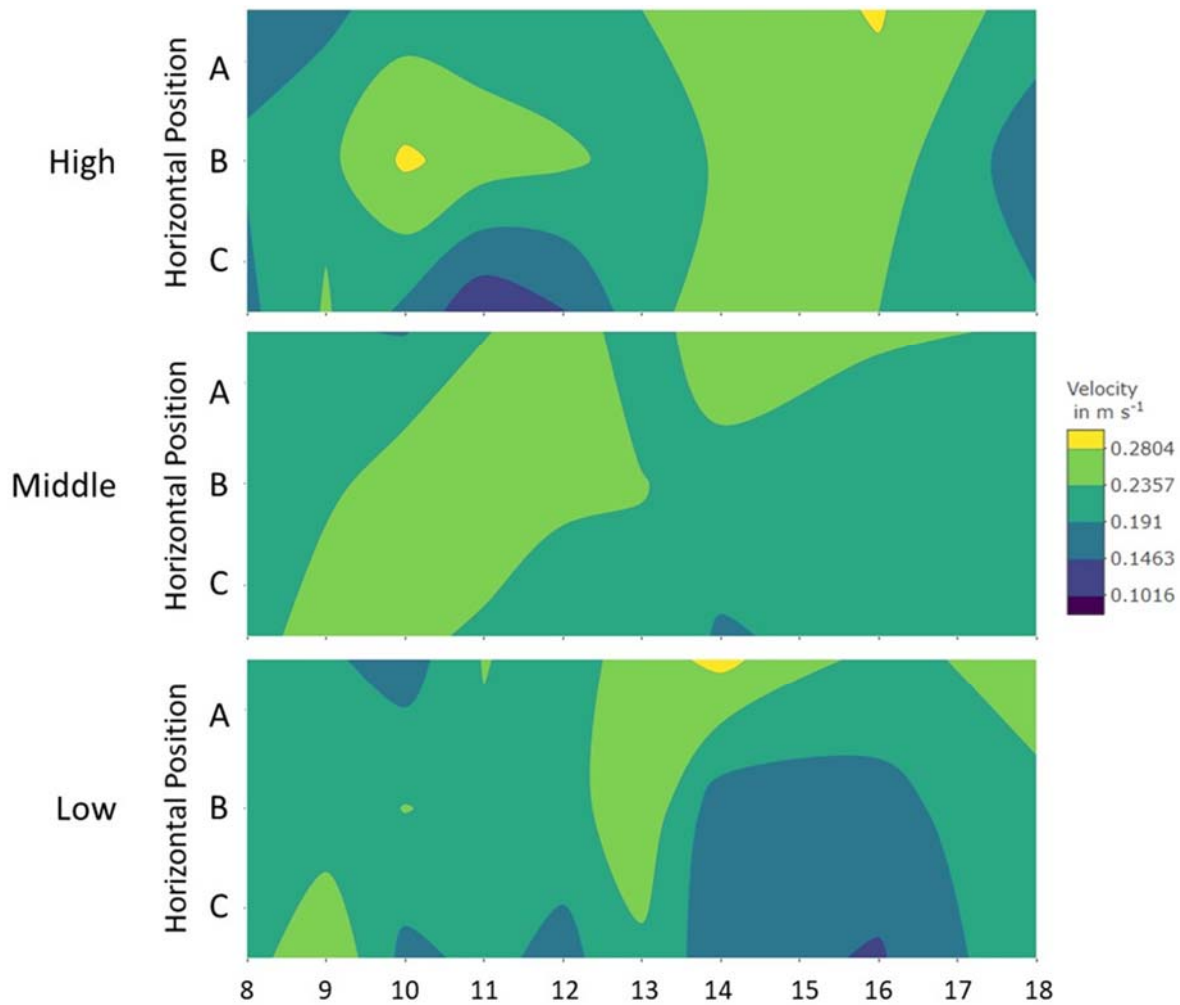
Figure S17. Vertical Velocity Profile of the Chamber at 0.2 \text{ m s}^{-1} (16 Hz), with Flow Straightener
