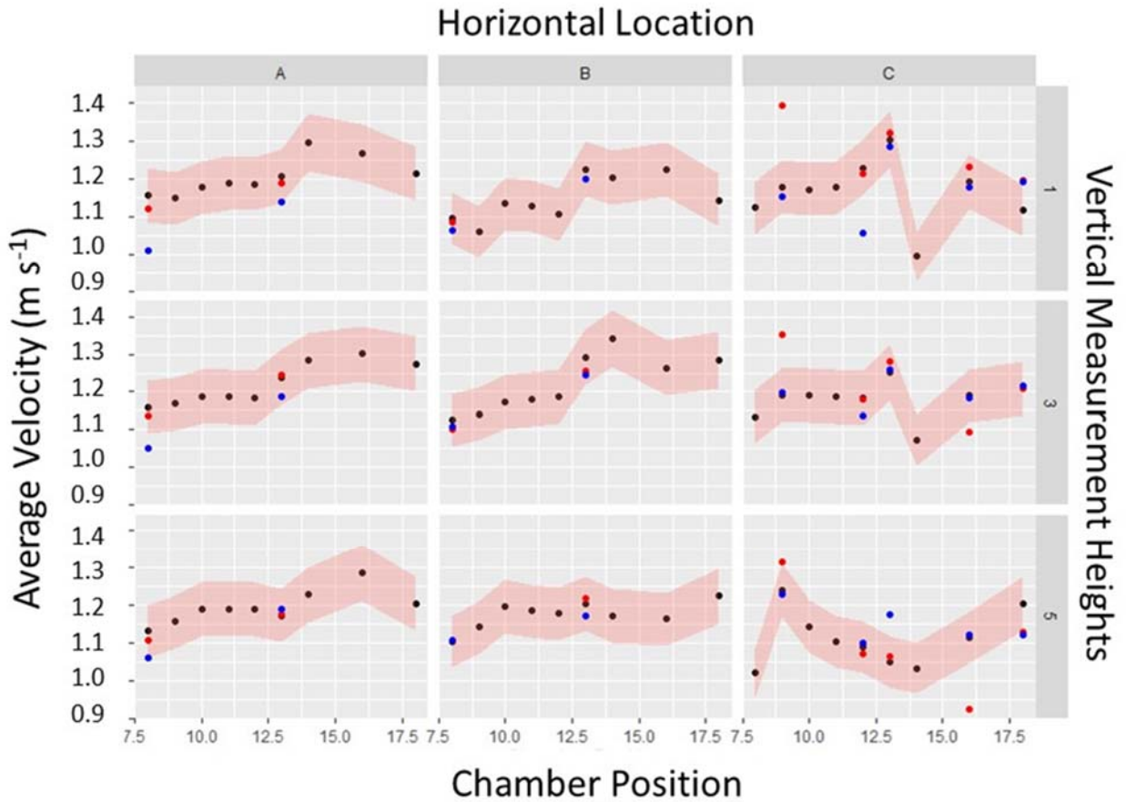
Figure S23. Day-to-Day Variability in Average Velocity at 1.0 \text{ m s}^{-1} , with Flow Straightener
