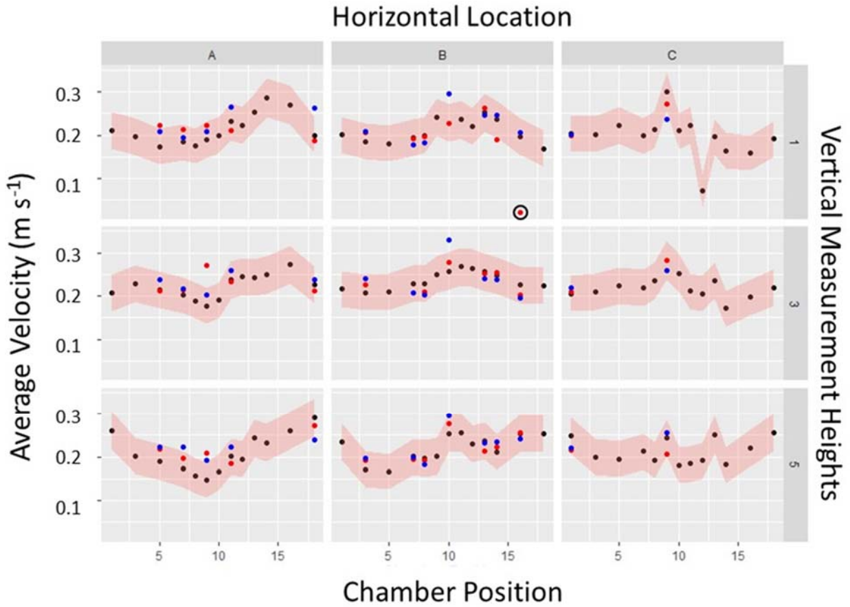
Figure S19. Day-to-Day Variability in Average Velocity at 0.2 \text{ m s}^{-1} , no Flow Straightener
