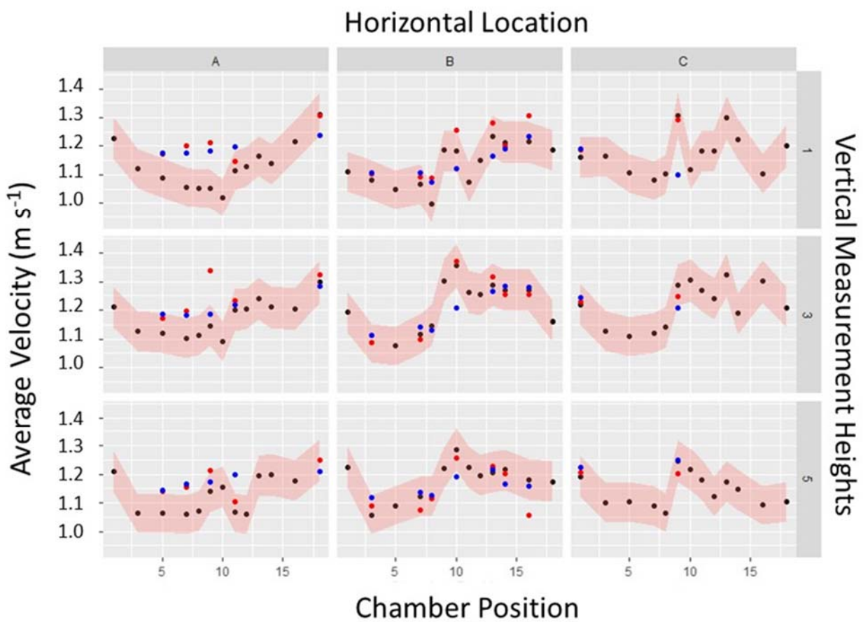
Figure S20. Day-to-Day Variability in Average Velocity at 1.0 \text{ m s}^{-1} , no Flow Straightener
