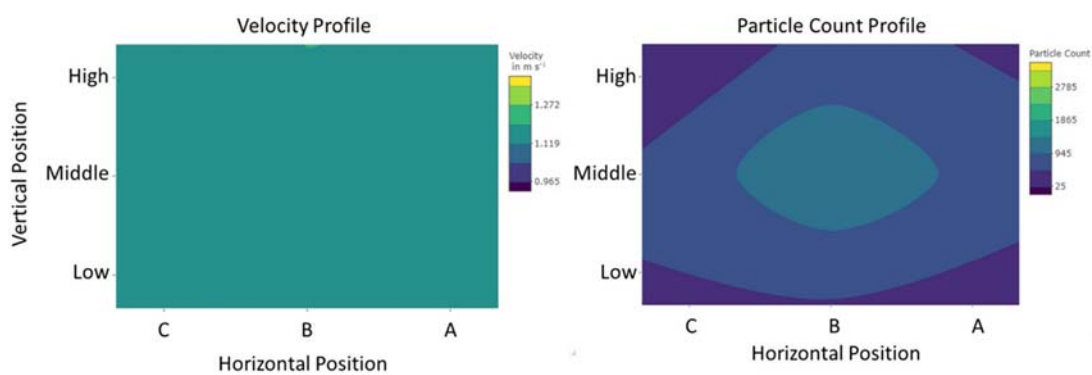
Figure S38. Velocity and Particle Count Profiles in Plane 10 at 1.0 \text{ m s}^{-1}
