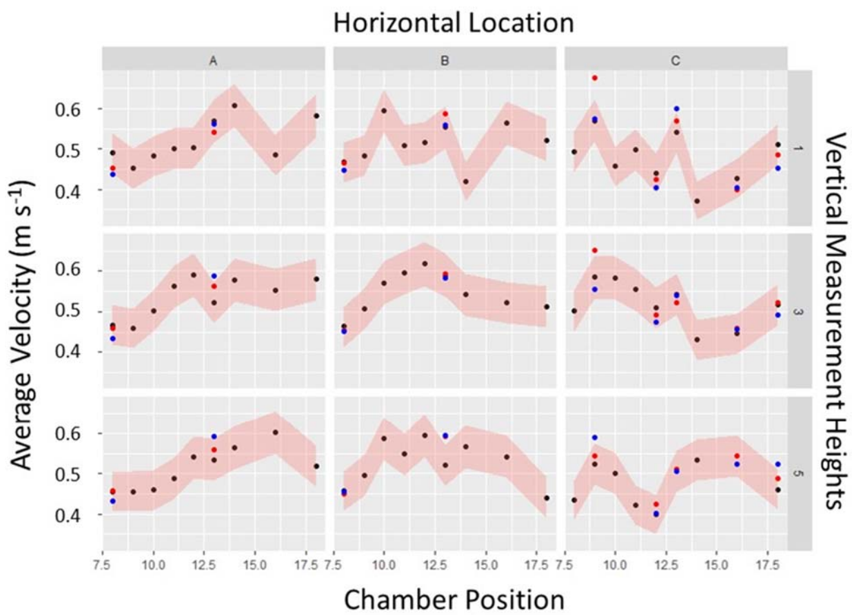
Figure S22. Day-to-Day Variability in Average Velocity at 0.5 \text{ m s}^{-1} , with Flow Straightener
