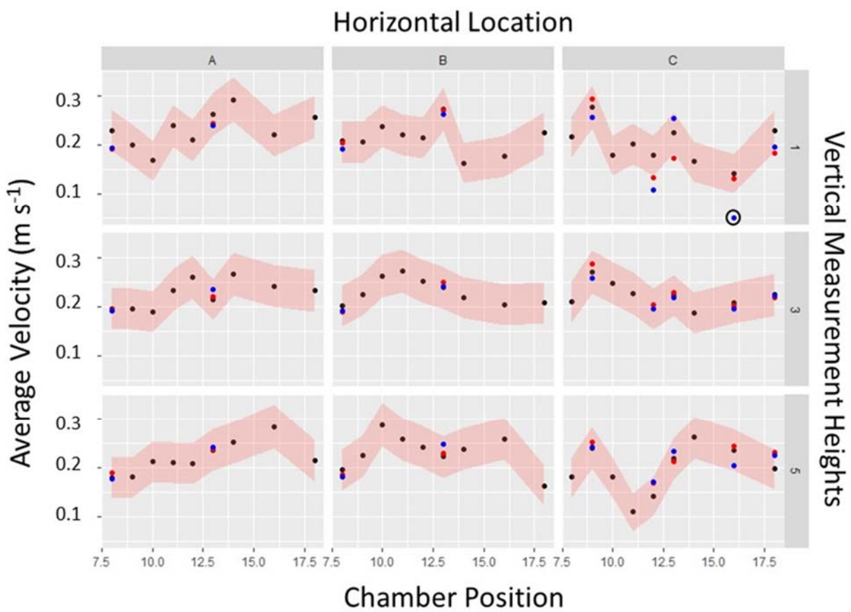
Figure S21. Day-to-Day Variability in Average Velocity at 0.2 \text{ m s}^{-1} , with Flow Straightener
