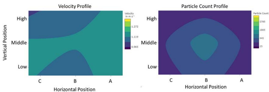
Figure S37. Velocity and Particle Count Profiles in Plane 8 at 1.0 \text{ m s}^{-1}
