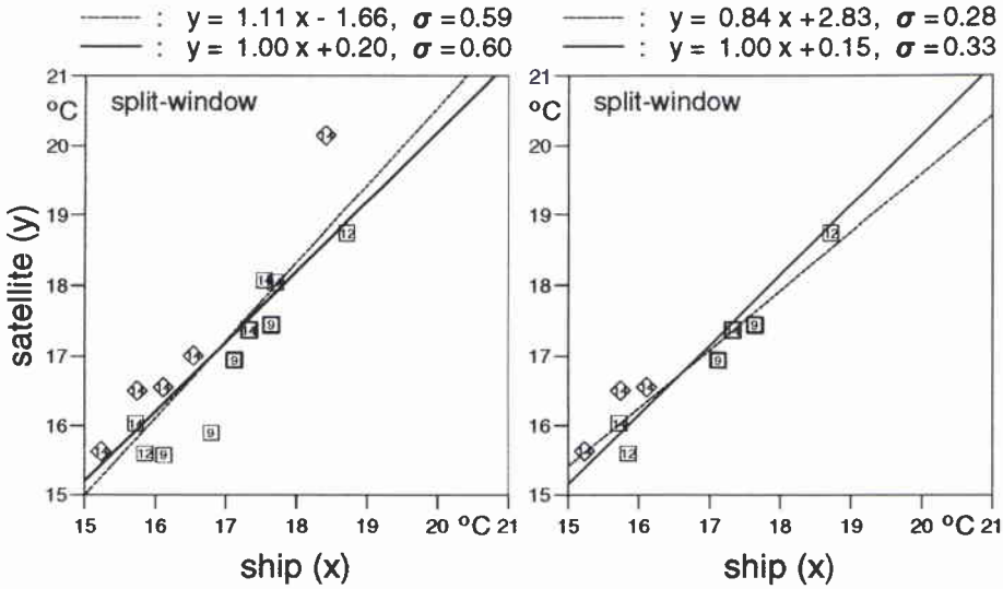
Figure 5: Comparison of coincident satellite- and ship-measured SST during the cruises in the Tyrrhenian Sea (diamonds) and south Adriatic Sea (squares). Bold squares indicate night-time data. Thresholds for the channel-2 albedo are 5% and 3% and for the channel-4 standard deviation 0.3°C and 0.15°C in the left and right panel, respectively.
