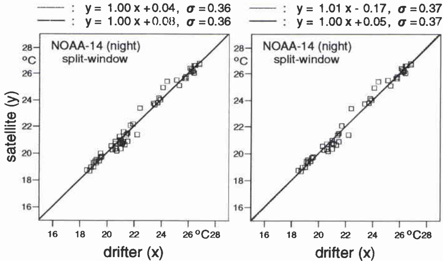
Figure 9: Comparison of coincident satellite- and drifter-measured SST from the south Adriatic and Ionian Sea. The night-time satellite data have been taken from NOAA-14 from May to July 1995. Thresholds for the channel-4 standard deviation are 0.3^{\circ}\text{C} and 0.1^{\circ}\text{C} in the left and right panel, respectively.
