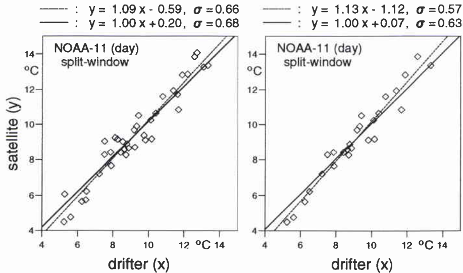
Figure 6: Comparison of coincident satellite- and drifter-measured SST from the Greenland-Iceland-Norwegian Seas. Thresholds for the channel-2 albedo are 5% and 3% and for the channel-4 standard deviation 0.3°C and 0.1°C in the left and right panel, respectively.
