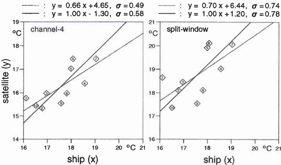
Figure 2: Comparison of satellite- and ship-measured temperatures at the positions indicated in Fig. 1. The numbers refer to the data of Table B1 in Annex B. Left panel: brightness temperatures. Right panel: retrieved SSTs.
