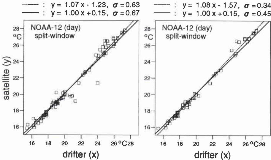
Figure 7: Comparison of coincident satellite- and drifter-measured SST from the south Adriatic and Ionian Sea. The day-time satellite data have been taken from NOAA-12 from May to July 1995. Thresholds for the channel-4 standard deviation are 0.3^{\circ}\text{C} and 0.1^{\circ}\text{C} in the left and right panel, respectively.
