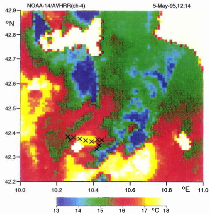
Figure 1: AVHRR (channel-4) brightness temperatures in the Tyrrhenian Sea (south of Elba). The crosses mark positions of NRV Alliance from about 40 min before to 50 min after the satellite overpass.
