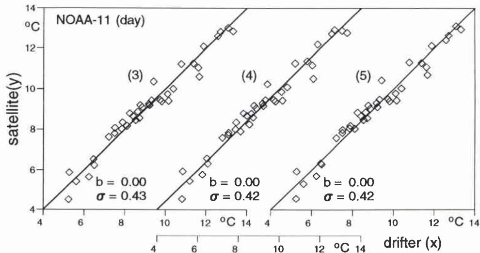
Figure 10: Comparison of coincident satellite- and drifter-measured SST from the Greenland-Iceland-Norwegian Seas. Matched coefficients are used for the algorithms (3)-(5). The thresholds for cloud detection are those of Fig. 6, left panel.
