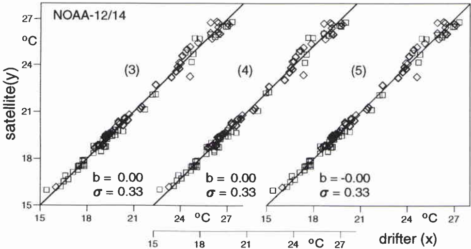
Figure 12: Comparison of coincident satellite- and drifter-measured SST from the Adriatic and Ionian Seas. Satellite measurements from zenith angles less than 40^\circ from both satellites, NOAA-12 (squares) and NOAA-14 (diamonds), are considered. Night-data are indicated by bold frames. Matched coefficients are used for the algorithms (3)-(5). The thresholds for cloud detection are the same as in Fig. 11.
