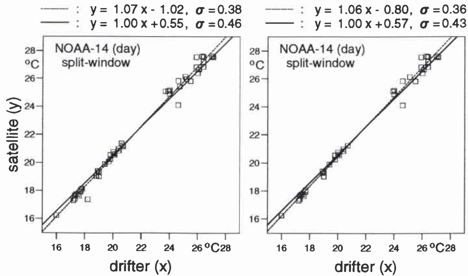
Figure 8: Comparison of coincident satellite- and drifter-measured SST from the south Adriatic and Ionian Sea. The day-time satellite data have been taken from NOAA-14 from May to July 1995. Thresholds for the channel-4 standard deviation are 0.3^{\circ}\text{C} and 0.1^{\circ}\text{C} in the left and right panel, respectively.
