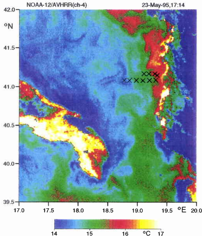
Figure 3: AVHRR (channel-4) brightness temperatures in the south Adriatic Sea. The crosses mark positions of NRV Alliance .
