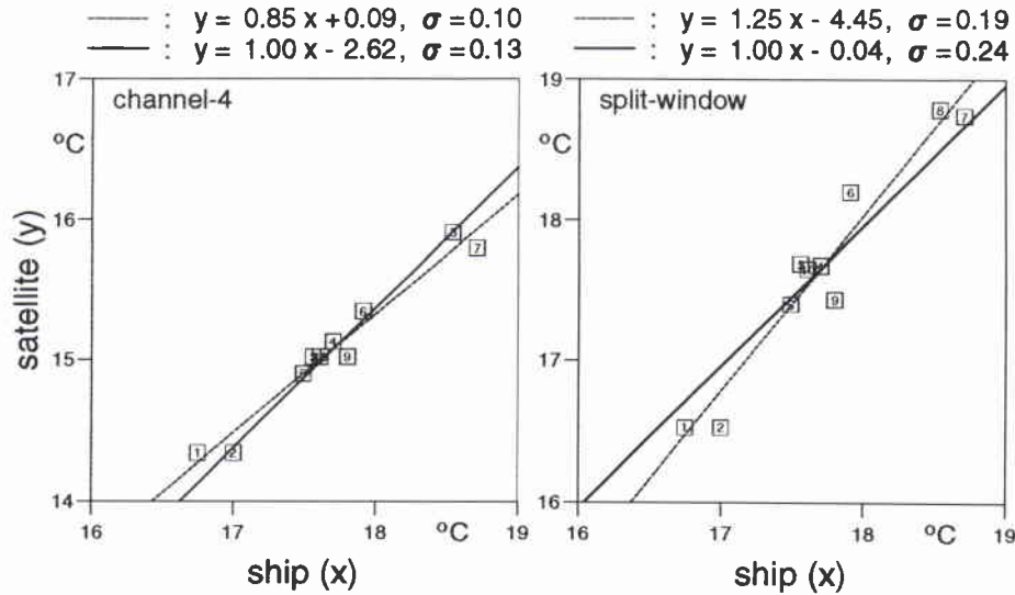
Figure 4: Comparison of satellite- and ship-measured temperatures at the positions indicated in Fig. 3. The numbers refer to the data of Table B2 in Annex B. Left panel: brightness temperatures. Right panel: retrieved SSTs.
