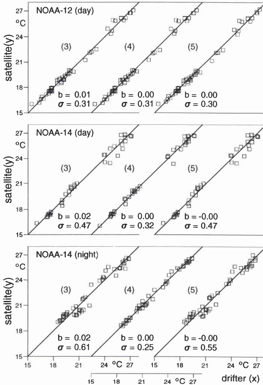
Figure 11: Comparison of coincident satellite- and drifter-measured SST from the Adriatic and Ionian Seas. Matched coefficients are used for the algorithms (3)-(5). The thresholds for cloud detection are those of Figs. 7-9, right panels.
