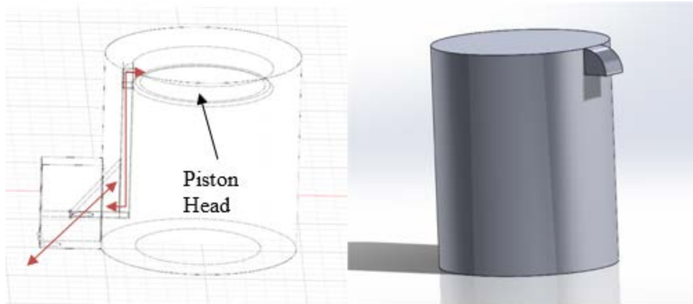
Figure 30. Left: Wireframe Model of Cylinder, Piston at Top. Flow Arrows in Red. Right: Solid Model of Cylinder, with In/Out Port Shown
