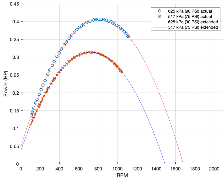
Figure 8. UTAM4-030 Power Curves
