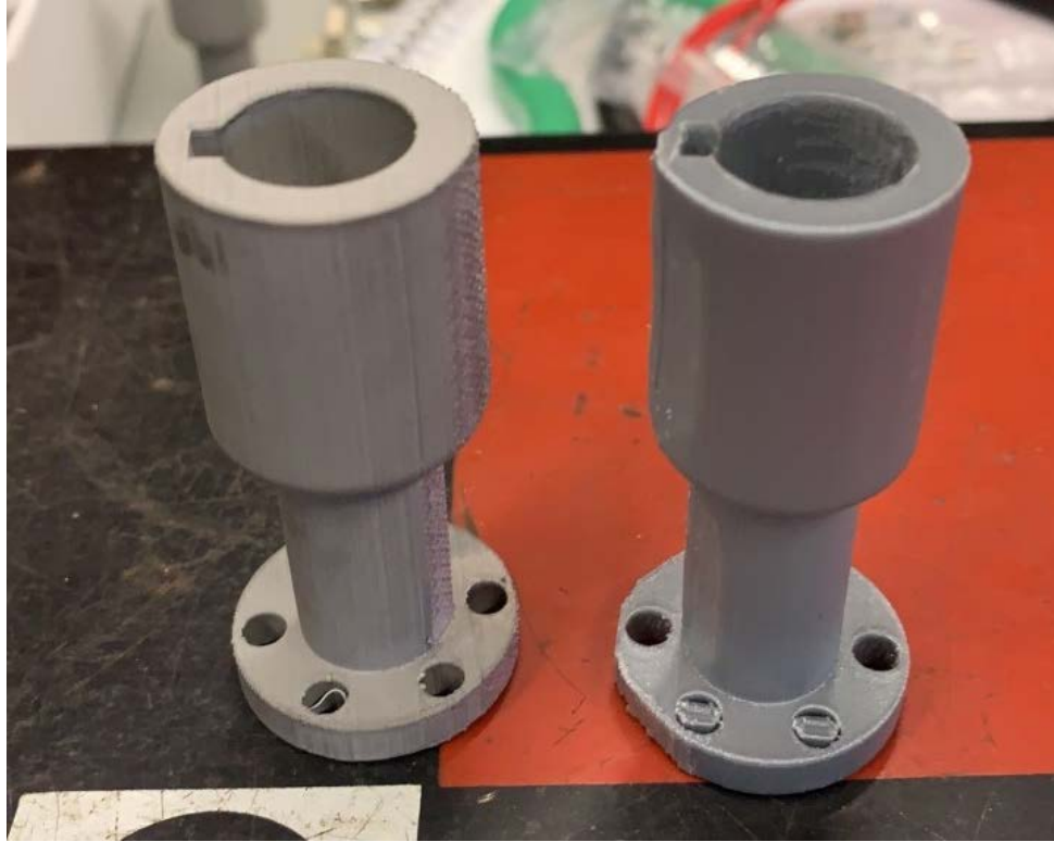
Figure 25. Additive Manufactured Couplings, 17-4 SS (left) and PLA (right)
