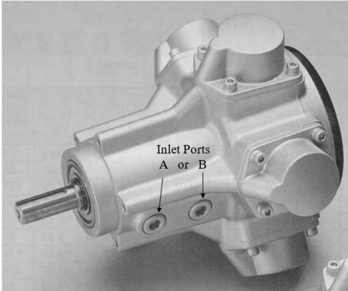
Figure 6. UTAM4-030 Radial Air Motor. Source: [5].
