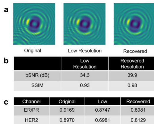
Fig. 5. Resolution enhancement of hologram. (a) Examples of holograms. (b) Increased pSNR and SSIM by deep learning-based resolution enhancement. (c) R^2 for the intensity prediction using the original, low resolution, recovered resolution holograms
