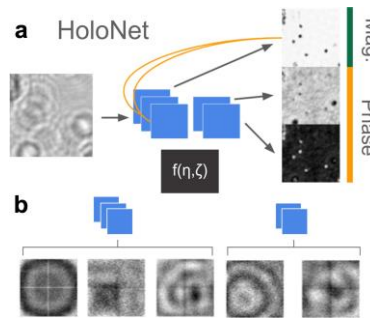
Fig. 2. HoloNet deep learning system. (a) Deep learning pipeline with a sample 192 \times 192 input hologram tile. Tile is processed in realtime by five magnitude and phase recovery filters to output a three-channel reconstruction. (b) Visualization of the learned filters, demonstrating the machine's ability to learn complex optical transformations.
