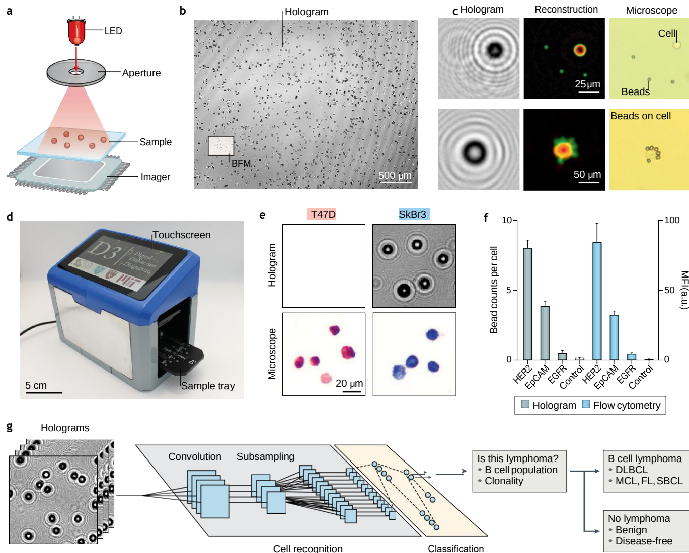
Fig. 3 | LDIH. a | Imaging configuration in lens-free digital in-line holography (LDIH). The system consists of a light-emitting diode (LED), an aperture and an imager, with a sample placed directly above the imager. b | Wide-field-of-view hologram captured by the LDIH imaging system. The individual block dots are cells, and the black box indicates the field of view of a \times 20 bright-field microscope (BFM). c | Raw holograms show undecipherable patterns but the numerical image reconstruction recovers object images. The reference BFM images were taken at \times 20 magnification. d | A portable, stand-alone LDIH device built and used for point-of-care cancer diagnostics. Recorded holograms are transferred to a remote server for image reconstruction. e | Human T47D and SkBr3 breast cancer cells were stained for the oestrogen receptor/progesterone receptor (red) and human epidermal growth factor receptor 2 (HER2; blue) and imaged via LDIH and BFM. Note that the hologram contrast changed according to the staining level. f | Cells were labelled for different biomarkers and analysed by LDIH
