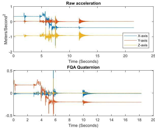
Figure 23. Acceleration data and corresponding quaternion
