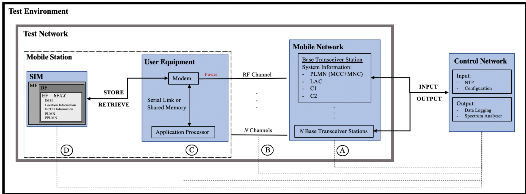
Figure 11. Experiment Environment
