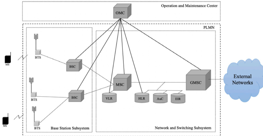
Figure 4. GSM Architecture. Adapted from [18].
