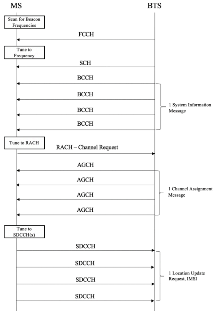
Figure 9. Simplified Process for Initializing Location Update
