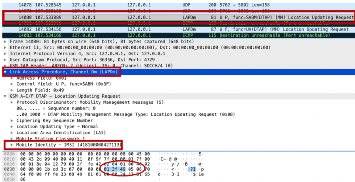
Figure 15. Wireshark Packet Capture Location Update Part I
