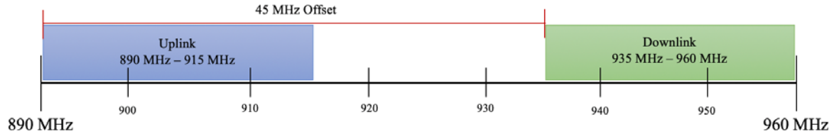
Figure 5. Uplink and Downlink Spectrums for Band 900
