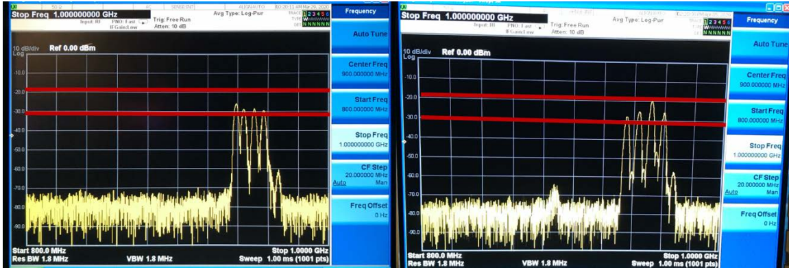
Figure 31. Matched vs. Unmatched Downlink Power Peaks, 900 MHz Band
