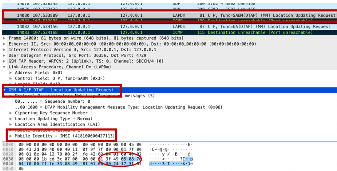
Figure 16. Wireshark Packet Capture Location Update Part II
