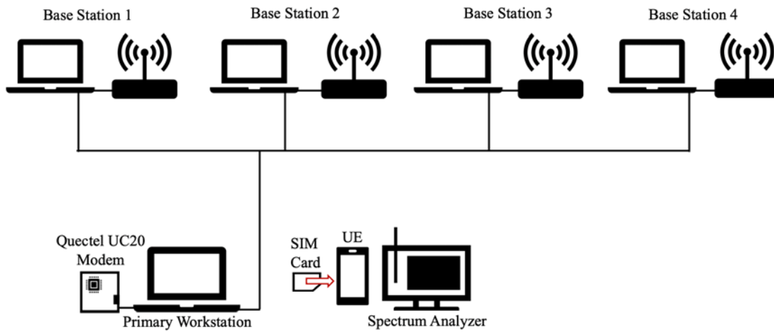
Figure 18. Workspace Diagram
