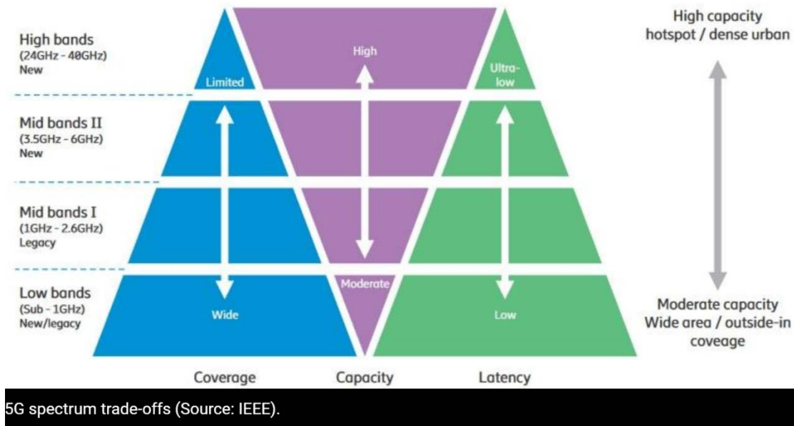
Figure 3. 5G Spectrum Trade-Offs 188
