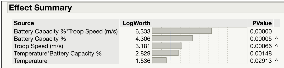
Figure 45. Total AN/PSN – 13(B) DAGR Batteries Effects Summary Shows Factor Significance
