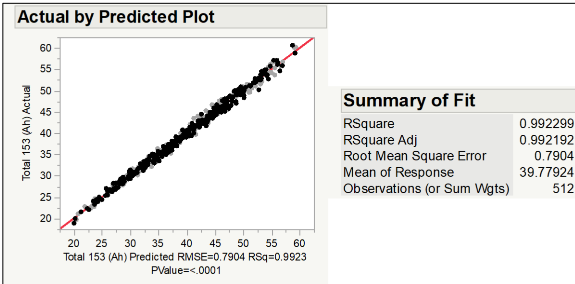
Figure 24. Total AN/PRC-153 Amp-Hours Actual by Prediction Plot and Summary of Fit
