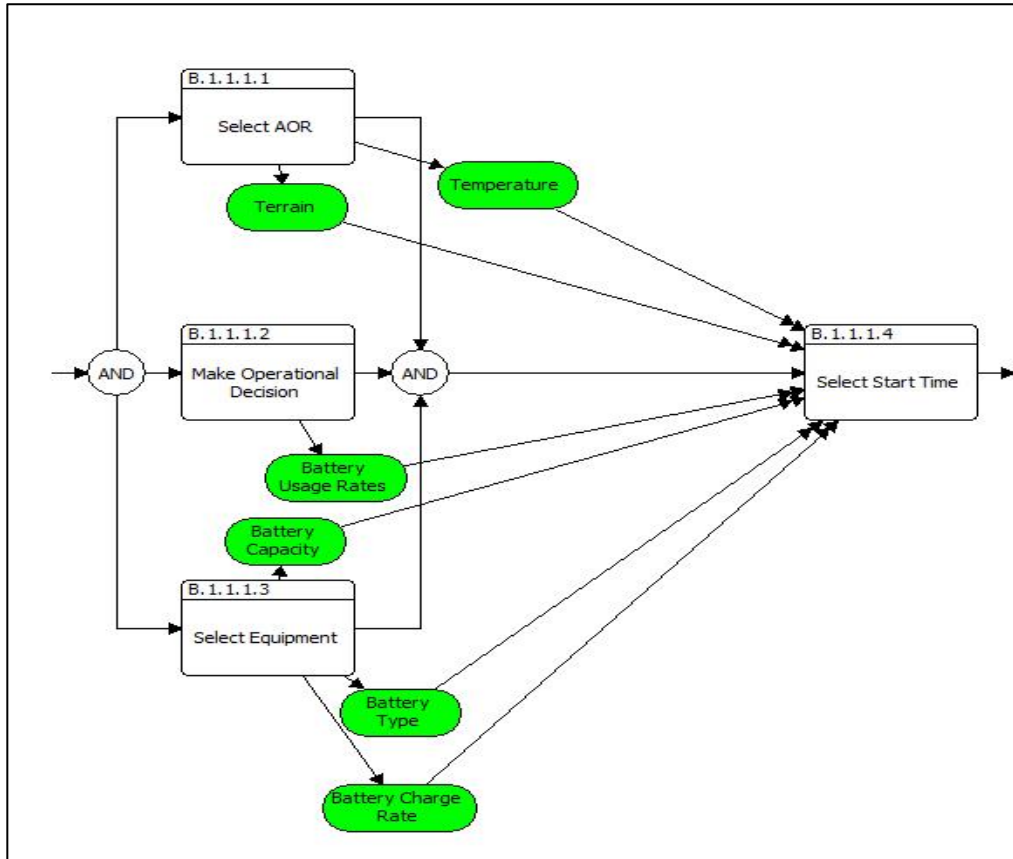
Figure 11. Plan Functional Flow Block Decomposition
