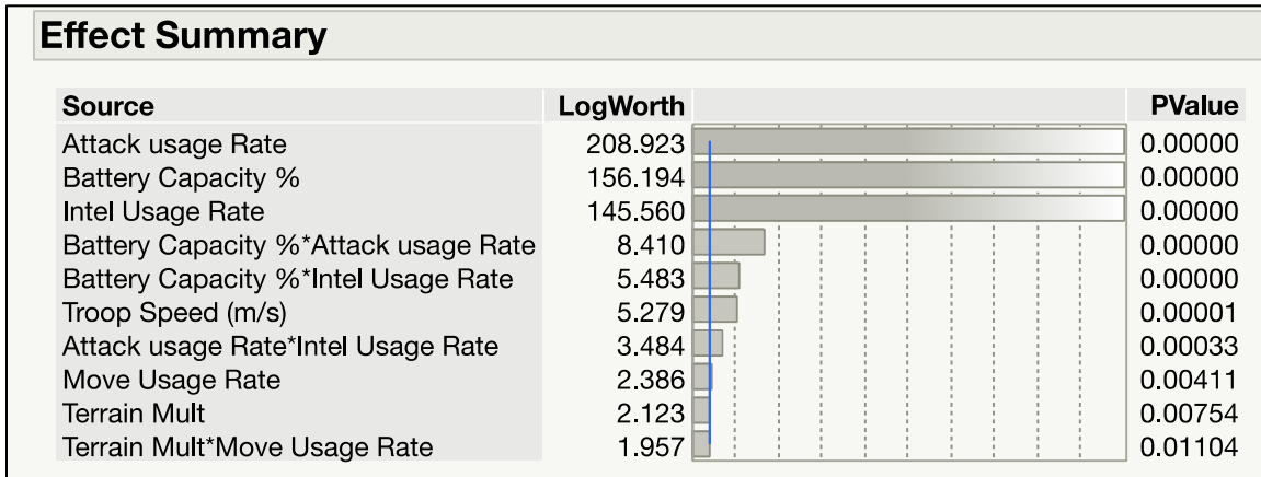
Figure 42. Total AN/PRC-148 Batteries Effects Summary Shows Factor Significance
