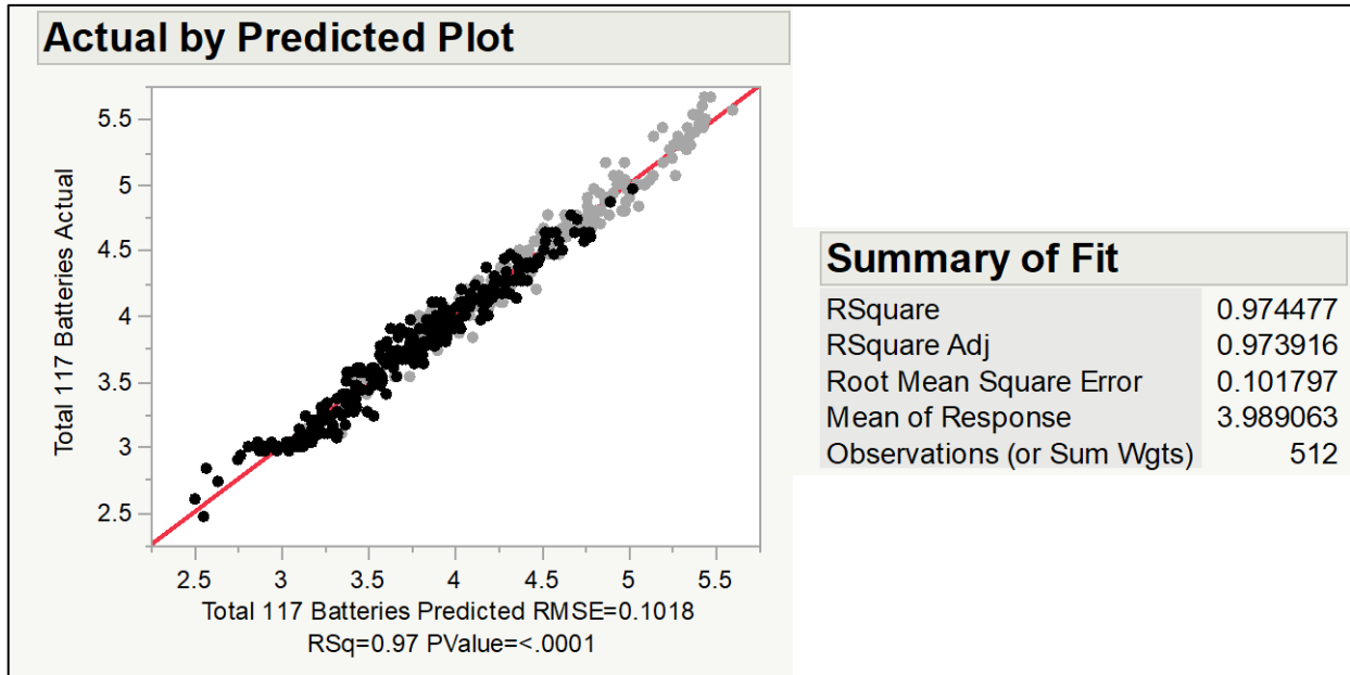
Figure 35. Total AN/PRC-117 Batteries Actual by Prediction Plot and Summary of Fit
