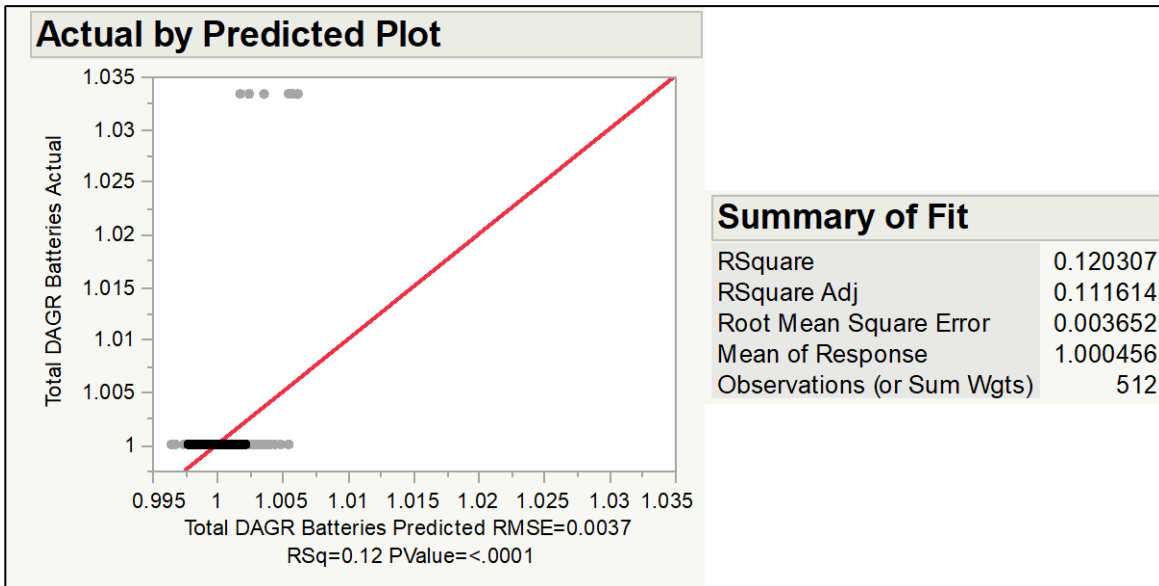
Figure 44. Total AN/PSN – 13(B) DAGR Batteries Actual by Prediction Plot and Summary of Fit
