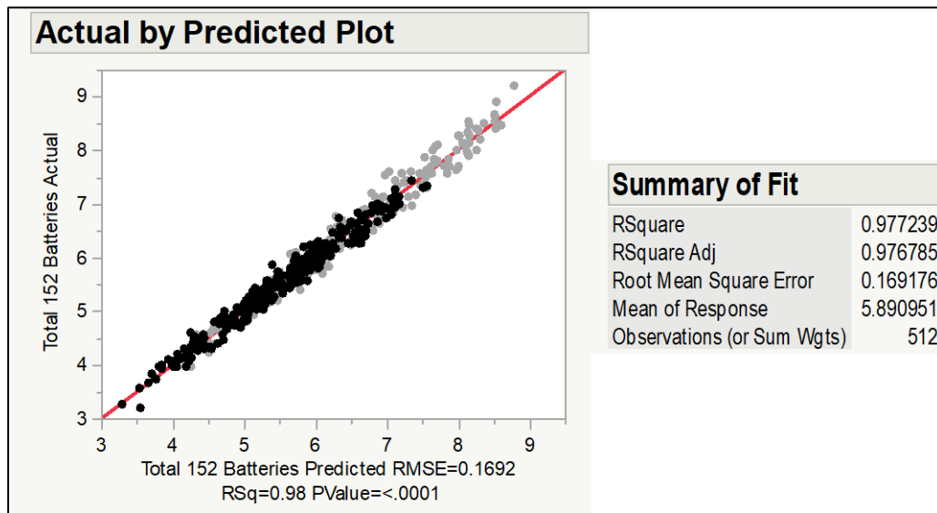
Figure 38. Total AN/PRC-152 Batteries Actual by Prediction Plot and Summary of Fit
