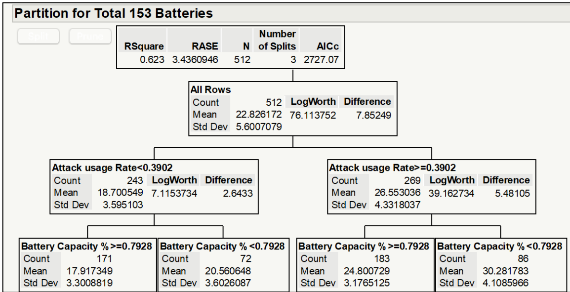
Figure 21. Partition of Total AN/PRC-153 Batteries Using the Attack Usage Rate and Battery Capacity
