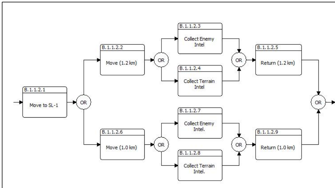
Figure 12. Observe Functional Flow Block Decomposition
