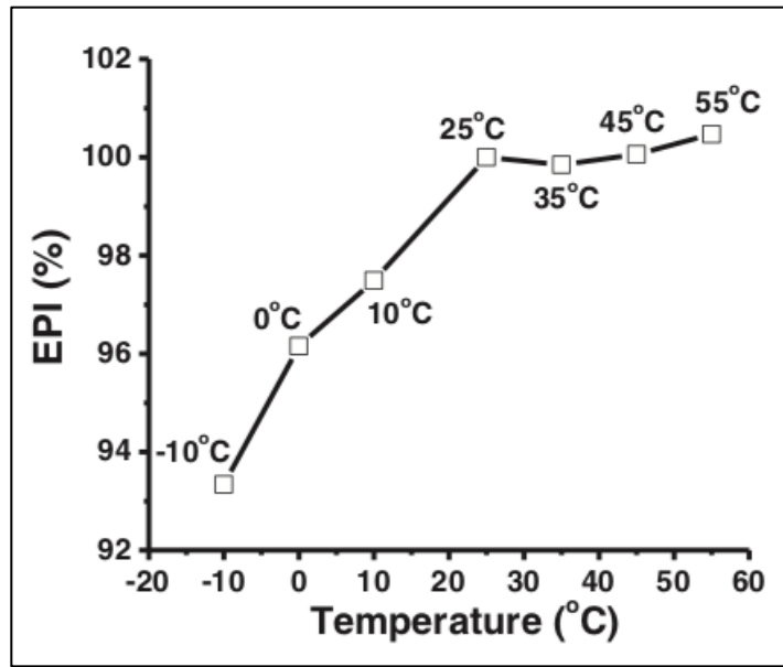
Figure 2. Energy-Power Index (EPI) Profile of Lithium-Ion Cells. Source: Kumar et al. (2018).
