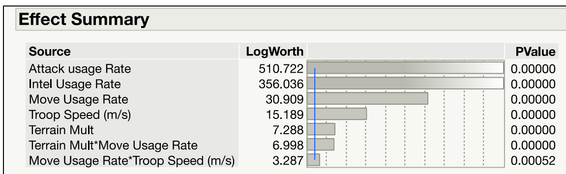
Figure 25. Total AN/PRC-153 Amp-Hours Effects Summary Shows Factor Significance
