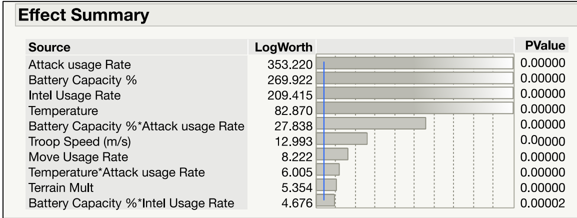
Figure 39. Total AN/PRC-152 Batteries Effects Summary Shows Factor Significance
