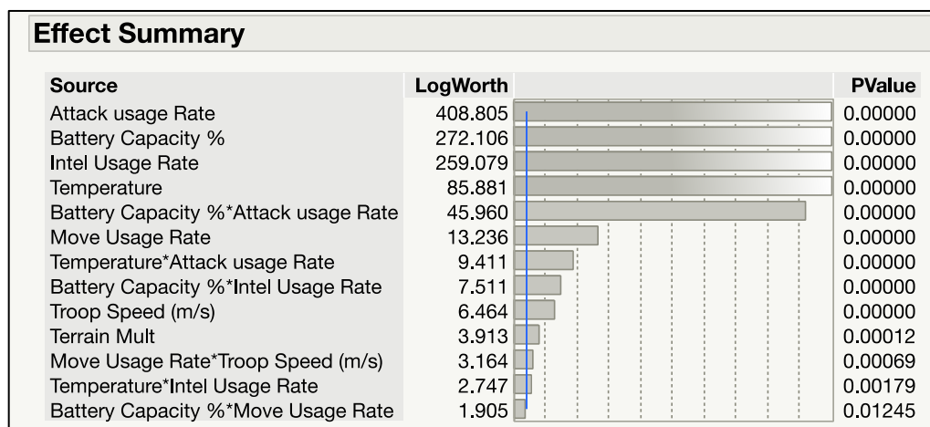
Figure 19. Total AN/PRC-153 Batteries Effects Summary Shows Factor Significance
