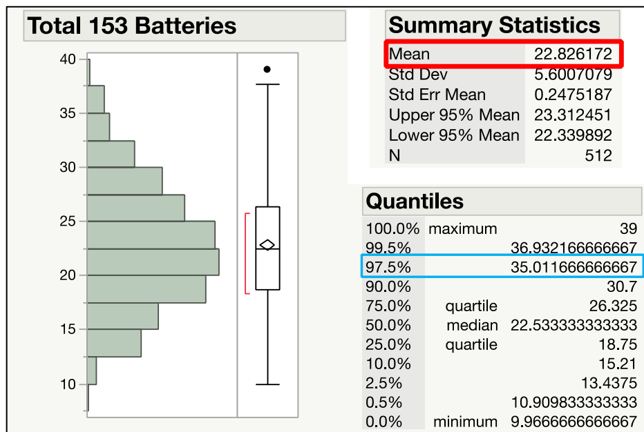
Figure 16. Total AN/PRC-153 Batteries Histogram and Data Summary
