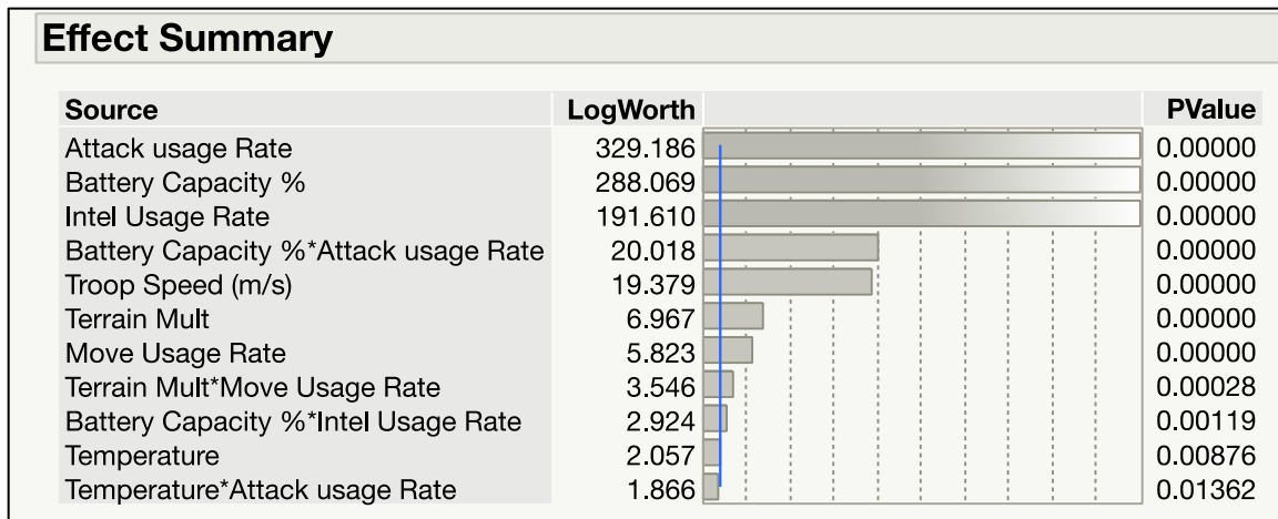
Figure 36. Total AN/PRC-117 Batteries Effects Summary Shows Factor Significance
