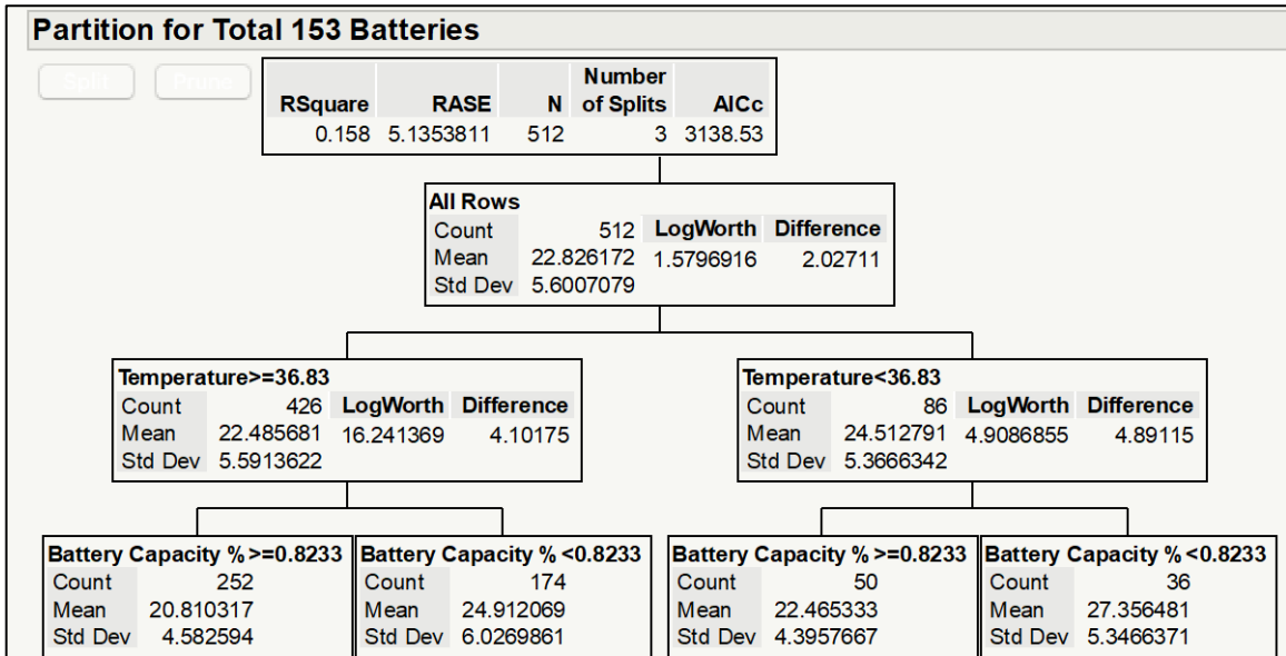
Figure 22. Partition of Total AN/PRC-153 Batteries Using Battery Capacity
