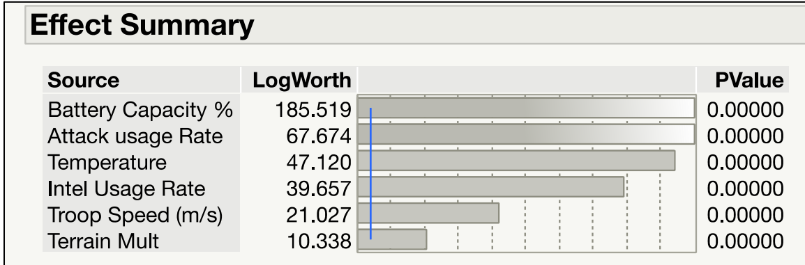
Figure 33. Total AN/PRC-150 Batteries Effects Summary Shows Factor Significance
