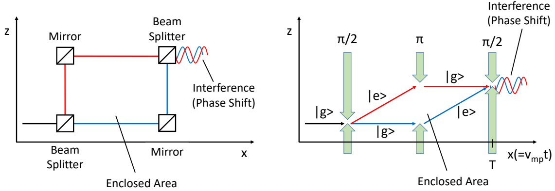
Figure 4.2: Mach-Zehnder interferometer using light waves (left). Mach-Zehnder interferometer using matter waves with light pulses as analogs for beam splitters and mirrors (right). Note that this simultaneously represents state-space and top-down views.
