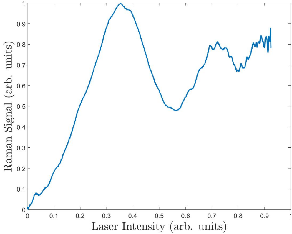
Figure 5.11: Rabi oscillations.
