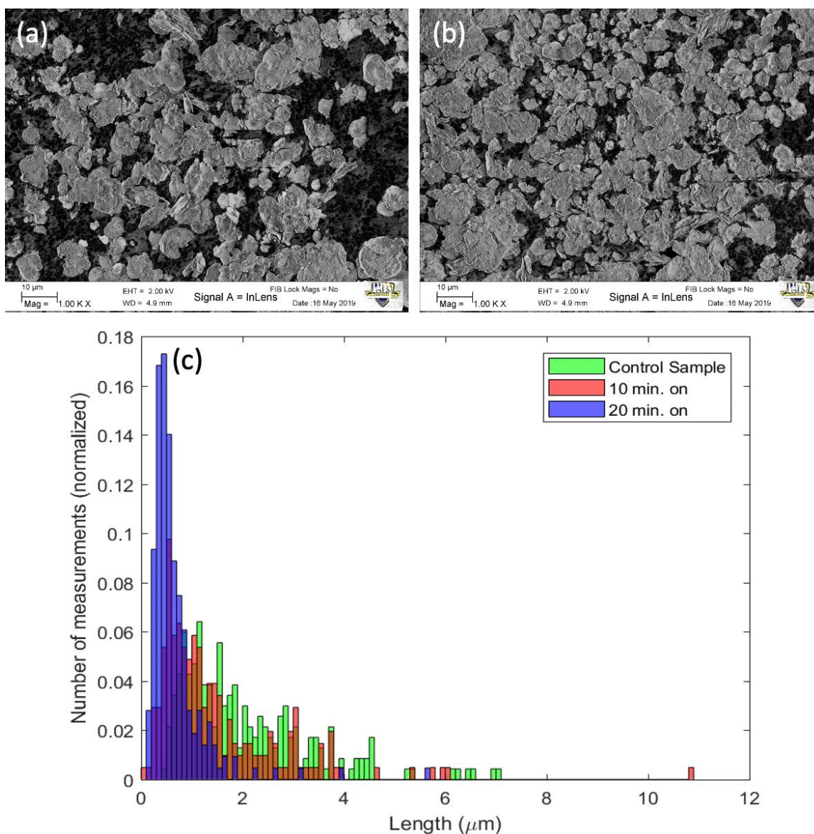
Figure 12. BNNP Following (a) 10 Minutes and (b) 20 Minutes of Cryomilling and (c) a Histogram of the Longest Dimension of BNNP in Each Group
