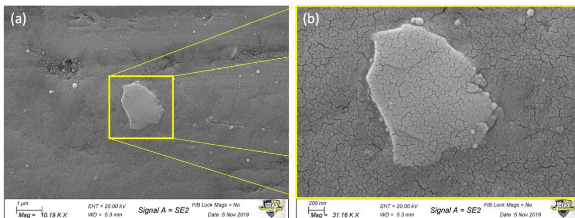
Figure 21. BNNP Observed in Coating 3 at (a) Intermediate Magnification and (b) High Magnification
