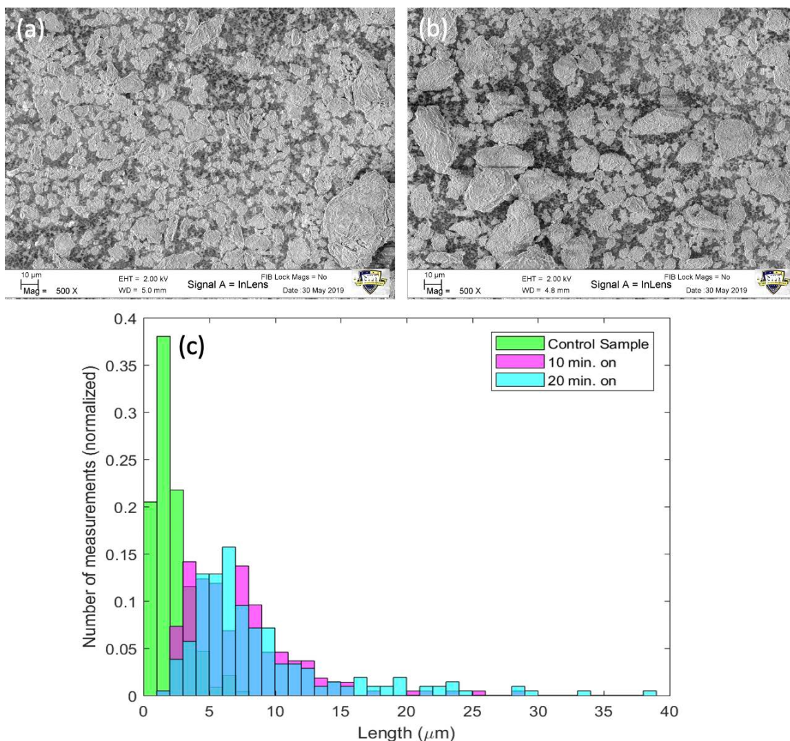
Figure 13. BNNP Following (a) 10 Minutes and (b) 20 Minutes of HEBM and (c) a Histogram of the Longest Dimension of BNNP in Each Group
