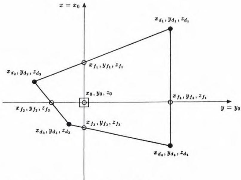
Fig. 4. UNIRAS interpolation method grid scheme.
