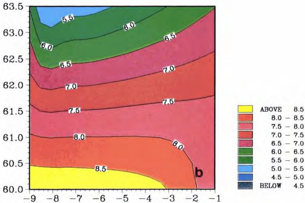
Fig. 7. (a) Temperature measurements at 100 m depth, from the GIN '86 data. (b) Temperature field obtained from the Levitus climatology at 100 m depth.
