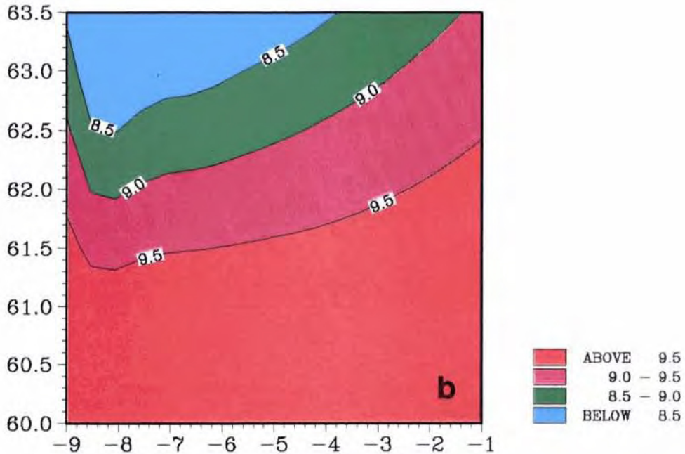
Fig. 5. (a) Temperature measurements at 10 m depth from the GIN '86 data. (b) Temperature field obtained from the Levitus climatology at 10 m depth.
