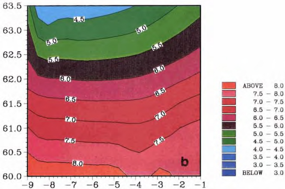
Fig. 9. (a) Temperature measurements at 200 m depth, from the GIN '86 data. (b) Temperature field obtained from the Levitus climatology at 200 m depth.
