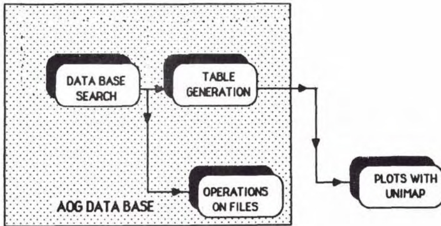
Fig. 2b. Database plan diagram.
