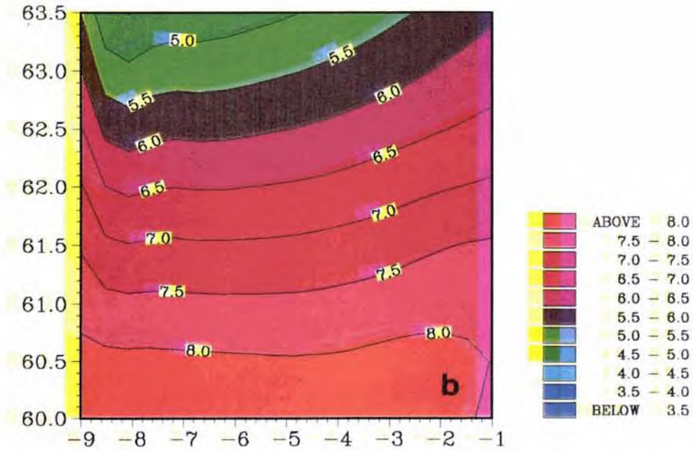
Fig. 8. (a) Temperature measurements at 150 m depth, from the GIN '86 data. (b) Temperature field obtained from the Levitus climatology at 150 m depth.
