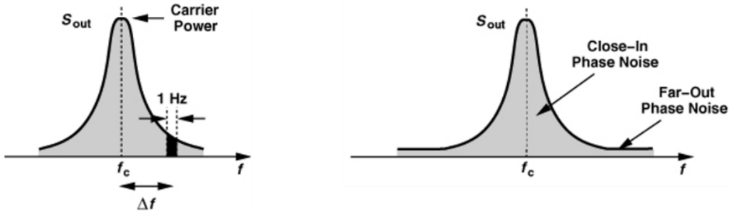
Figure 33. Phase noise measurement of 1 Hz band located \Delta f from signal of interest carrier frequency. Source: [19].
