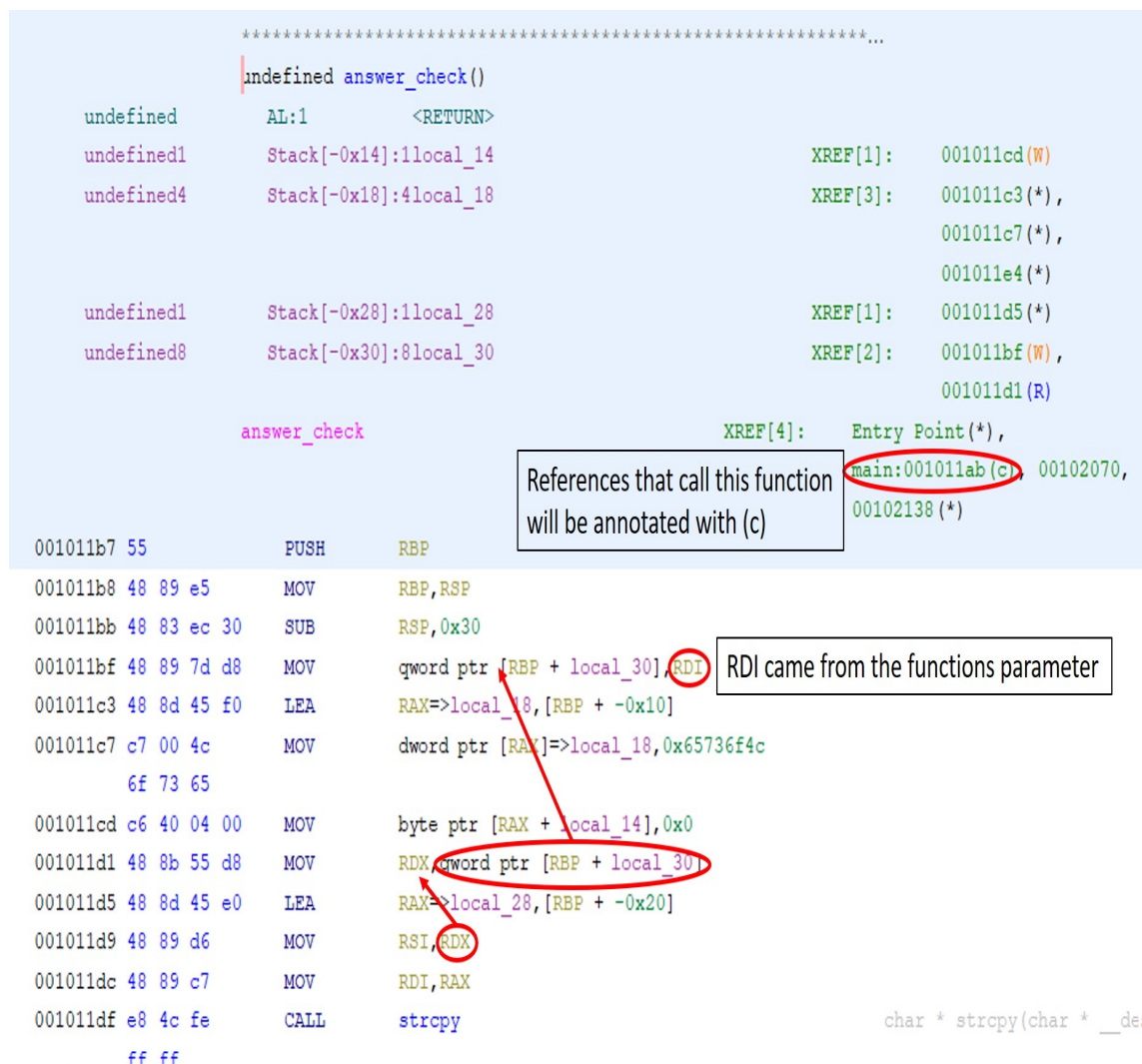
Figure 4.2. Ghidra disassembly of a source being passed to a sink
