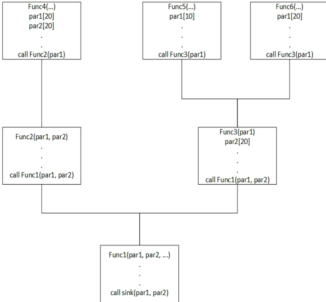
Figure 3.1. Source tree with the sink as the root
