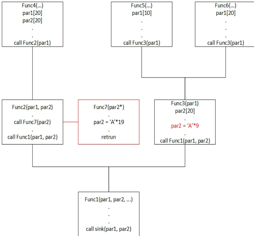
Figure 5.5. Source tree highlighting how the sources are filled
