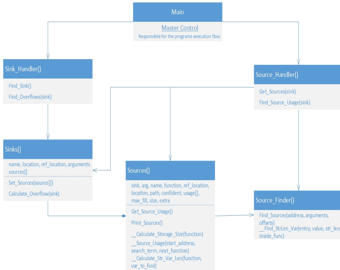
Figure 4.1. Class diagram for the buffer overflow detection program
