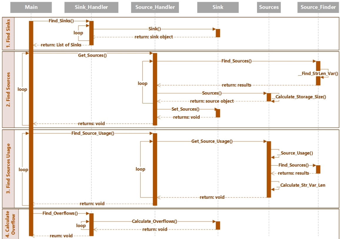
Figure 4.3. Sequence diagrams for buffer overflow detection
