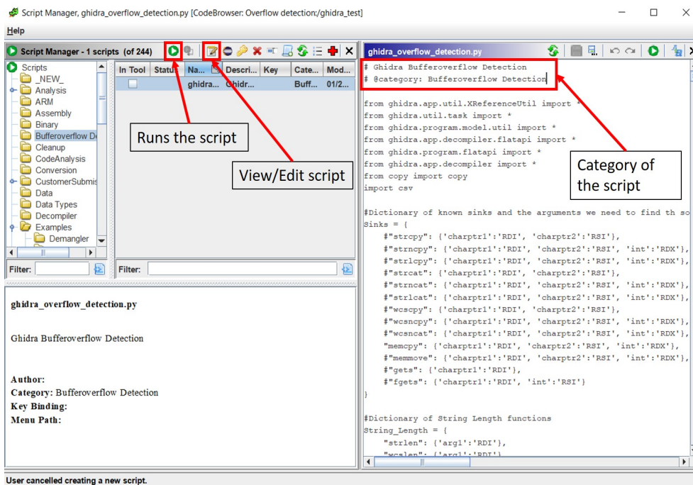
Figure A.3. Ghidra script manager for view, editing, and running scripts
