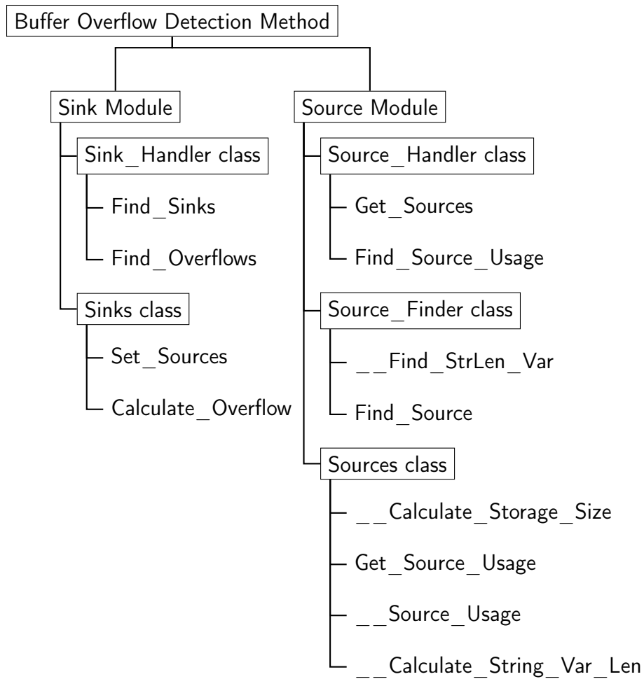
Figure 5.1. Organization of modules, classes, and functions
