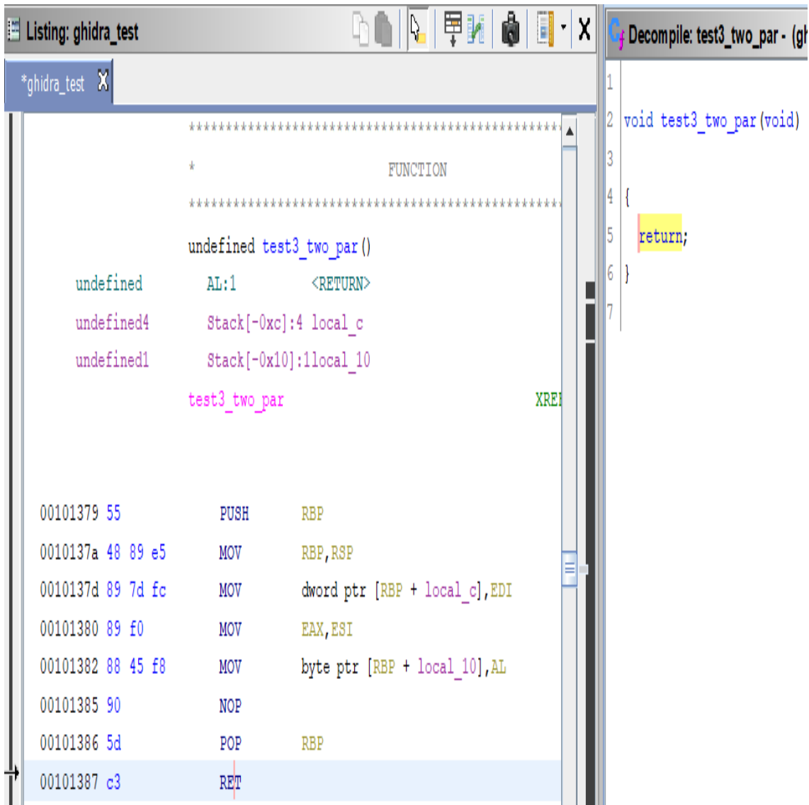
Figure E.3. Test 3: Function with two parameters
