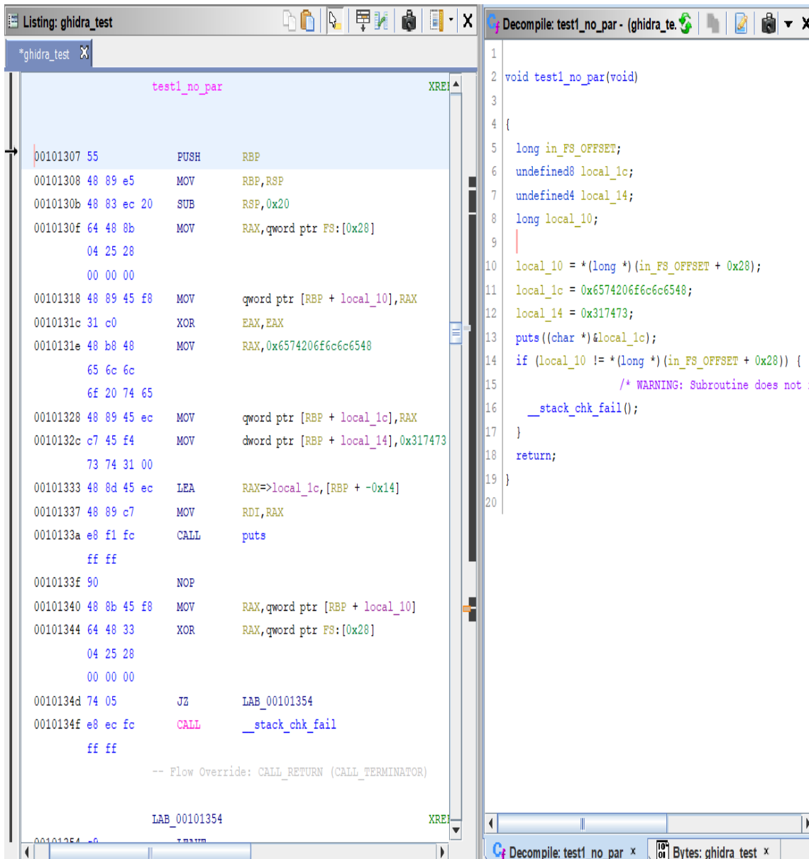
Figure E.1. Test 1: Function with no parameters
