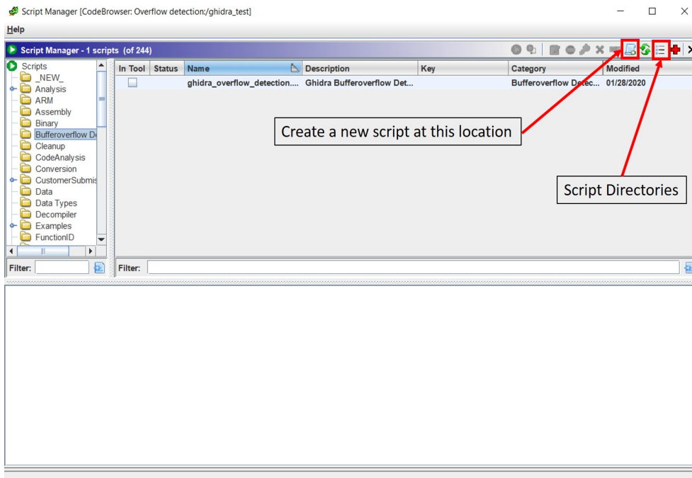
Figure A.2. Ghidra script manager window
