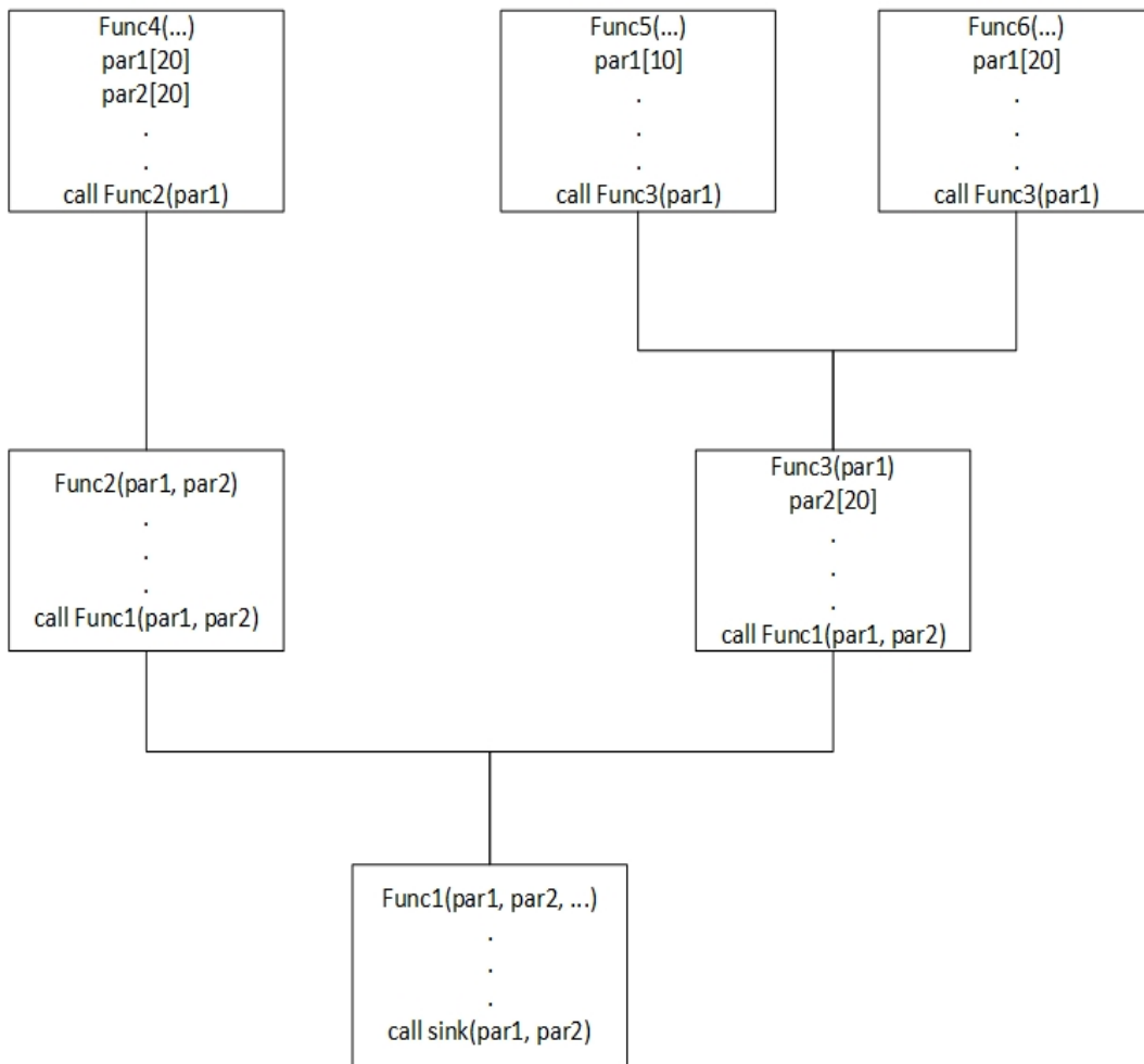
Figure 5.2. Source tree with the sink as the root (repeat from chapter 3)
