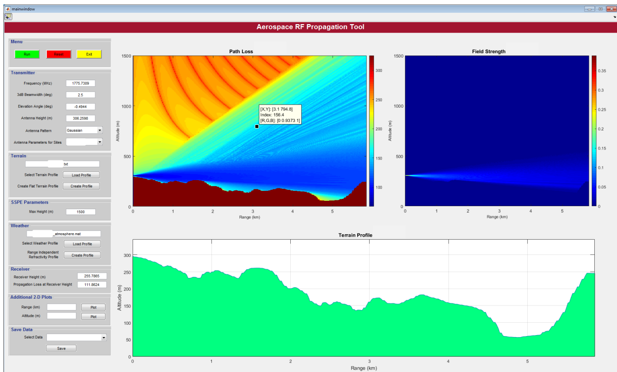
Figure 6. Path loss calculation completed.
