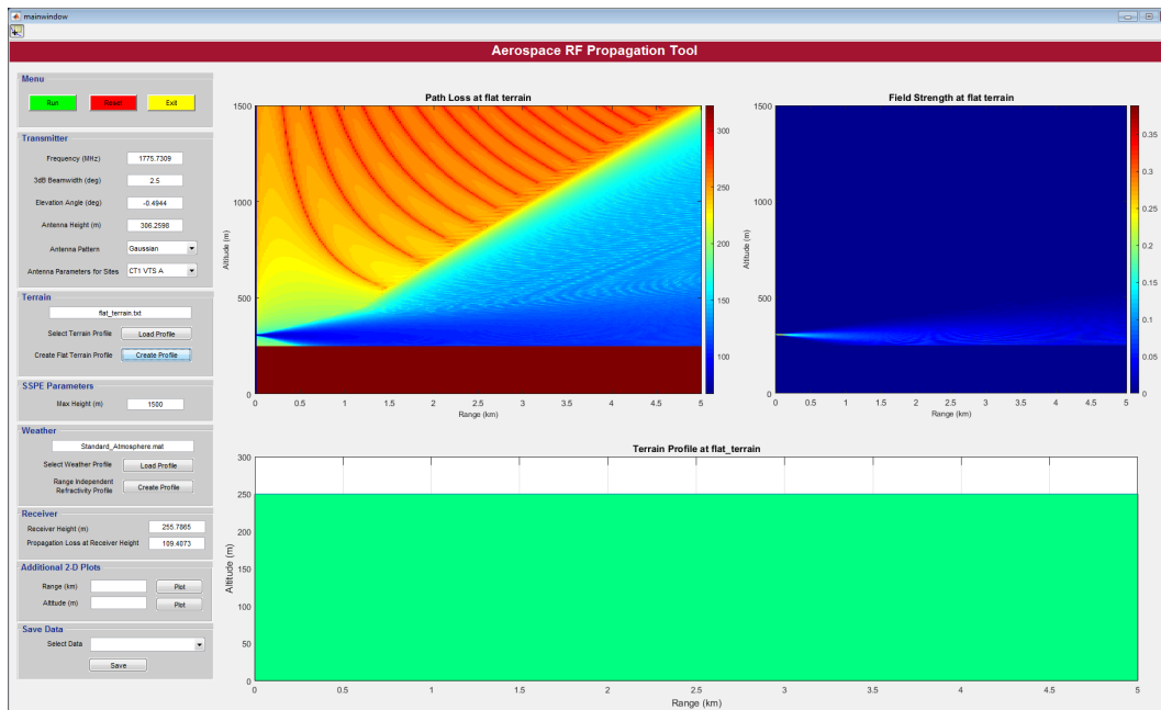
Figure 16. Using flat terrain and range independent weather profile.
