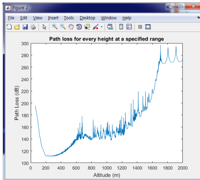
Figure 10. Path loss for every height at a specified range.
