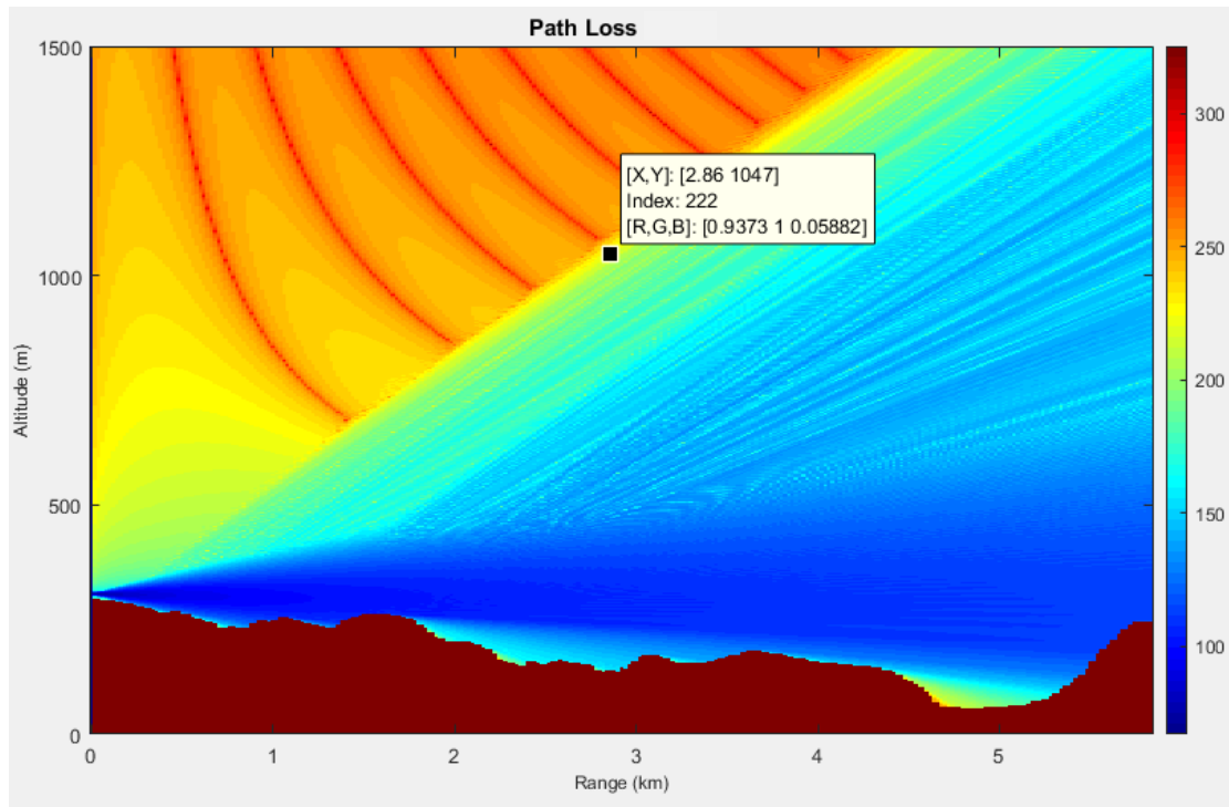
Figure 7. Path loss plot.
