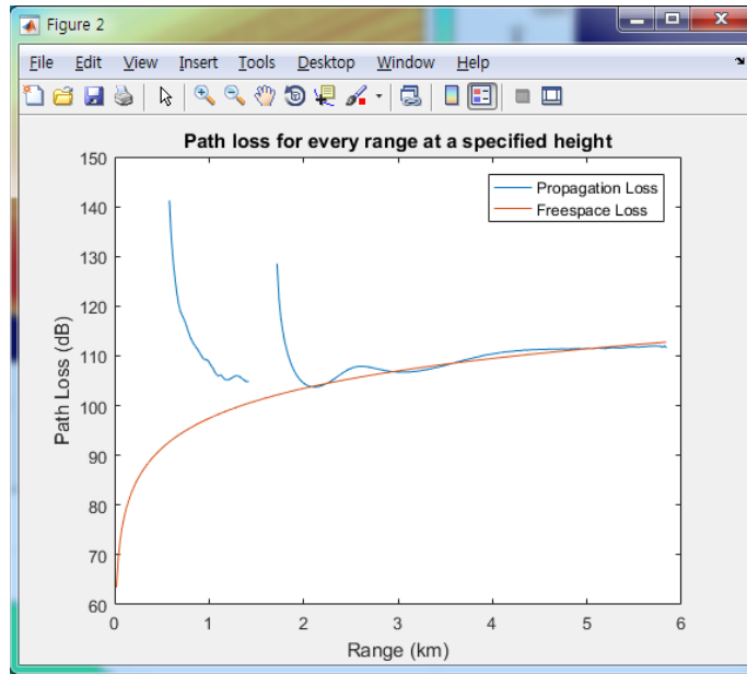
Figure 9. Path loss for every range at a specified height.
