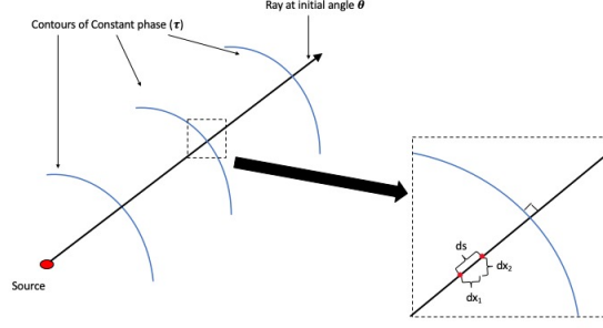
Figure 2-3: The ray leaving the source at a specified angle travels perpendicular to the wave front. Here, we see that infinitesimal changes in the Cartesian plane ( x_1, x_2 ) corresponds to infinitesimal steps along the ray or arc-length.
