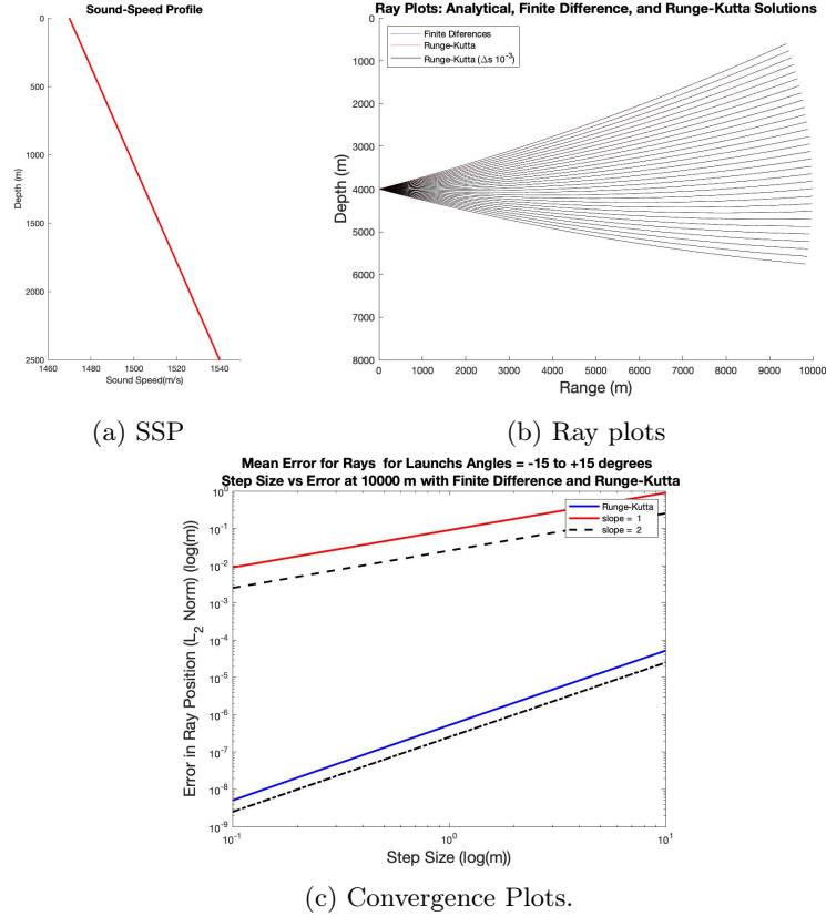
Figure 3-7: Using a less steep SSP gradient and extending the rays to 10^4 m: a) SSP (b) Initial ray trajectories are evenly spaced between 15^\circ above and below the horizontal. Runge-Kutta and forward Euler Rays are computed using a step-size of 1 m with the reference ray trace using Runge-Kutta and a step-size of 10^{-3} m. (c) Convergence rates are identical to those observed when comparing to the analytical solution.
