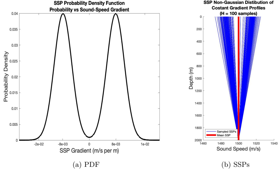
Figure 4-1: (a) We combine two separate normal distributions with means at \pm 8\text{e-}3 respectively into a non-Gaussian distribution (b) From this distribution, we can sample SSPs of different sound-Speed Gradients
