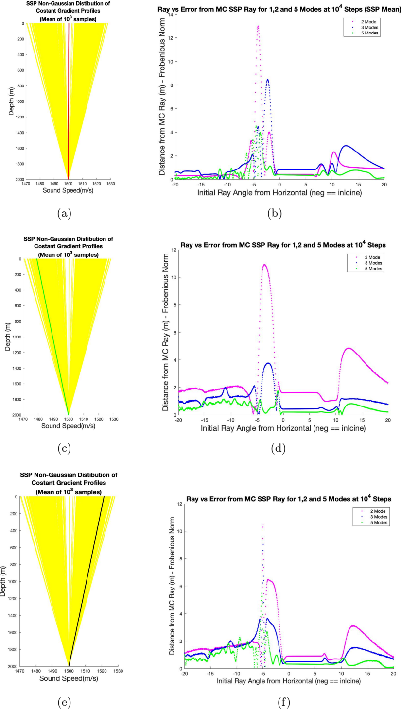
Figure 4-6: Panels (a), (c), and (e) Computed ray traces for highlight SSPs. Panels (b), (d), and (f) show the associated error as compared to the Monte Carlo solution for a particular realization when using 2, 3, or 5 modes. Note errors in a realization and the trend as we increase the number of modes. For a particular realization the error approaches the deterministic solution. Ray traces computed 1001 rays at evenly spaced angles between \pm 20^\circ , 1st-order Forward Difference with a 1m step-size.
