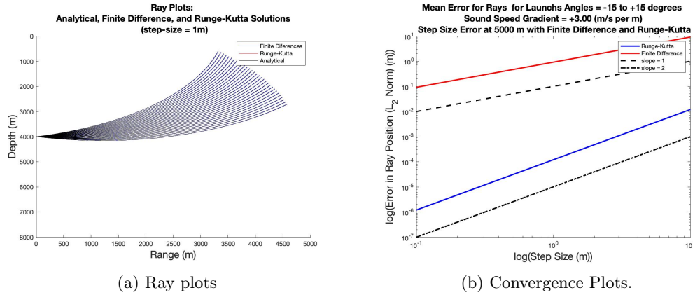
Figure 3-6: This test case is is an idealized ocean scenario. The sound speed profile has a constant gradient of 3 m/s per m resulting in unrealistic sound-speeds closer to the surface and the bottom. a) Ray paths evenly spaced between 15° above and below the horizontal and computed using a step-size of 1 m. At this scale, the difference in the ray paths are indistinguishable. (b) We observe the expected convergence rate as step size decreases confirming the first-order convergence of forward Euler and second-order convergence of Runge-Kutta.
