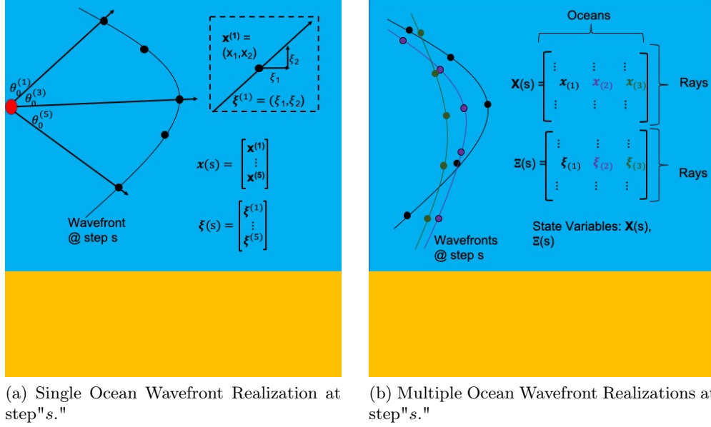
Figure 3-1: (a) Depiction of how for a single ocean, the wavefront at a given step along all of the rays "s" can be represented by 2 vectors, each of length 2 \times (\#rays) . (b) Depiction at the same step along the rays "s," for multiple ocean realizations, \mathbf{X} and \Xi represent a field of wavefronts for which we can obtain a reduced order representation.
