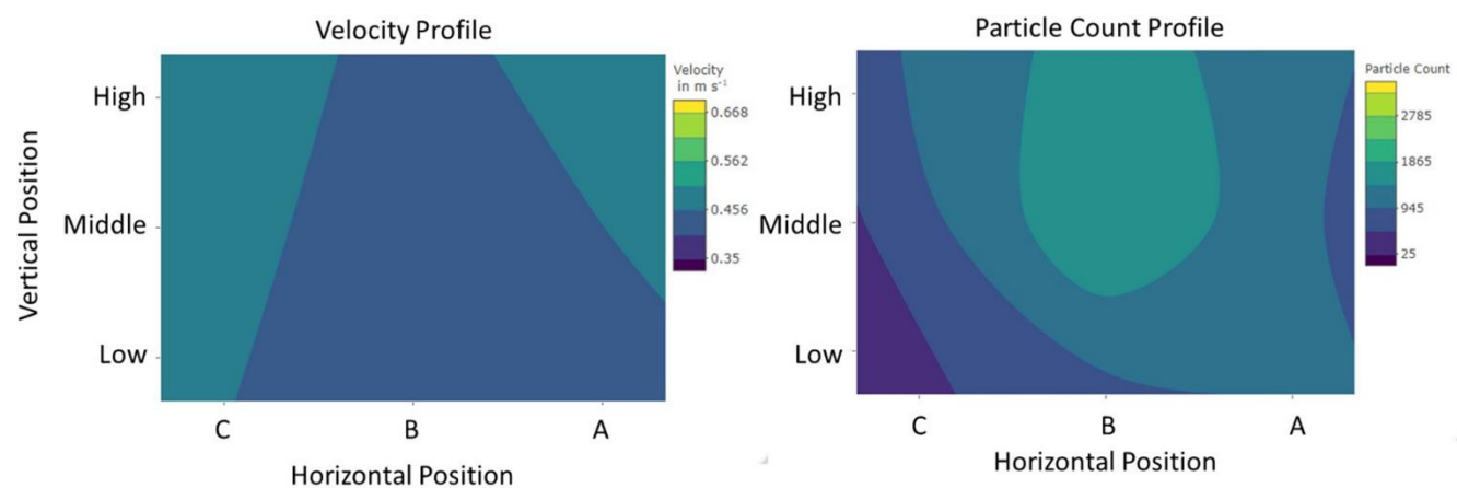
Figure 48. Velocity and Particle Count Profiles in Plane 5 at 0.5 \text{ m s}^{-1}
