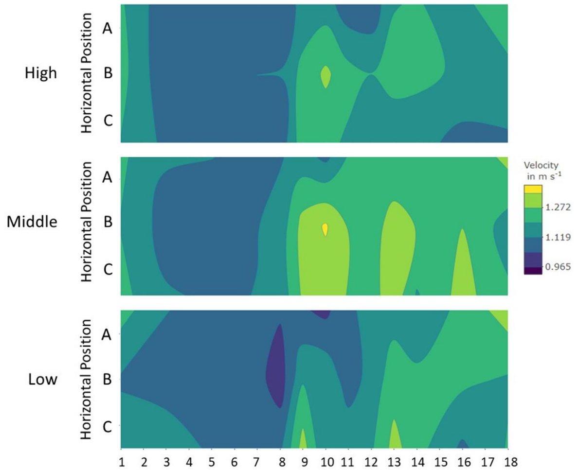
Figure S52. Vertical Velocity Profile of the Chamber at 1.0 \text{ m s}^{-1} (60 Hz), no Flow Straightener
