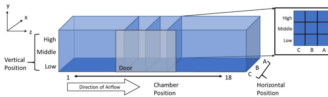
Figure 40. Chamber Measurement Locations
