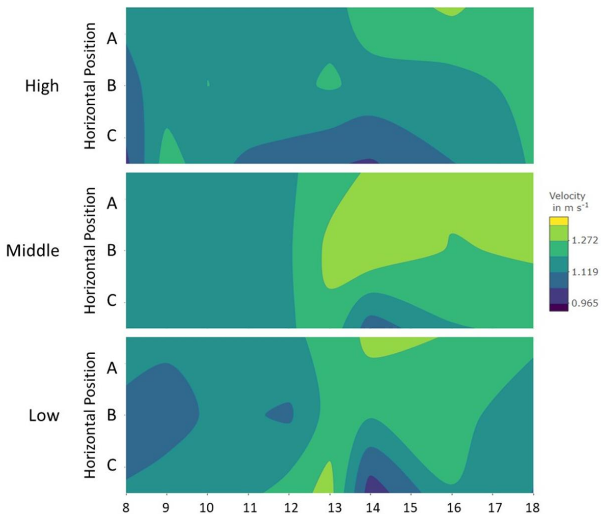
Figure S54. Vertical Velocity Profile of the Chamber at 1.0 \text{ m s}^{-1} (60 Hz), with Flow Straightener
