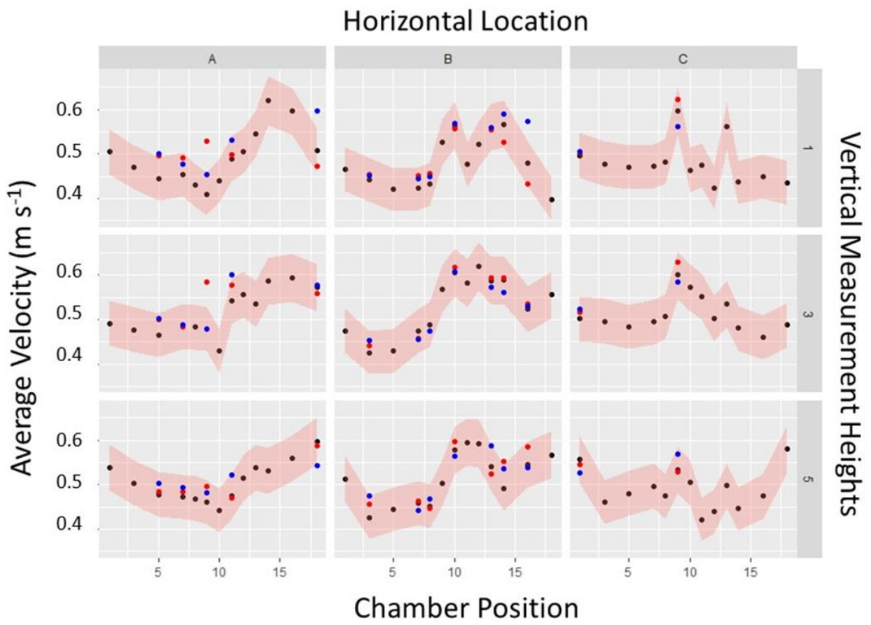
Figure 44. Day-to-Day Variability in Average Velocity at 0.5 \text{ m s}^{-1} , no Flow Straightener
