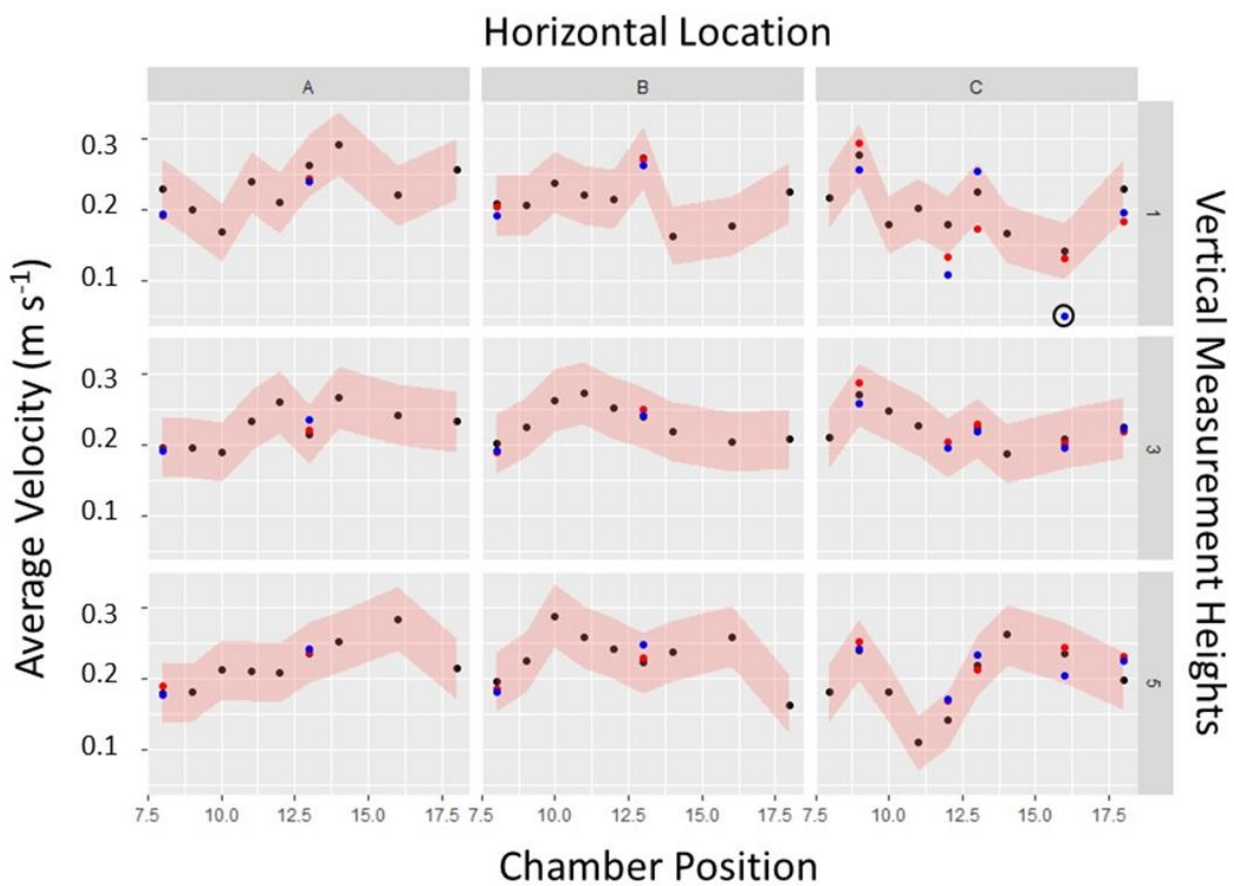
Figure S57. Day-to-Day Variability in Average Velocity at 0.2 \text{ m s}^{-1} , with Flow Straightener
