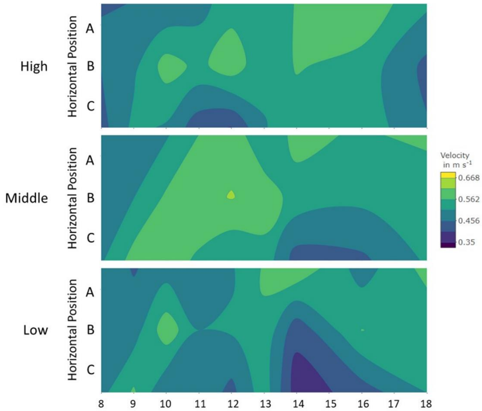
Figure 43. Vertical Velocity Profiles in the Chamber at 0.5 \text{ m s}^{-1} , with Flow Straightener
