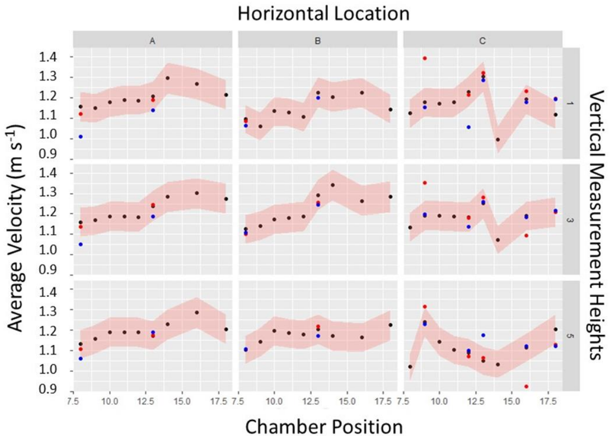
Figure S59. Day-to-Day Variability in Average Velocity at 1.0 \text{ m s}^{-1} , with Flow Straightener
