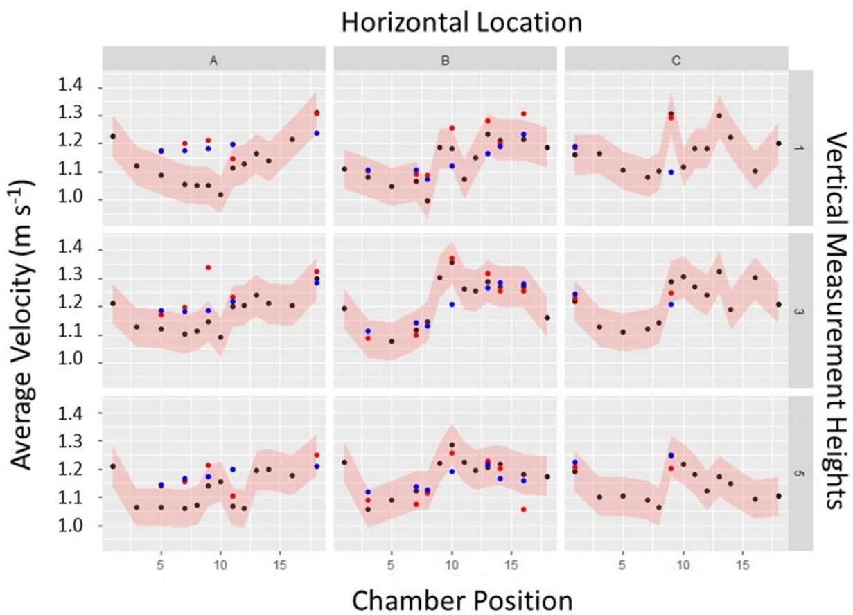
Figure S56. Day-to-Day Variability in Average Velocity at 1.0 \text{ m s}^{-1} , no Flow Straightener
