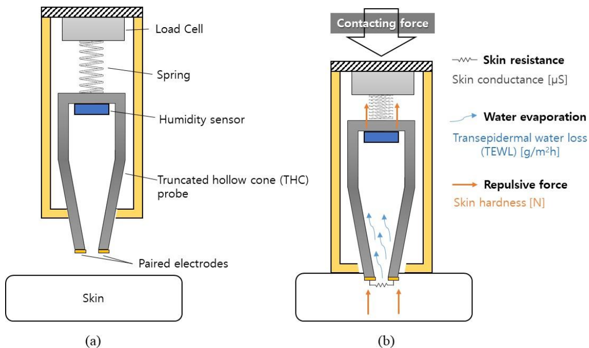
Figure 1. Working principle of the proposed device for assessing the skin conductance, transepidermal water loss (TEWL), and skin hardness, composed of a truncated cone probe, paired electrodes, a humidity sensor, a spring, and a load cell: (a) before skin contact; (b) after skin contact.
