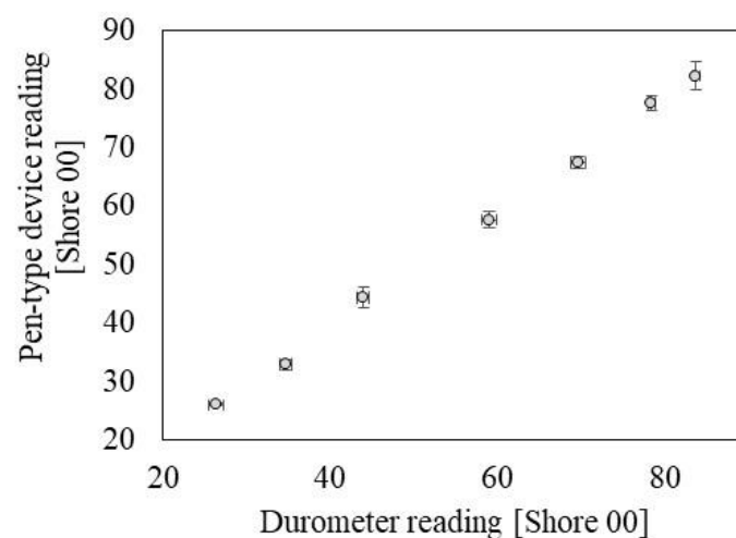
Figure 5. Hardness measurement performance of the pen-type device compared with durometer readings for the reference silicone rubber blocks.
