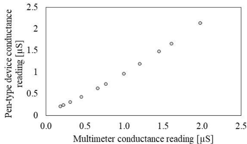
Figure 4. Conductance measurement performance of the present pen-type device for the reference resistors.
