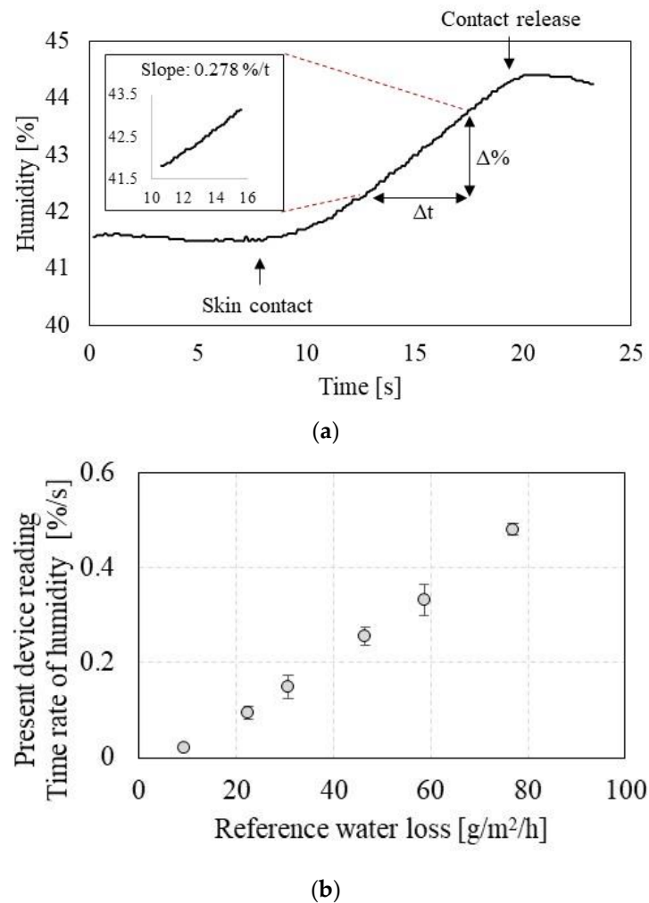
Figure 3. Transepidermal Water Loss (TEWL) measurement characterization, where the truncated hollow cone (THC) probe is in contact with the semipermeable membrane of the artificial skin: (a) the relative humidity profile over time; (b) calibration profile indicating the time rate of humidity depending on the reference water loss from the artificial skin.
