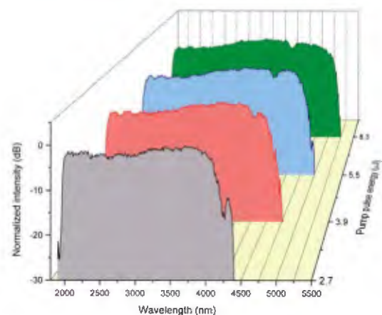
Figure 39: Supercontinuum spectra obtained from 9-m-long InF 3 fibre pumped at 2.02 µm, for pump pulse energies of ~2.7 µJ (36.3 kW), 3.9 µJ (52.4 kW), 5.5 µJ (73.9 kW), and 8.3 µJ (111.5 kW).
