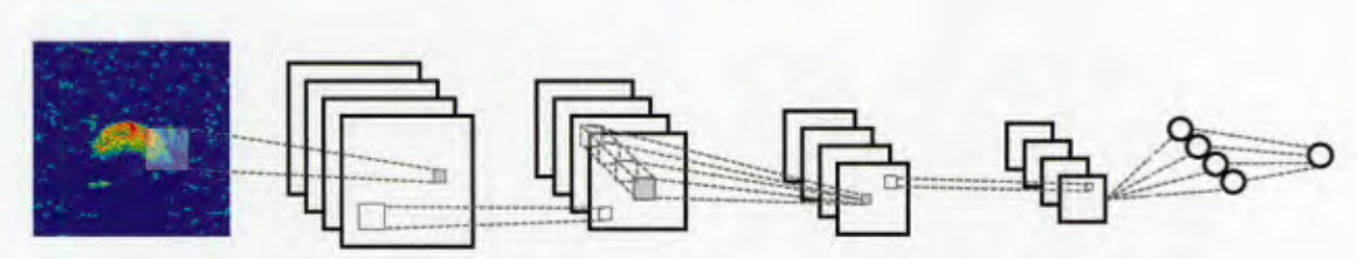
Figure 41: Schematic showing intermediate data representations in a basic CNN architecture with a SAS image chip of a truncated-cone as input.
