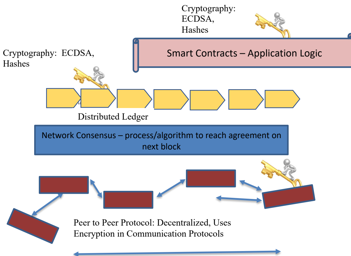
Figure 1 Blockchain Components
