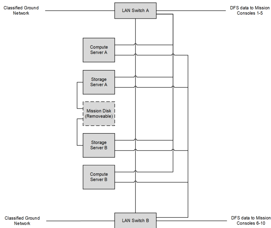
Figure 5: DSF Network Architecture
