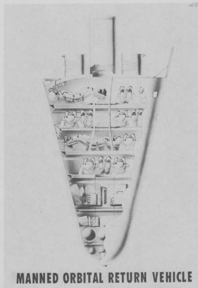
Fig. I-15. Orbital Return Vehicle
