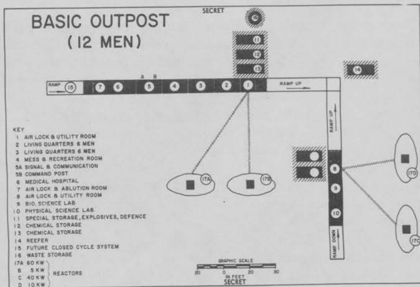
Fig. I-4. Layout of Basic 12-man Outpost
