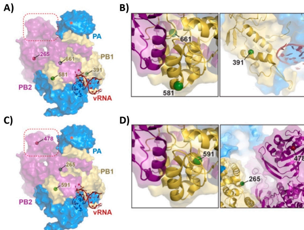
Figure 9. Location of the ts , ca and att mutations of AA and Len MDV in the viral polymerase complex. (A) PB1 (green spheres) and PB2 (purple sphere) mutations responsible for the ts , ca and att phenotype of AA are shown on the reference model of the RNA dependent RNA polymerase, RdRp, complex (PDB ID 5M3H) [58]. The RdRp complex is shown as a surface-rendering model with its subunits PA (blue), PB1 (yellow) and PB2 (purple), and bound vRNA (red). Dotted square (red) indicates the PB2 cap-binding domain. Red asterisk shows the approximate location of the endonuclease catalytic site of PA. (B) Close-up images of the locations of the AA PB1 mutations E581G and A661T (left) and K391E (right). (C) Same as in (A) but for Len. (D) Close up locations of LenV591I (PB1, left), K265N (PB1, right) and V478L (PB2, right) mutations. All images were generated and rendered in the program Pymol [59].
