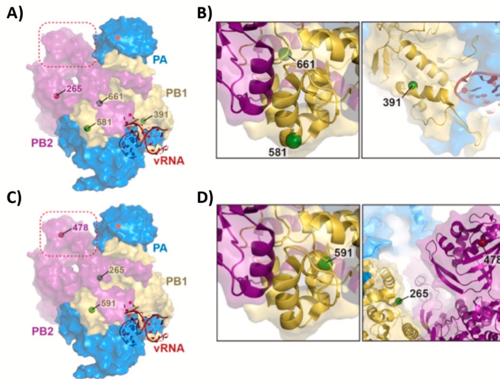
Figure 10: Location of the ts, ca and att mutations of AA and Len MDV in the viral polymerase complex.
