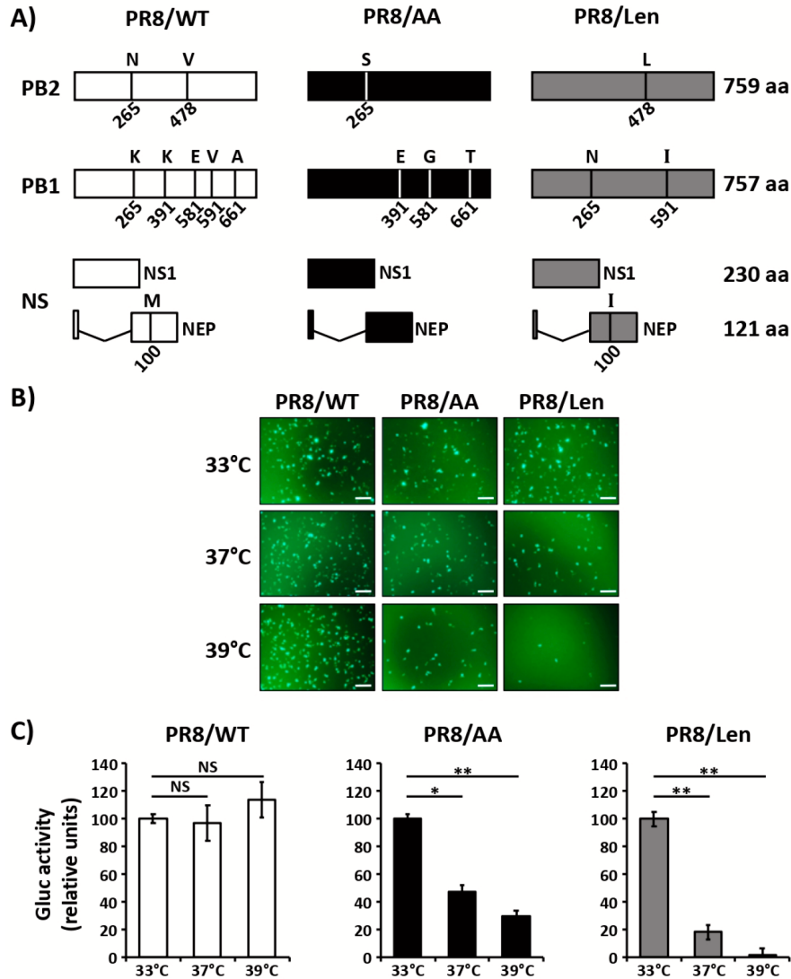
Figure 1: Effect of temperature on the polymerase activity of PR8/AA and PR8/Len.
