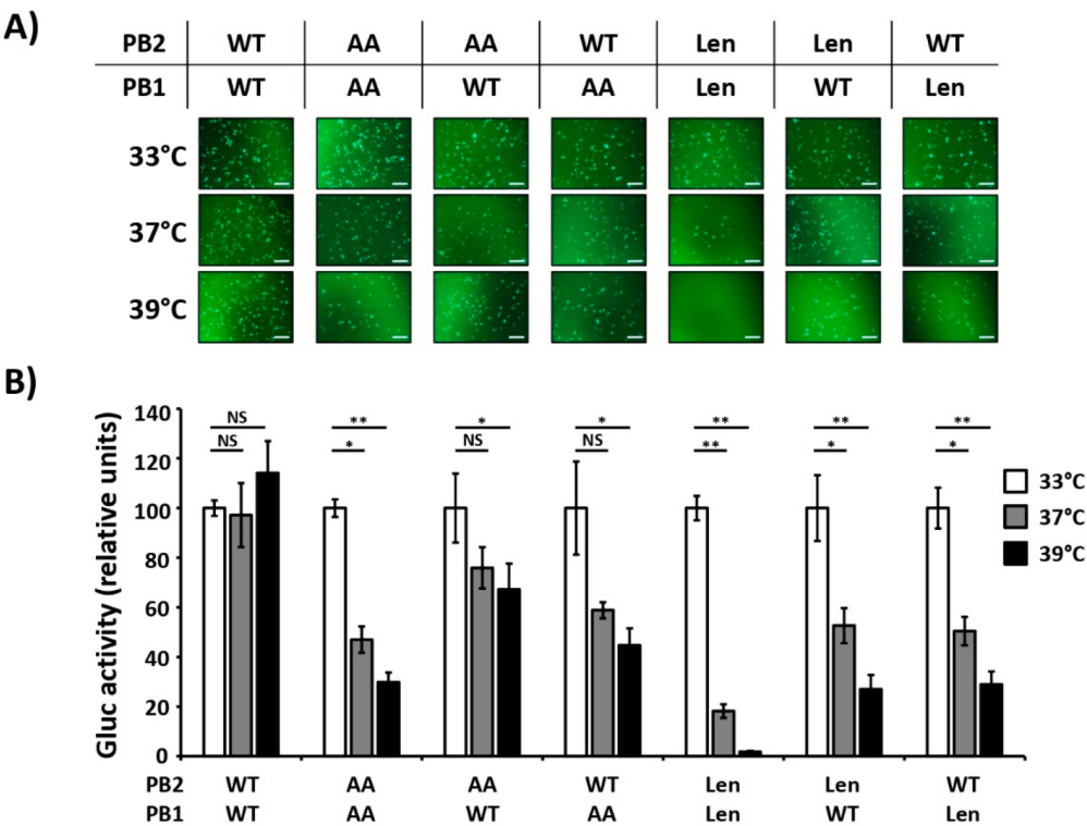
Figure 3: Contribution of PB2 and PB1 mutations of PR8/AA and PR8/Len in the viral polymerase activity at different temperatures.
