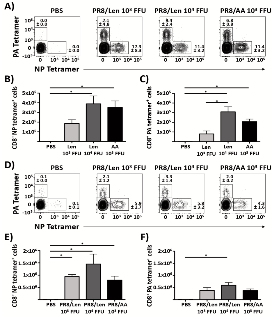
Figure 7: Induction of CD8 T cell responses by PR8/AA and PR8/Len viruses
