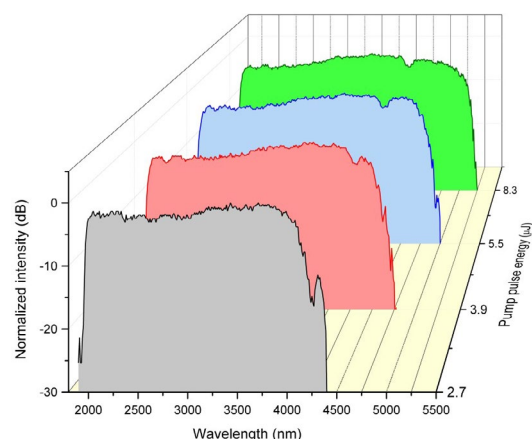
Figure 39: Supercontinuum spectra obtained from 9-m-long InF 3 fibre pumped at 2.02 \mu\text{m} , for pump pulse energies of \sim 2.7 \mu\text{J} (36.3 kW), 3.9 \mu\text{J} (52.4 kW), 5.5 \mu\text{J} (73.9 kW), and 8.3 \mu\text{J} (111.5 kW).
