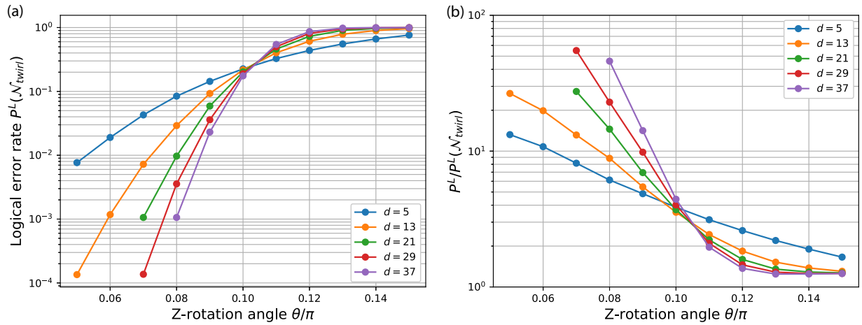
Fig. 3 Comparison between the logical error rates P^L and P^L(N_{\text{twirl}}) computed for coherent noise N(p) = e^{i\theta Z} p e^{-i\theta Z} and its Pauli twirled version N_{\text{twirl}}(p) = (1 - \epsilon)p + \epsilon Z p Z with \epsilon = \sin^2(\theta) . In both cases we used the minimum weight matching decoder. The plot demonstrates that applying the Pauli twirl approximation to the physical noise significantly underestimates the logical error rate in the sub-threshold regime
