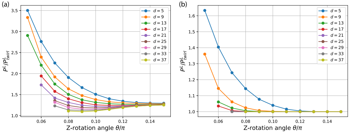
Fig. 5 Coherence ratio P^L / P^L_{\text{twirl}} for the conditional logical channel (left) and for the average logical channel (right). In both cases increasing the code distance makes the logical-level noise less coherent
