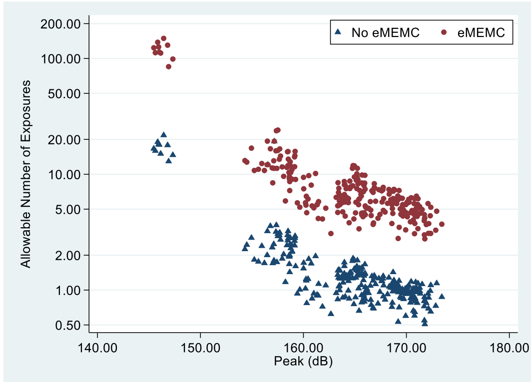
Figure 1. Allowable number of rounds (ANOR) returned by AHAAH as a function of impulsive peak level. Triangles represent ANOR under the unwarned assumption (i.e., no eMEMC). Circles represent ANOR under the warned assumption (i.e., eMEMC).
