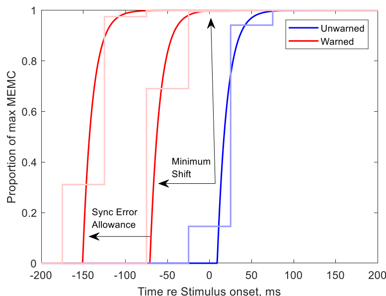
Figure 27. In AHAAH, the unwarned MEMC (blue) is expected to follow the onset of the impulse by 9 ms and then rise to a maximum within about 50 ms, with a morphology similar to a capacitive system that follows time constant of 11.7 ms. The warned MEMC (red) follows the same parameters as the unwarned response, with maximum MEMC occurring prior to stimulus onset (Price, 2007).
