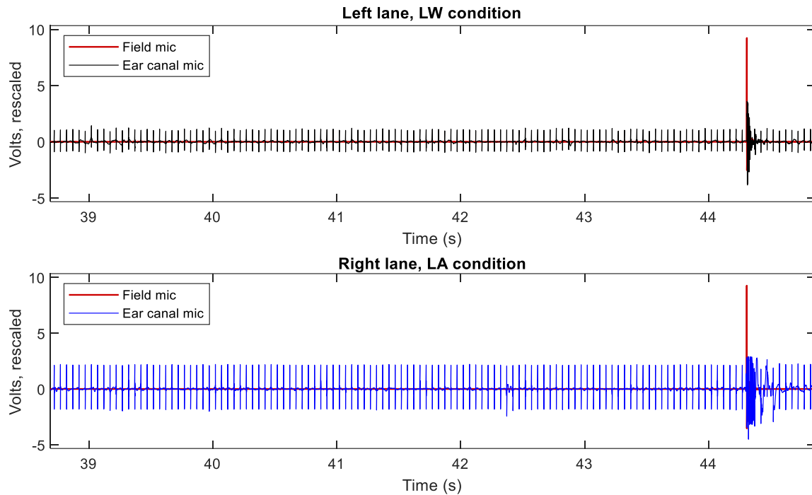
Figure 20. Example of field microphone and ear canal recordings. Participant in left lane waiting (LW); right lane active (LA). Details similar to preceding figure.
