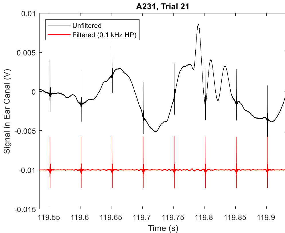
Figure 8. Click-based probe signals, before and after high-pass filtering. Plot represents pressure (Volts) at the probe microphone as a function of time (seconds). Click-based probe signals were presented with a 50 ms inter-stimulus interval. Unfiltered recordings (black curve) revealed that the probe signals were combined with physiological noise in the ear canal, which was minimized using a high-pass filter at 0.1 kHz (red curve, which was displaced by -0.01 V for clarity).
