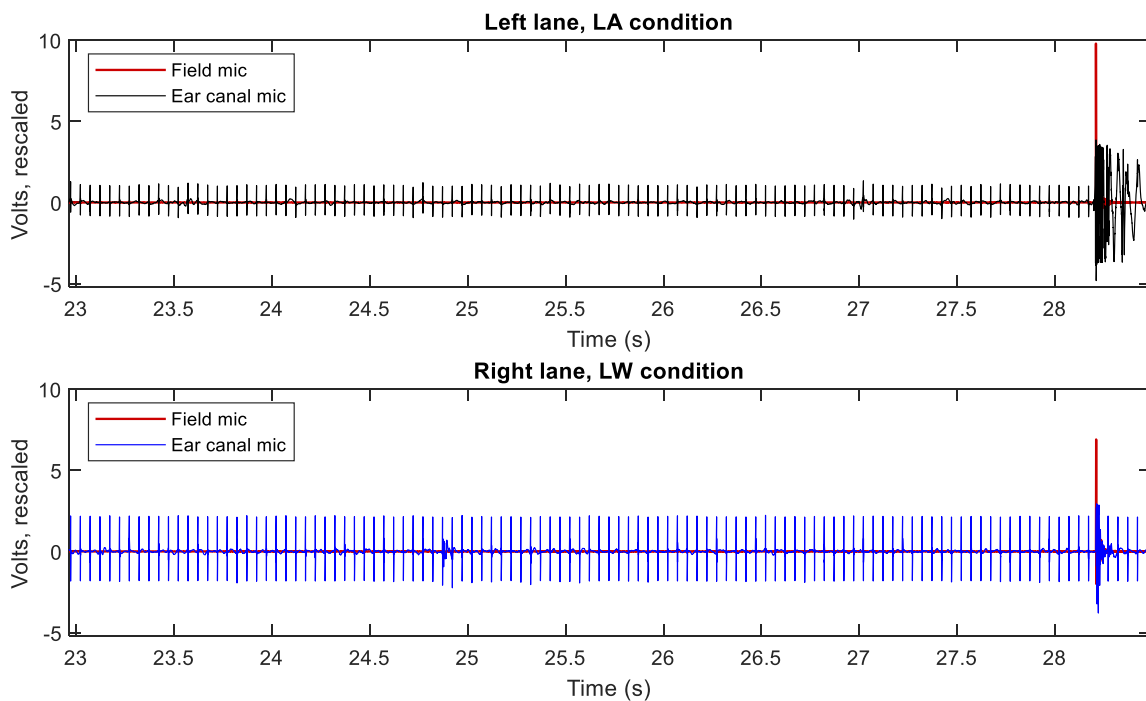
Figure 19. Example of field microphone and ear canal recordings. Participant in left lane active (LA); right lane waiting (LW). The red trace represents the field microphone signal nearest the selected firing lane. The black trace represents the recording taken from the participant in the left firing lane. The blue trace represents the recording taken from the participant in the right firing lane. Click signals (repeated every 50 ms) appear as vertical bars in the black and blue traces.
