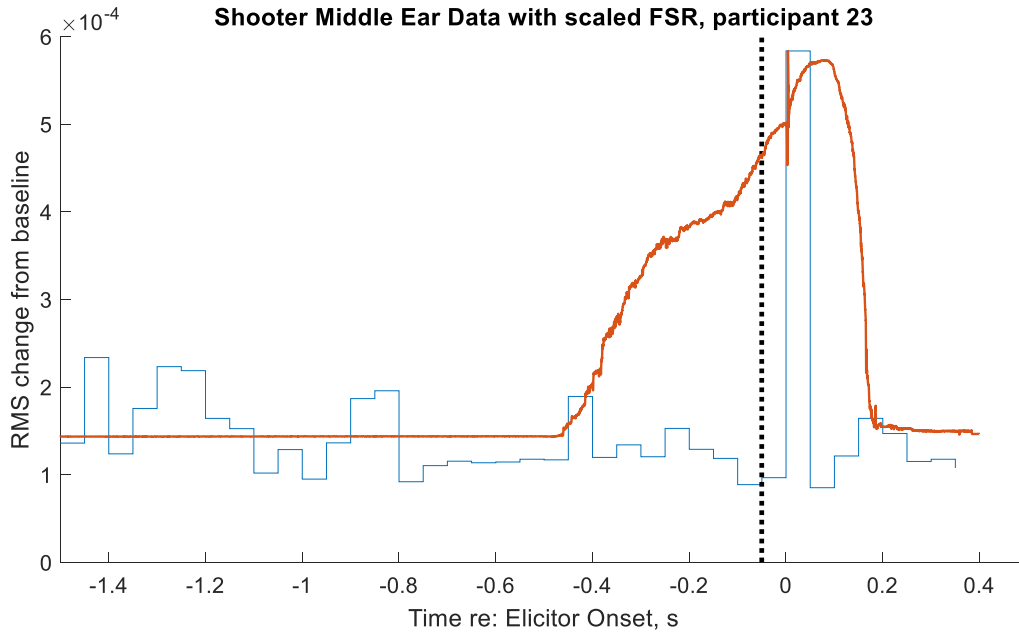
Figure 29. Example of 25 th percentile RMS differences from baseline for participant 23 during the simulated shooter (SH) task with participant ear canal activity (blue) and scaled trigger force activity measured using the FSR400 (red). Trigger force begins to increase approximately 0.45 seconds prior to trigger pull and hammer fall, shown as the red notch at time=0. Ear canal activity remains unchanged from baseline prior to time=0, and the change occurring during the trigger pull/hammer fall may be an rMEMC (UCR), but more likely demonstrates infiltration of the hammer fall signal into the measurement equipment. The acoustic gunfire recording playback occurred 62 ms after time=0, and would not influence the RMS change occurring between 0 and 50 ms.
