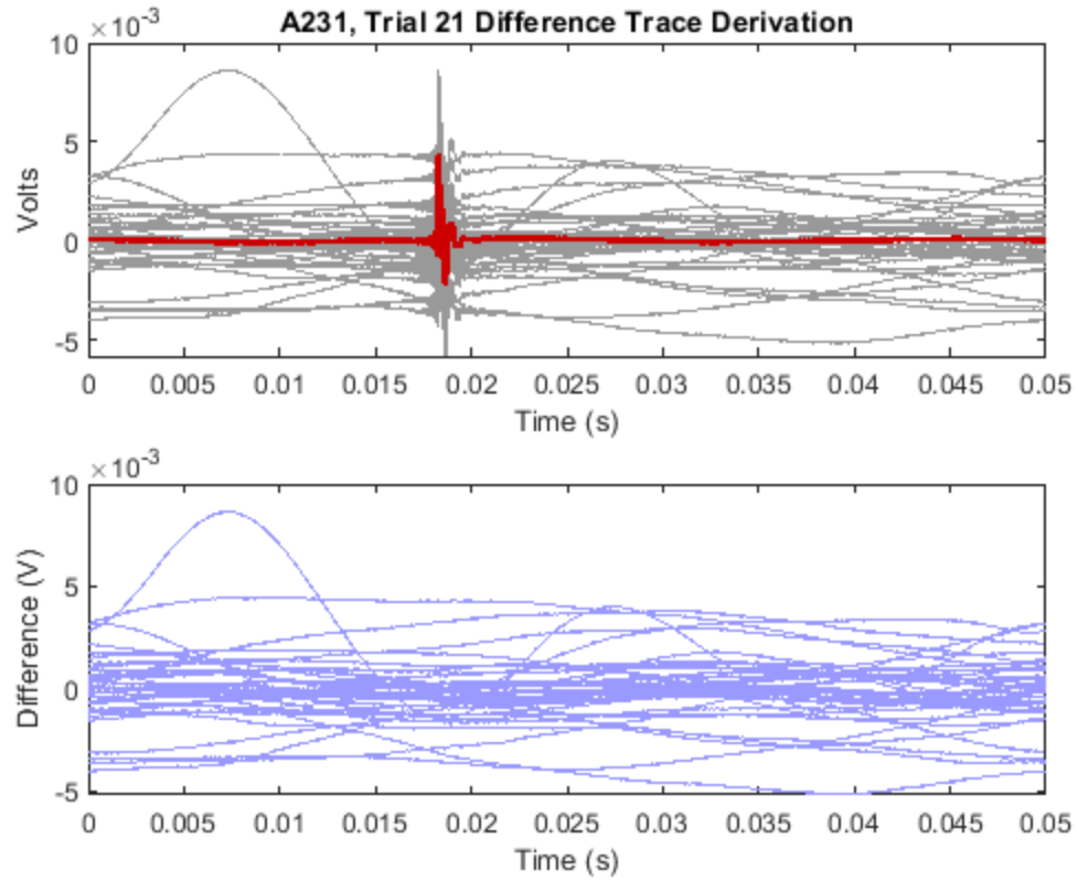
Figure 9. Derivation of difference waveforms for click-based probe signals. Upper plot represents pressure (Volts) as a function of time. Gray curves represent the 0.05 second intervals associated with individual click signals. The red curve represents the time-aligned mean of all clicks outside the elicitor interval (i.e., baseline). Lower plot represents the difference (individual click minus baseline) waveforms for each click within the elicitor interval for a single trial.
