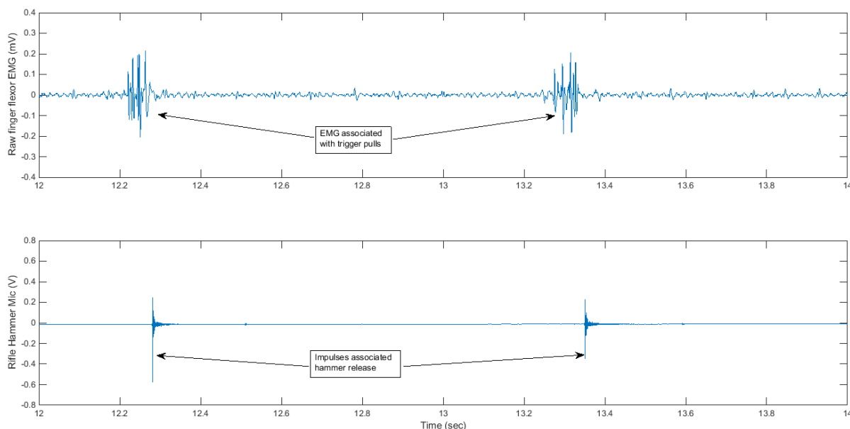
Figure 15. The upper plot represents an EMG recording associated with trigger pulls using a toy gun, and the lower plot represents the associated acoustic signal generated by the hammer release.
