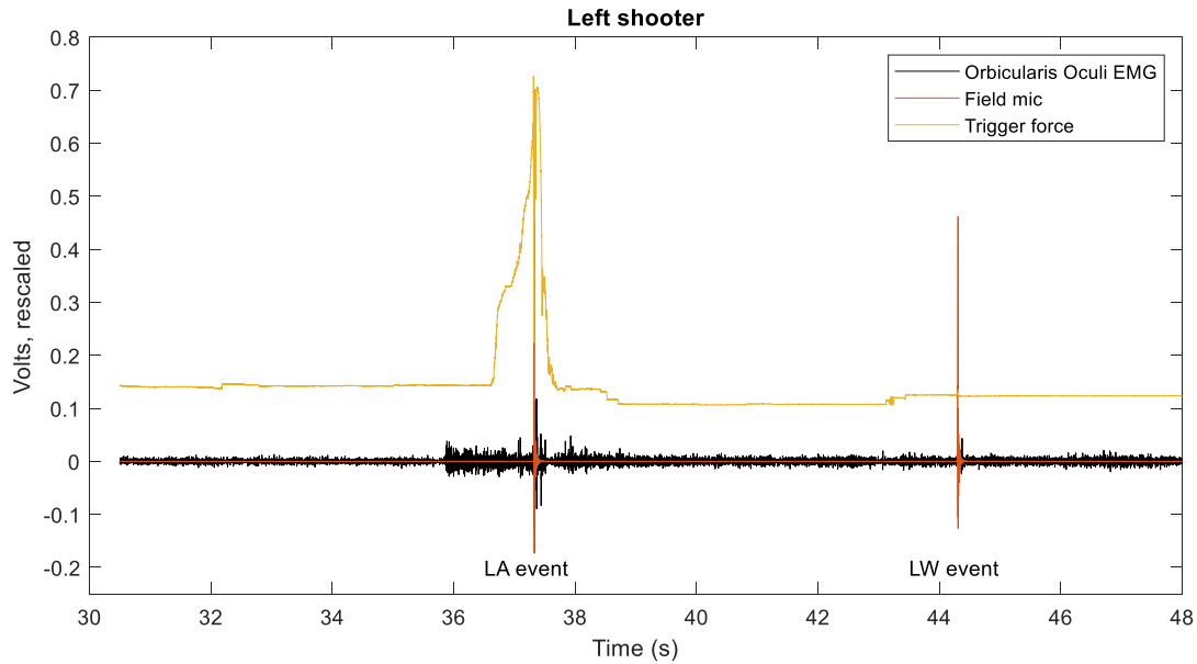
Figure 21. Example of consecutive LA and LW events from the same participant. The black trace represents the EMG signal from the orbicularis oculi (OO) muscle. The red trace represents the waveform recorded at the field microphone. The yellow trace represents the force applied to the gun trigger by the participant. The LA event region begins with activation of the OO muscle, followed by increasing trigger force leading to discharge, which is detected using the field microphone. The LW event region shows only the discharge of the weapon operated by the right shooter, with no significant change in OO EMG or trigger force during the event period, except a small startle response on the OO muscle immediately following blast arrival. Participants fired a standard M4 (5.56 x 45 NATO) service carbine with standard (M193 ball) ammunition on a 25-meter firing range (Figure 22).
