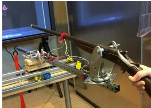
Figure 14. A photo of the distraction activity setup for the Dry Fire condition. The IMU is attached to the barrel. The FSR400 is attached to the gun trigger.
