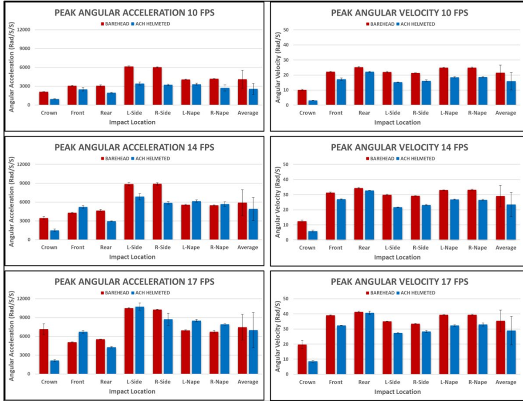
Fig. 6 Peak rotational acceleration (left) and velocity (right) by impact location for bareheaded and ACH helmeted Hybrid-III at 10-, 14-, and 17-fps impacts
