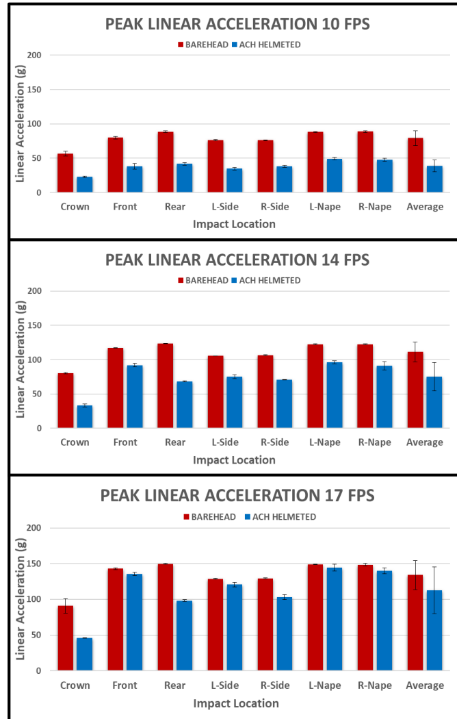
Fig. 5 Peak linear accelerations at each impact location for bareheaded and ACH helmeted Hybrid-III at 10-, 14-, and 17-fps impacts
