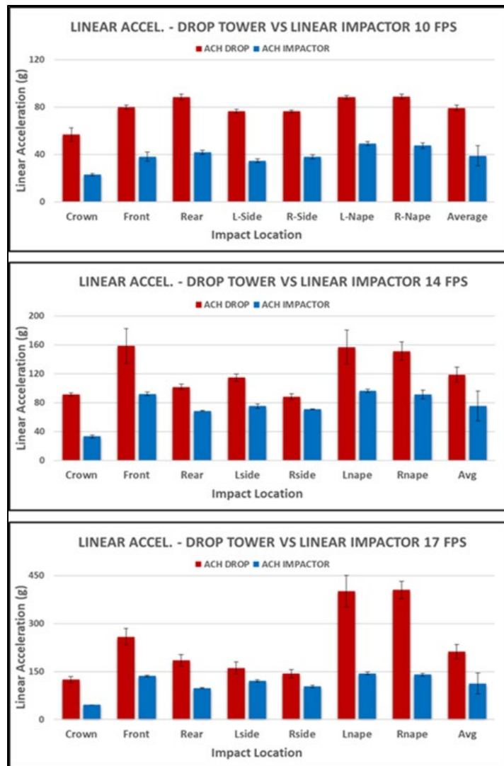
Fig. 7 Comparison of ACH peak linear accelerations between the Army standard drop tower method and nonstandard pneumatic impactor test methods
