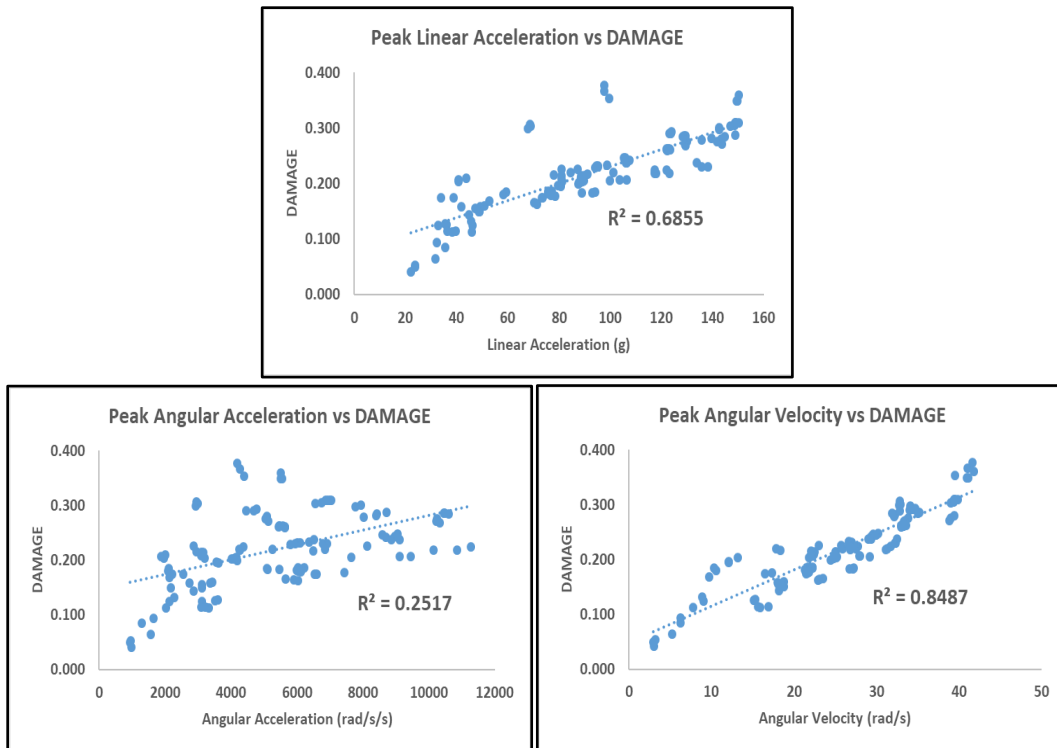
Fig. 9 Linear regression of bareheaded and helmeted headform kinematic response to calculated DAMAGE score
