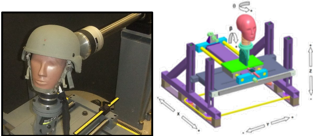
Fig. 2 (Left) Pneumatic ram machine setup. (Right) Target assembly used in the pneumatic ram method consisting of surrogate head and neck on a translating table (Biocore 2019).
