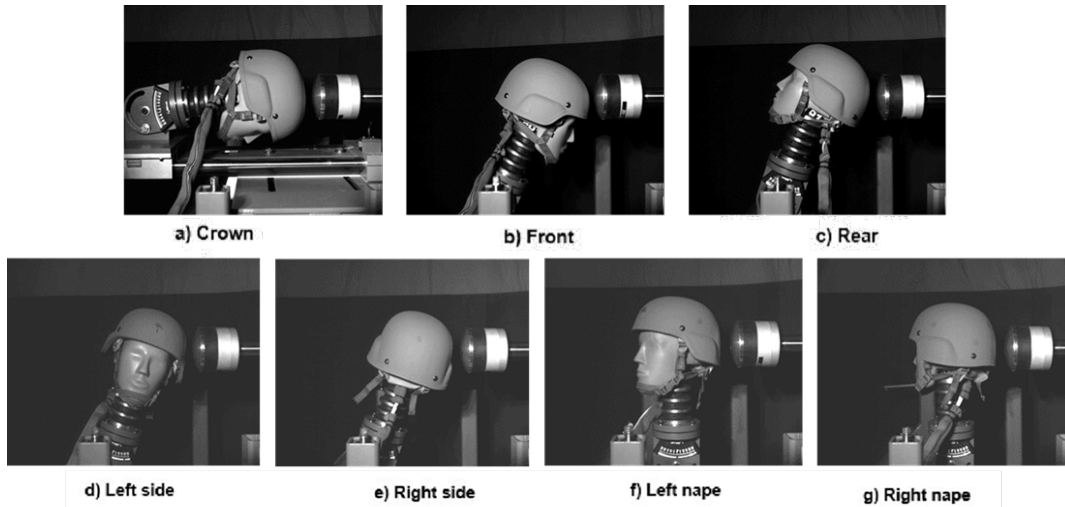
Fig. 3 (Top) Helmet impact location per the ATC blunt impact procedure on the Army standard monorail-based test format. (Bottom) Corresponding helmet impact locations for the pneumatic ram test setup.
