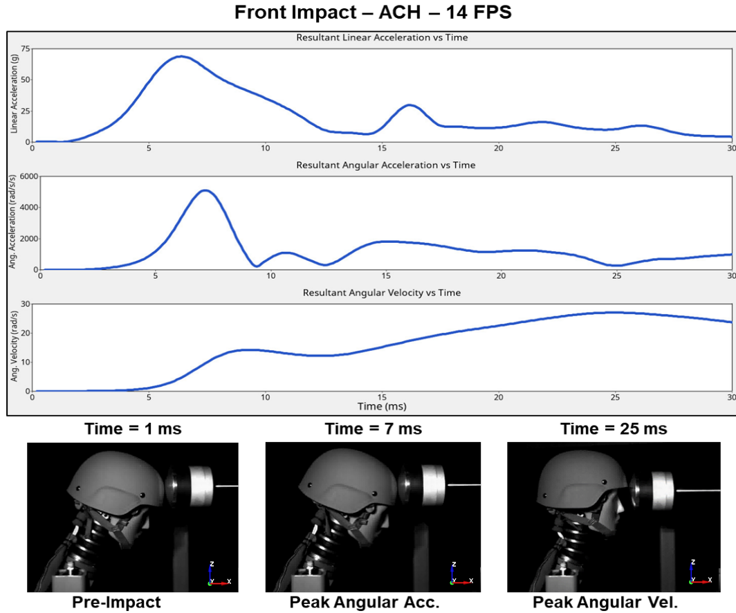
Fig. 4 Example of resultant data traces for a pneumatic ram impact to the front of a Hybrid III head with ACH helmet at 14 fps. (Bottom) Images of the head and helmet at stages between pre-impact and peak angular acceleration during pneumatic ram impact. Compression of the front pads can be observed as the space between the forehead and helmet shell decreases. At peak angular velocity, the head is rotating and neck is flexing away from the impactor.
