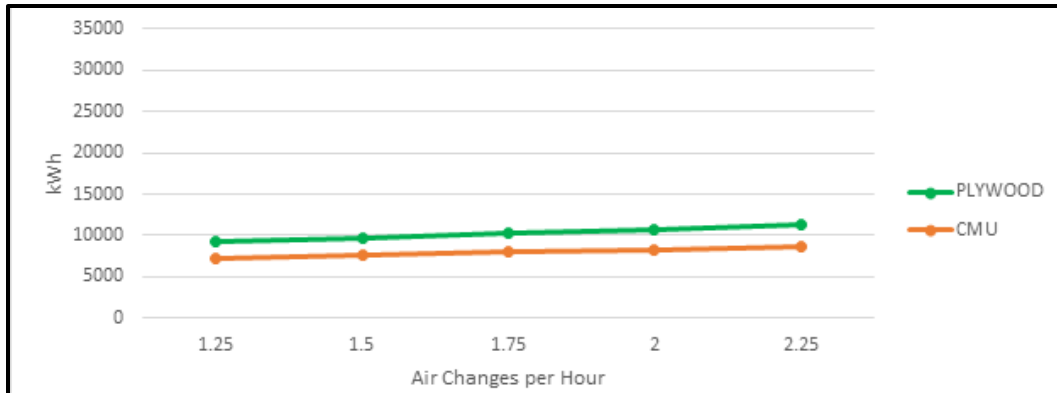
Figure 7. ACH variances for two constructions: R-12 for plywood and CMU, in Atlanta, GA.
