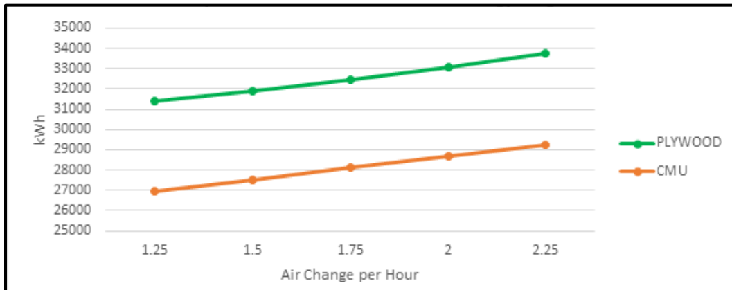
Figure 8. ACH variances for two constructions: R-12 for plywood and CMU, in Fairbanks, AK.
