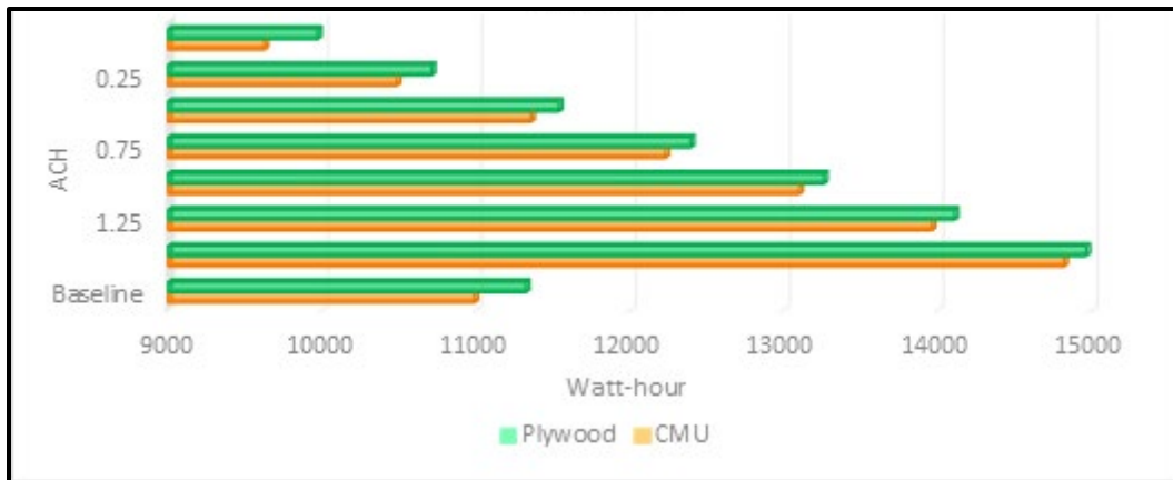
Figure 9. ACH variances for two constructions: R-6 for plywood and CMU.
