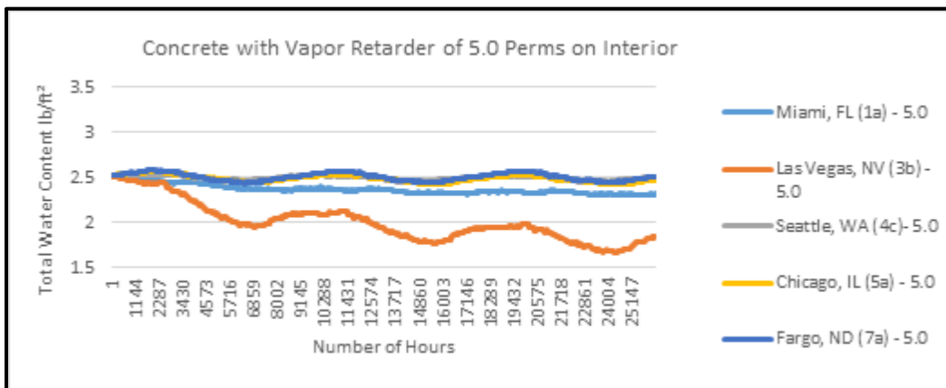
Figure 15. Concrete with vapor retarder of 5.0 perms on interior.
