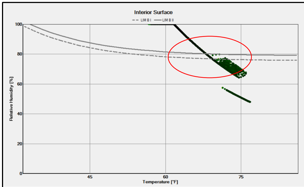
Figure 22. WUFI® isopleth diagram of 1.0 vapor retarder on interior surface in Climate Zone 5a.
