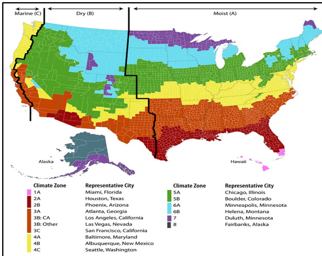
Figure 2. Detailed climate zone map.
