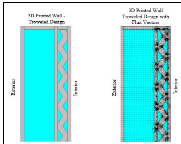
Figure 30. 3D Printed wall troweled with 12-in. exterior cavity, 4-in. interior cavity with 2-in. webbing infill.
