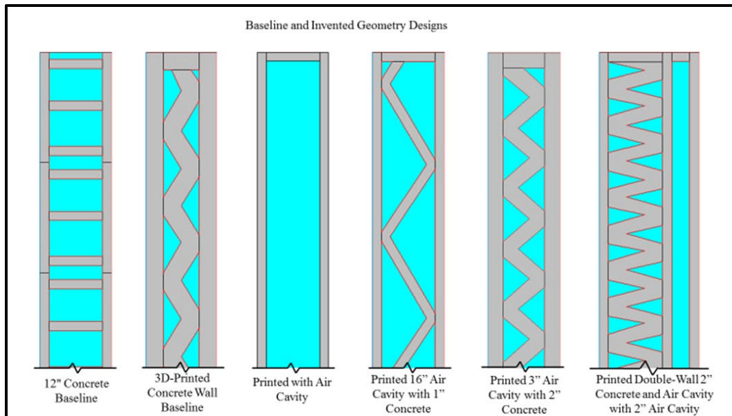
Figure 29. Baseline and proposed wall designs.
