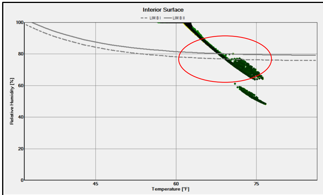
Figure 21. WUFI® isopleth diagram of the baseline B-Hut wall surface in Climate Zone 5a.
