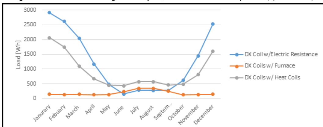
Figure 4. Load of the building over the year, under several HVAC systems (w/insulation).
