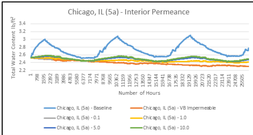
Figure 17. Interior vapor retarder placement in Chicago, IL (5a)
