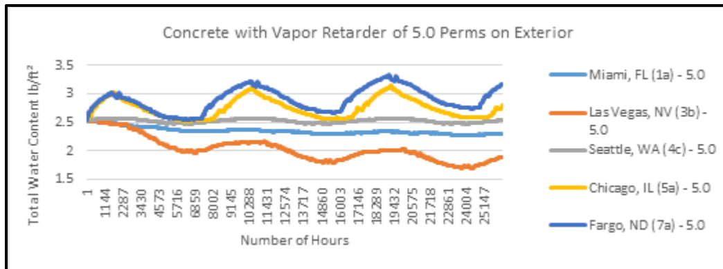
Figure 14. Concrete with vapor retarder of 5.0 perms on exterior.
