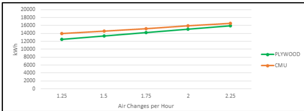
Figure 6. ACH variances for two constructions: R-12 for plywood and CMU, in Urbana, IL.
