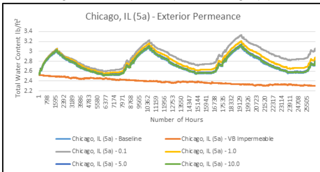
Figure 16. Exterior vapor retarder placement in Chicago, IL (5a)
