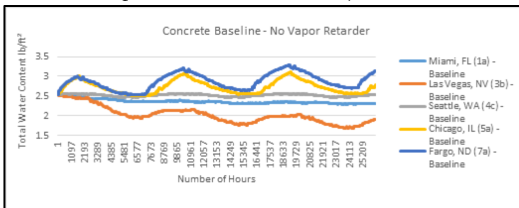
Figure 13. Concrete baseline without a vapor retarder.
