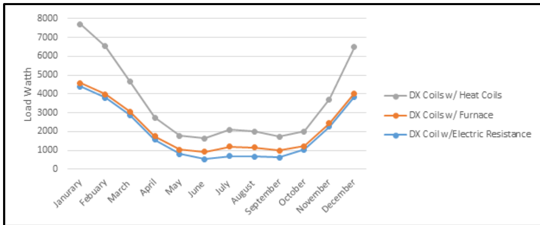
Figure 5. Load of the building over the year, under several HVAC systems (w/o insulation).
