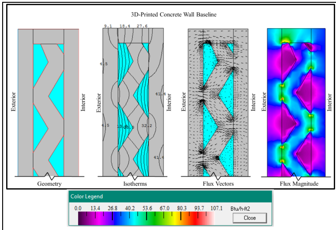
Figure 28. 3D-Printed concrete wall in THERM.
