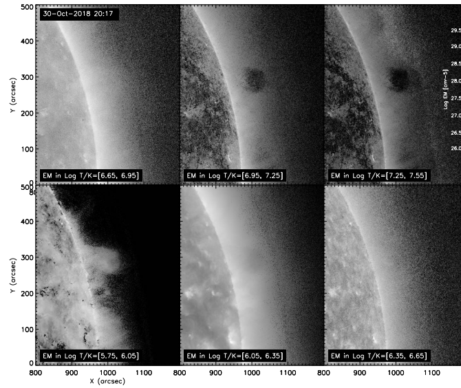
Fig. 15—DEM maps during the eruption of the cavity on 2018 October, 30 at 20:17 UT by the sparse inversion method. Each panel shows the total EM at a different temperature range.
