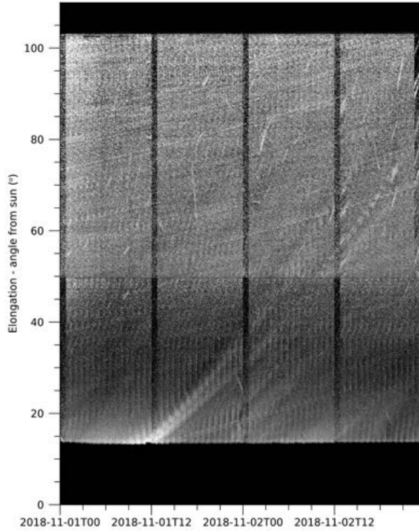
Fig. 8—Height-time plot or J-map of the CME in both WISPR Detectors taken from the spacecraft orbit plane.
