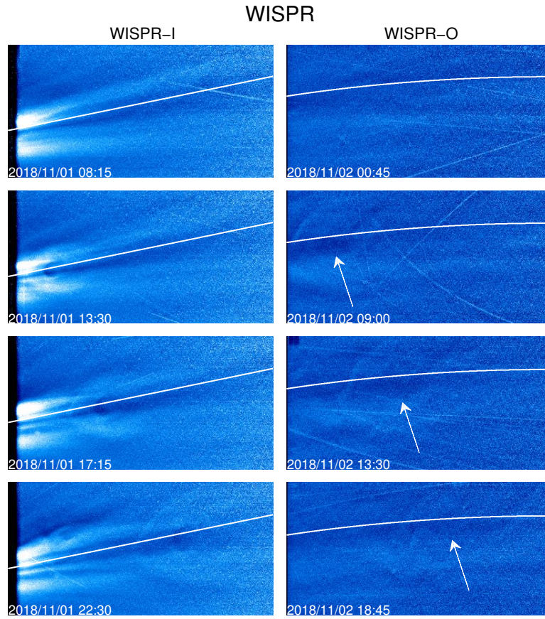
Fig. 7—The CME in both WISPR-I (Left) and WISPR-O (Right). The images from both detectors are cropped to 800x400 pixels. In Detector 2, the white arrows were added to point out where the core of the CME is located. The first image in a each sequence is a pre-event image. The solar equatorial plane has been added as a white line in each image for reference. The bend in the equatorial plane in WISPR-O is a result of the distortion of the detector.
