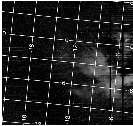
Fig. 3—An image of the 2010-Apr-03 CME from 20:49 UT in HI1-A based on our preliminary background removal techniques. The Helioprojective Coordinate System is overplotted on the data.
