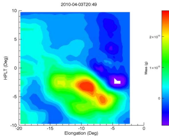
Fig. 4—Contour plot of the mass calculated based on the image from Figure 3. The extra mass in the outer edge of the image is error from the un-shifted background bleeding into the data.
