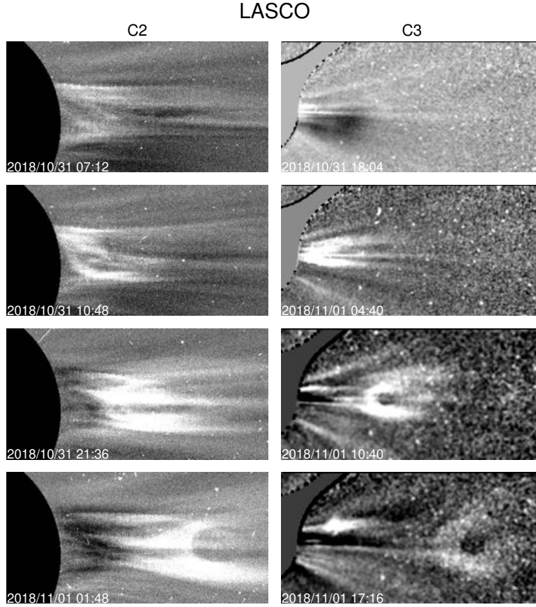
Fig. 10—The CME as observed in LASCO C2 and C3 from the October 31 into November 01. The images from both detectors are cropped to 300x200 pixels. The first frame in each series shows a pre-event image.
