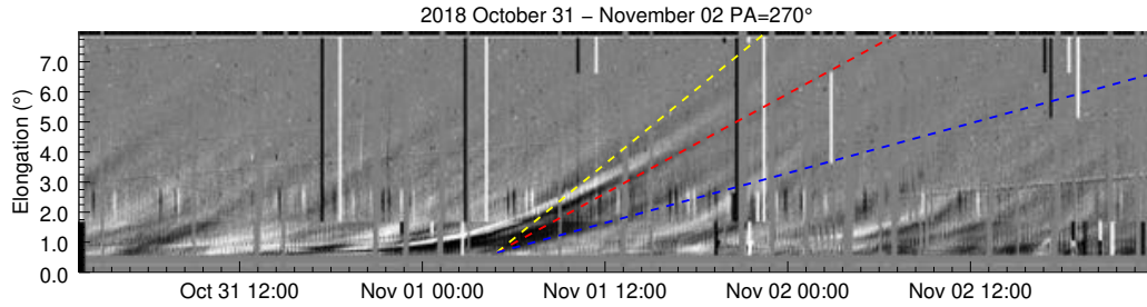
Fig. 11—J-map from LASCO beginning on October 31, combining the C2 and C3 data at position angle 270^\circ (roughly 0^\circ heliographic latitude). The CME is both the bright feature as well as the dark void in front, which correspond to the trailing edge and cavity, respectively. For reference, lines with slopes representing 100 \text{ km s}^{-1} (blue), 200 \text{ km s}^{-1} (red) and 300 \text{ km s}^{-1} (yellow) velocities have been included.
