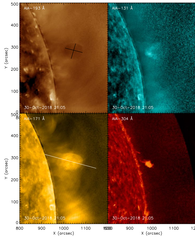
Fig. 13—AIA images during the eruption on October 30. Different wavelengths enhance different elements of the CME including the dark, circular cavity (193 Å; 1.6 MK and 20 MK), the bright trailing edge (131 Å; 0.4 MK and 10 MK), a bright blob that is co-spatial with the cavity (171 Å; 0.6 MK) and the prominence at the base of the eruption (304 Å; 0.05 MK). The black line in the 193 Å frame was used to calculate the size of the cavity. The white line in the 171 Å frame is the approximate direction of motion and was used to measure the height and calculate the velocity of the cavity in AIA.
