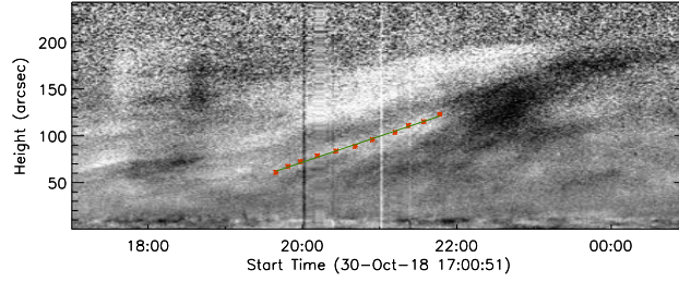
Fig. 14—The height-time plot showing the eruption of the cavity in AIA 171 Å. The position of the slice is shown in the lower-left panel of the Figure 13. The red asterisks mark the positions of the lower edge of the erupting cavity and the linearly fit to the points is in green.
