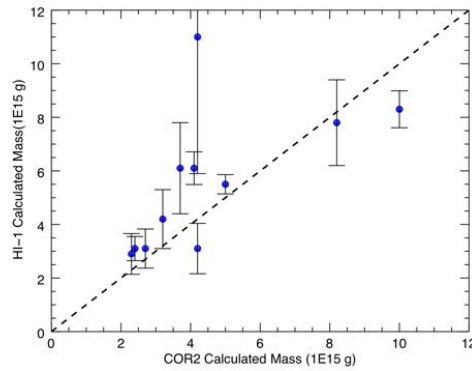
Fig. 6—Comparison between the mass as measured in COR2 and in HI1. The dashed line is the line of unity.
