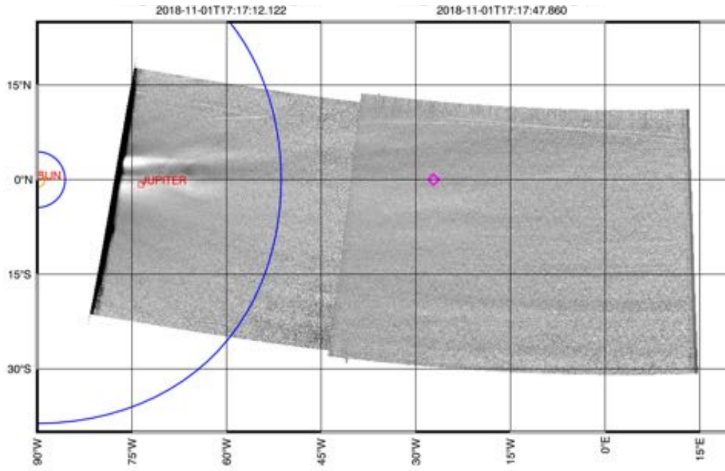
Fig. 9—Observation of the CME in WISPR, in a heliocentric coordinate system with 0^\circ latitude at the PSP orbital plane (see text). The blue circles indicate the approximate position of the C3 field of view based on a projection of the Thomson sphere onto the image plane and ignoring the longitudinal separation of the spacecraft. The pink diamond represents position of the velocity vector of the spacecraft on the image plane. The position of Jupiter is marked as well.
