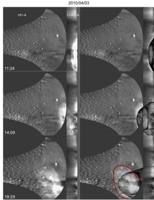
Fig. 2—A GCS fitting along with data from a CME observed 2010-Apr-03 by SECCHI-A. The images are projected onto a rectangular coordinate system, with a linear elongation from the Sun on the x-axis and position angle in the instrument reference on the y-axis. This projection allows COR2 and HI1 images to be combined into a single common field of view. The difference between the model and the data rises sharply as the CME leaves the low corona. In addition to the deviations along the CME front caused by the simplistic rigidity of the model (red line), there is more complicated physics going on behind the CME, where a clear trailing edge is forming and the legs of the ejecta remain narrow.
