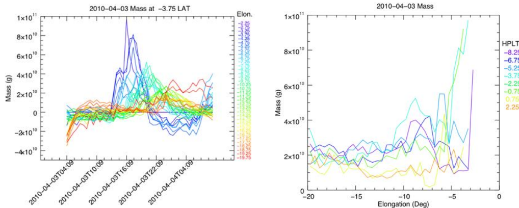
Fig. 5—Left: Each line is a simulated in-situ plot of the CME mass at -3.75^\circ (near the CME nose) as the 2010-Apr-03 CME passes at different height. Right: Each line shows the evolution of mass as the CME propagates away from the Sun for a different helioprojective latitude.
