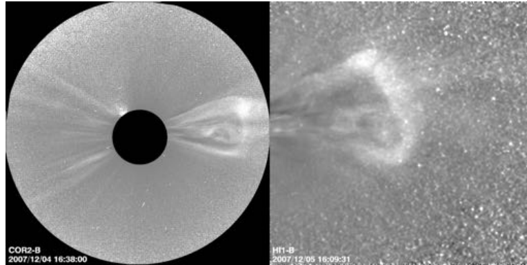
Fig. 1—SECCHI images from COR2-B and HI1-B of the same CME about a day apart, illustrating the observed structural evolution. Out to the edge of COR2, the CME appears to have the classic flux rope shape with a rounded front and interior cavity. In HI1, the front has flattened and the interior cavity has lost definition. The morphological changes with height could indicate a loss of coherence in the magnetic field but instrumental and observational effects between instruments must be mitigated.
