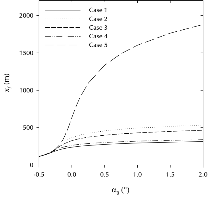
Figure 1. Influence of small elevation angle upon projectile range for projectiles fired from 1 m in elevation.
