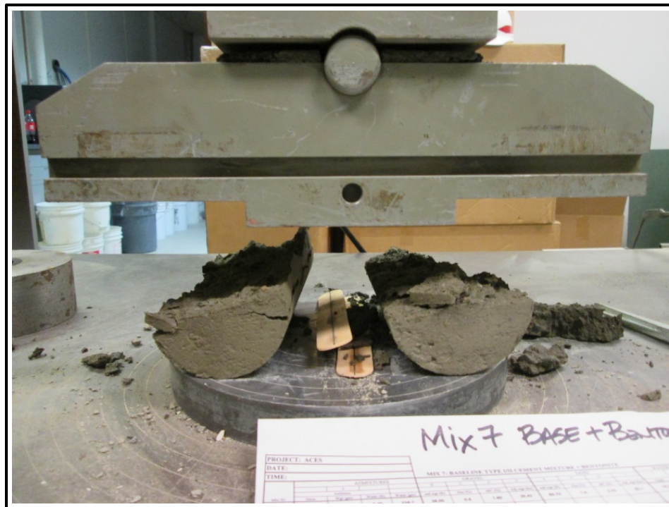
Figure 3-12. Mix 7 Base+Bentonite splitting tensile strength test cylinder at 4-hr test age after failure.
