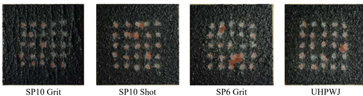
Figure 17 – As-received impact resistance results for Nonskid C
