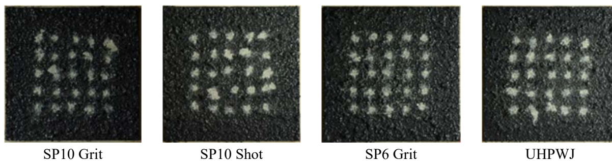
Figure 15 – As-received impact resistance results for Nonskid B
