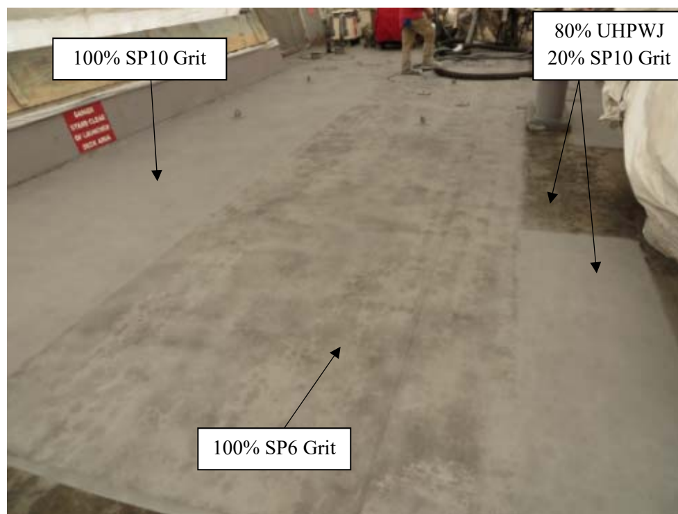
Figure 6 – Overview of the DDG missile deck after final surface preparation
