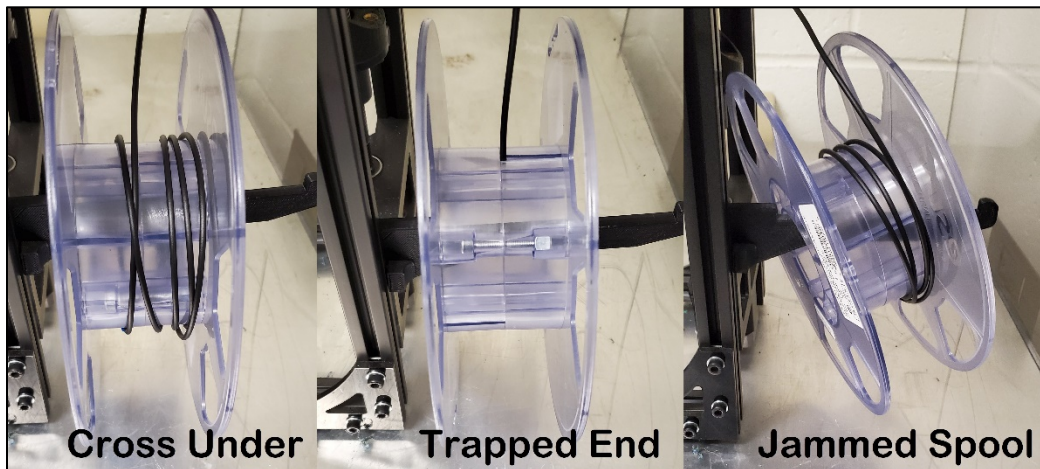
Fig. 13 Scenarios of filament reel becoming jammed
