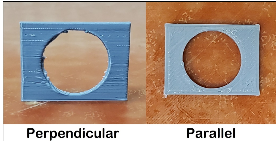
Fig. 5 Hole formation
