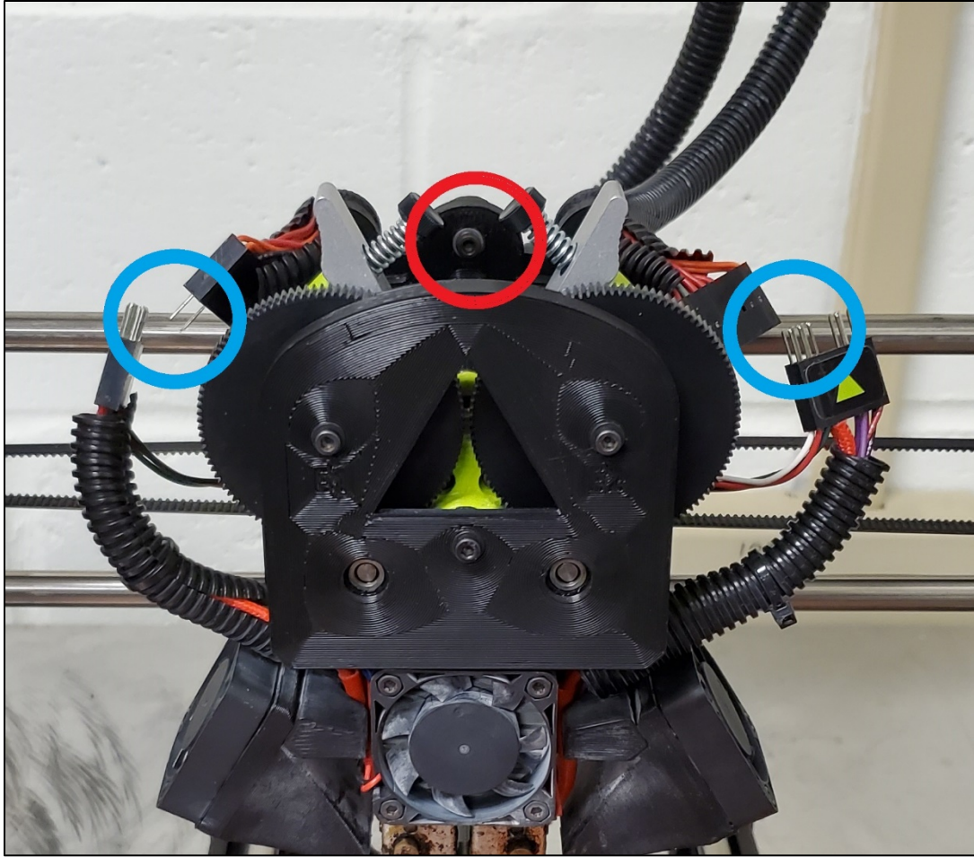
Fig. 19 Removing Dual Extruder v3
