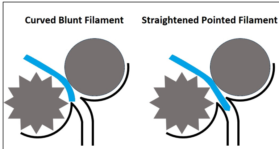
Fig. 7 Proper filament preparation reduces feeder cog lodging
