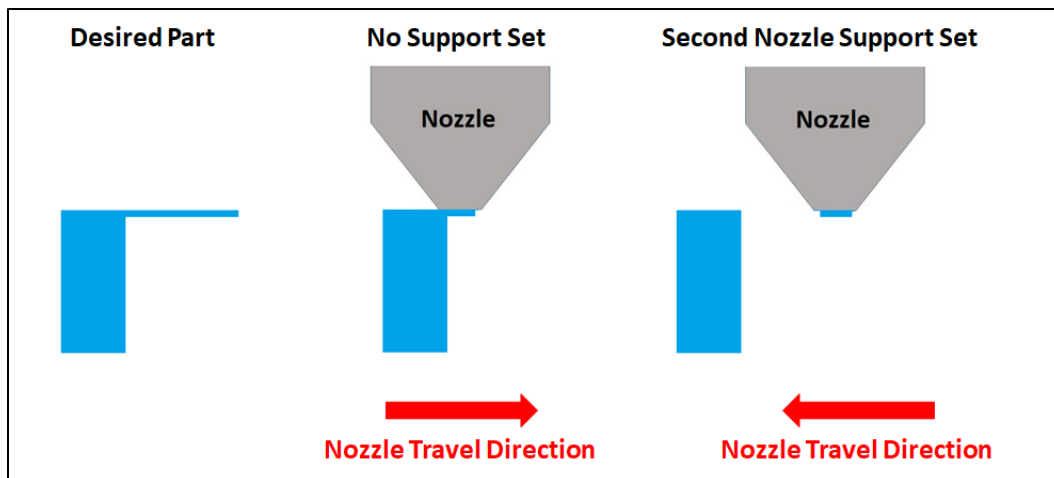
Fig. 10 Support option effect on nozzle path
