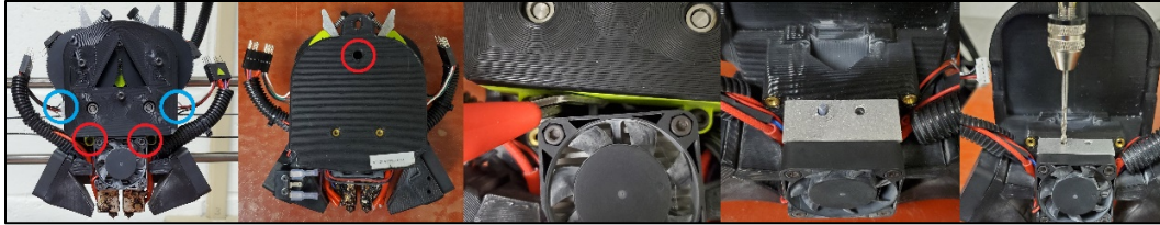
Fig. 20 Nozzle cleaning
