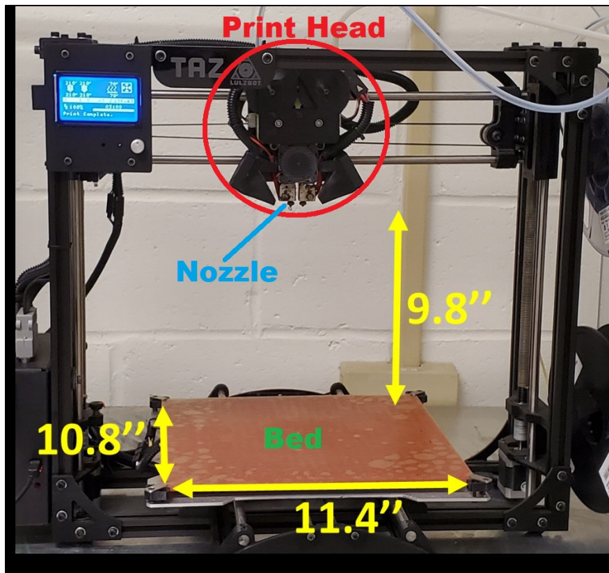
Fig. 2 Printer layout
