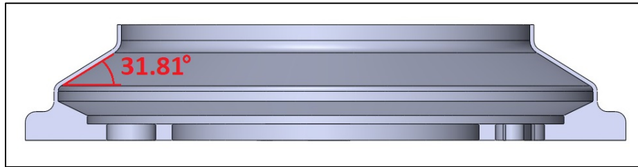
Fig. 9 Maximum unsupported overhang
