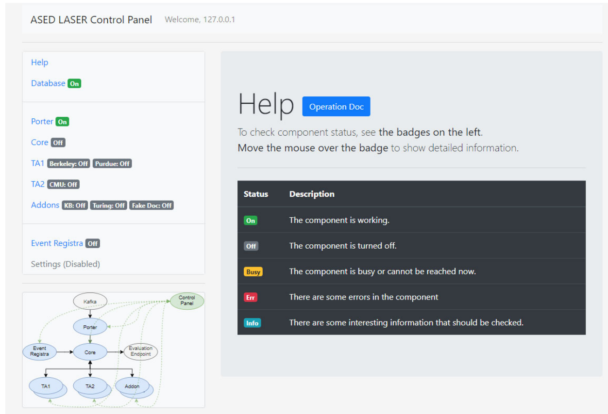
Figure 2. The LASER System UI.
