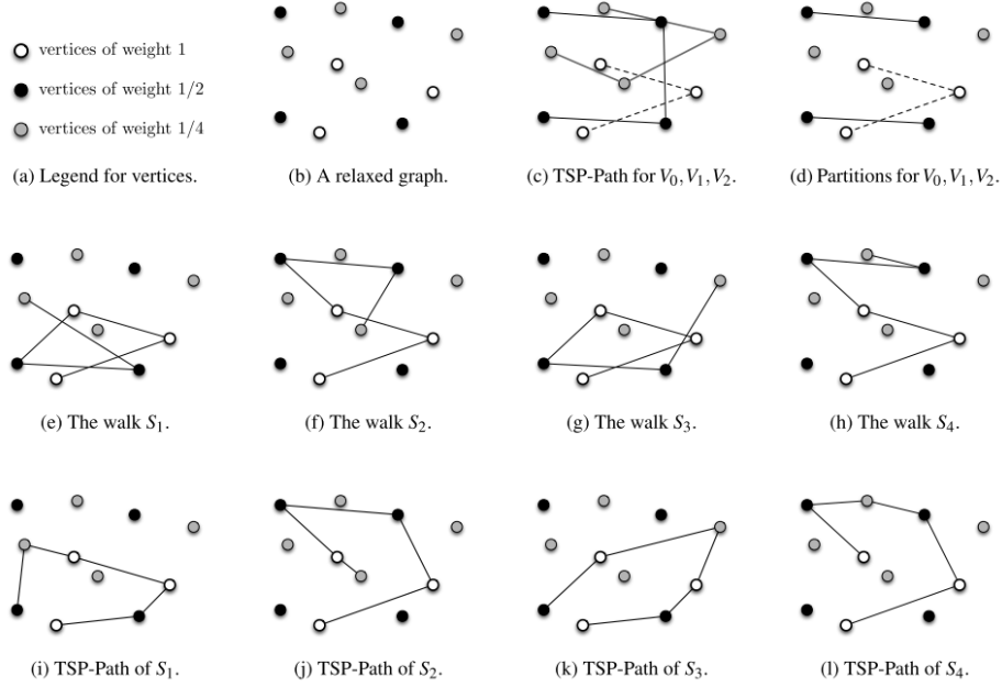
Figure 2.4. Example of the node partitioning algorithm from [3] (original image from the source), where multiple subtours are constructed with high priority nodes being included in more subtours than those of low priority.
