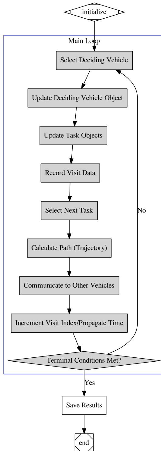
Figure 3.7. Data flow diagram for the PUMPS main loop, from initialization to termination.
