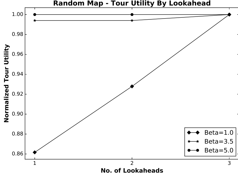
Figure 4.20. Increasing lookahead increases the final tour utility.
