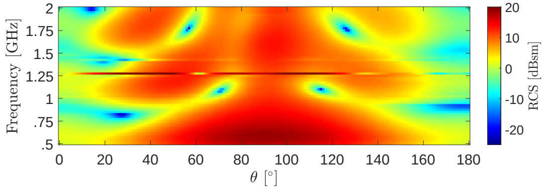
Figure 5.9: RCS Reconstruction with first 24 modes.
