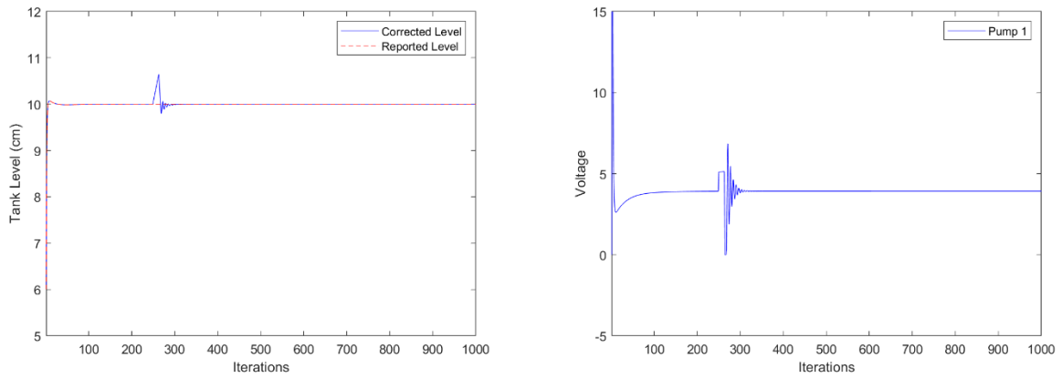
Figure 6.18. System Response to Stuxnet-like Attack #4 with LSTM Ensemble Controller.
