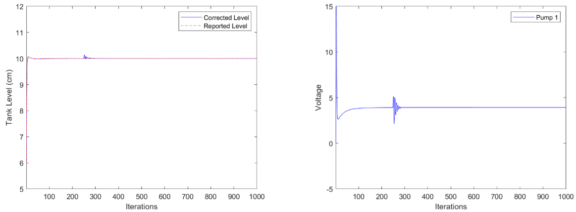
Figure 6.19. System Response to Stuxnet-like Attack #4 with Proposed Controller.
