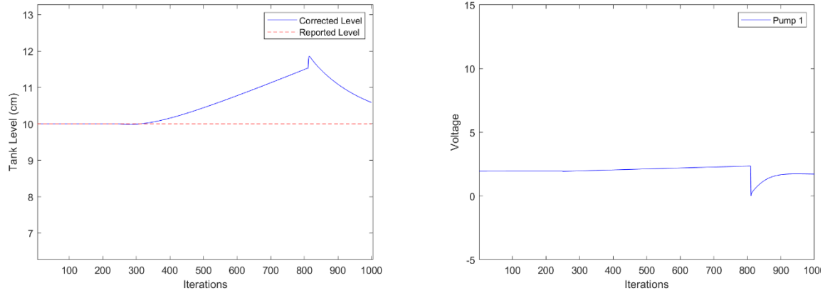
Figure 6.17. System Response to Stuxnet-like Attack #4 with Comparison Controller.
