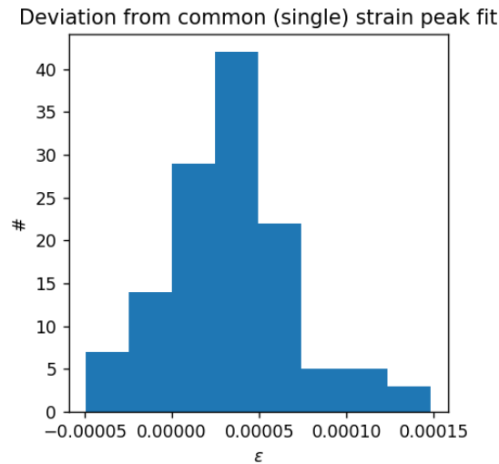
Figure 9. Distribution of difference between fit for \varepsilon_{yy} component, taking a common strain to fit peaks and average of least squares solution with distinct strain evaluated for each peak.
