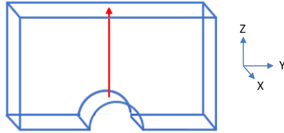
Figure 10. Geometry of calibration scan on the water-jet cut but un-welded reinforcement arch from Specimen #2. The red vector indicates the line along which the scan was performed.
