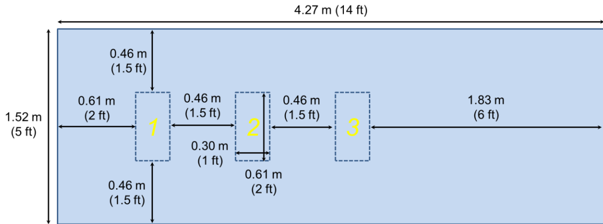
Figure A1. Schematic of the cutting diagram for the 25.4 mm (1-in.) thick plate of HSLA-100 steel showing the location of the sub-plates removed by water-jet cutting to serve as the three “sister samples” for the project.
