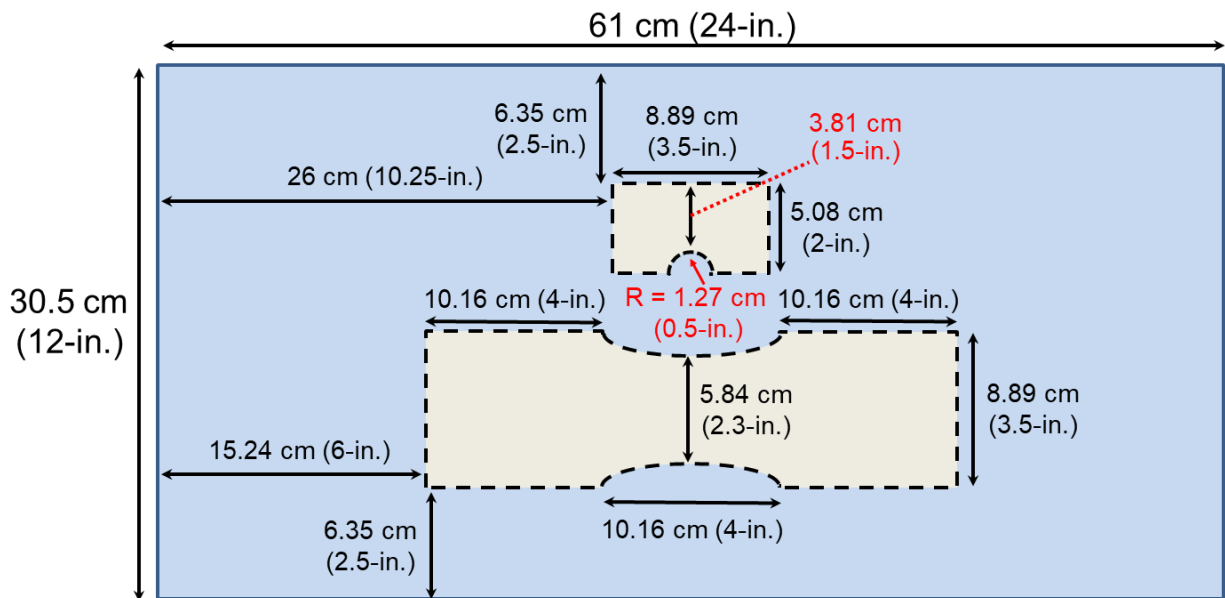
Figure A2. Schematic of the cutting diagram for the 25.4 mm (1-in.) thick HSLA-100 steel sub-plates showing the location of the dog-bone and reinforcement arch removed by water-jet cutting to serve as the basis for the final two “sister samples” for the project.
