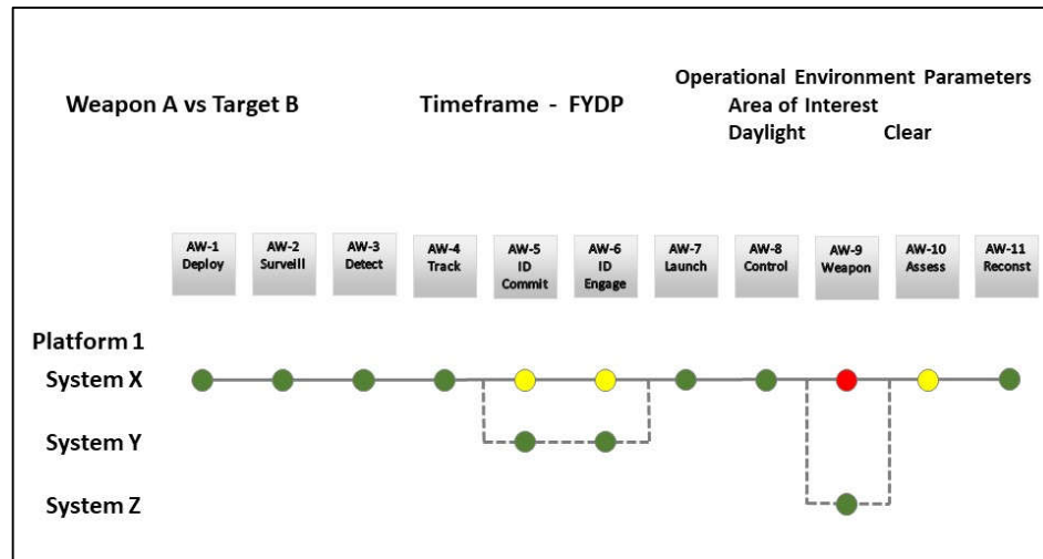
Figure 1. Scored event chain applied to a SoS consisting of three systems has complexity (14, 15 ,4)
