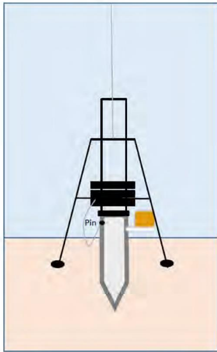
Figure 7 If feet of frame sink in, cotter pin will not be released from sampler (Pin shown, left).
