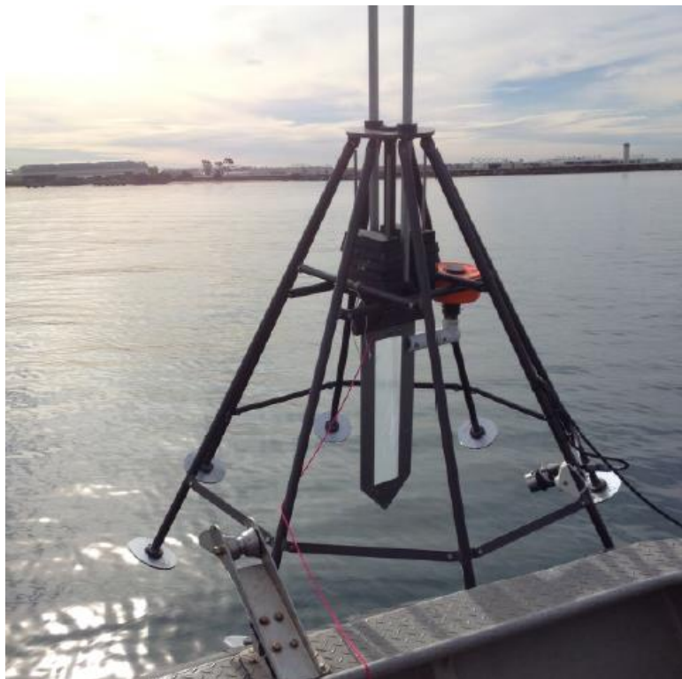
Figure 3 Drive-frame system.
