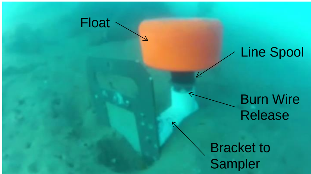
Figure C-4. The timed-release retrieval float.
