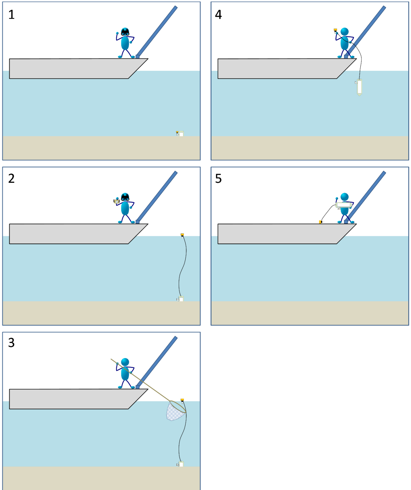
Figure 18 Retrieval cartoon for the Passive Push system.
