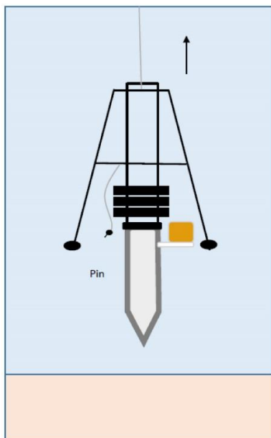
Figure 8 If sediment jams the frame socket, it may cause the sampler to remain in the drive frame, despite release of the cotter pin.
