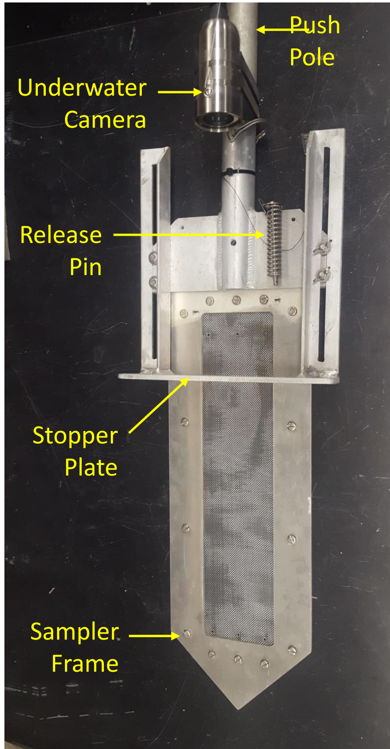
Figure C-2. Push pole system.
