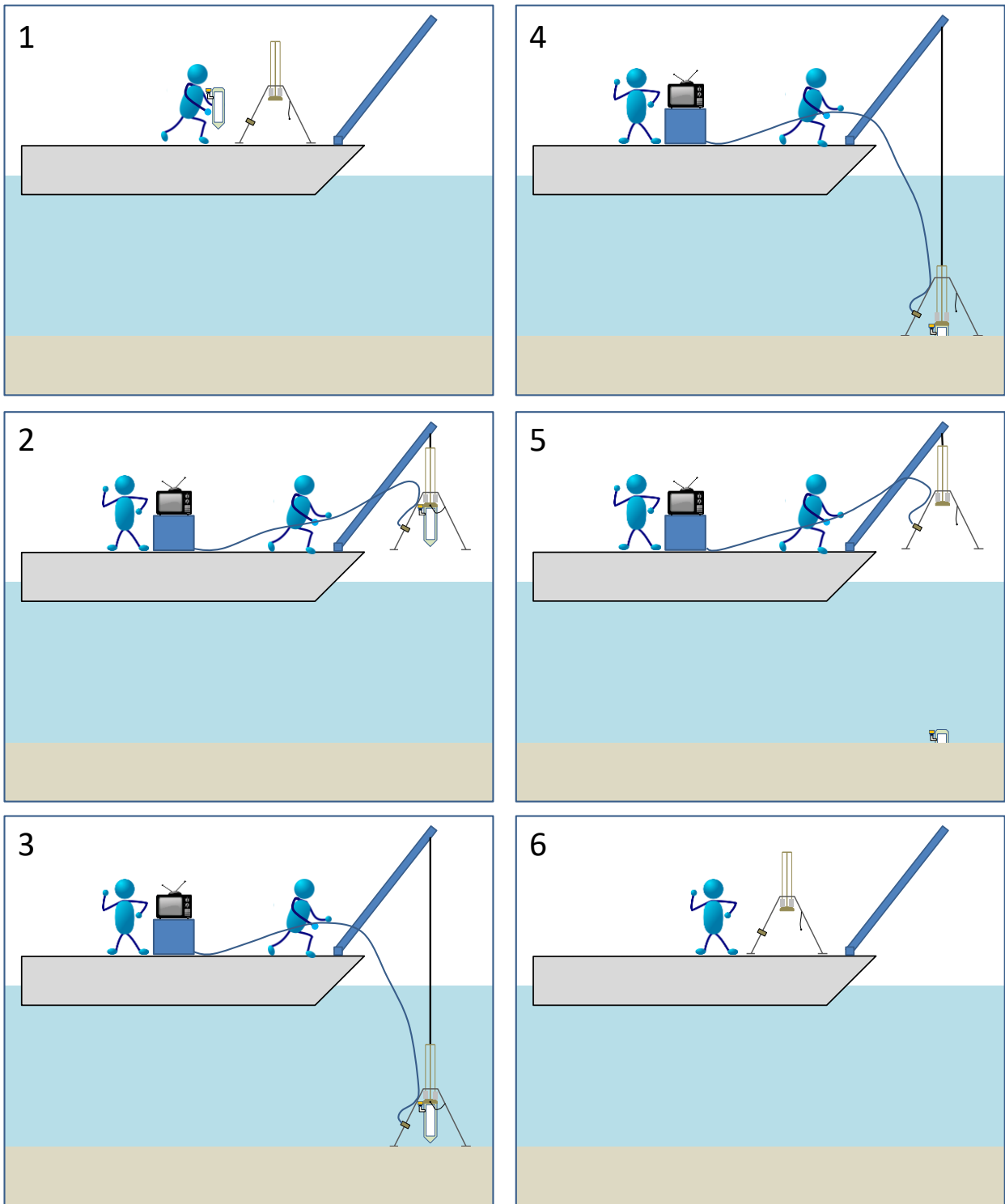
Figure C-6. Deployment cartoon for the Passive Push drive-frame deployment system.
