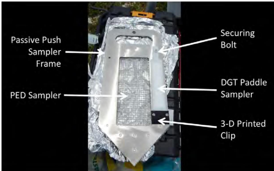
Figure 5 Sampler frame with both polyethylene device (PED) and diffusive gradient in thin film (DGT) samplers loaded for deployment at Tern Island.
