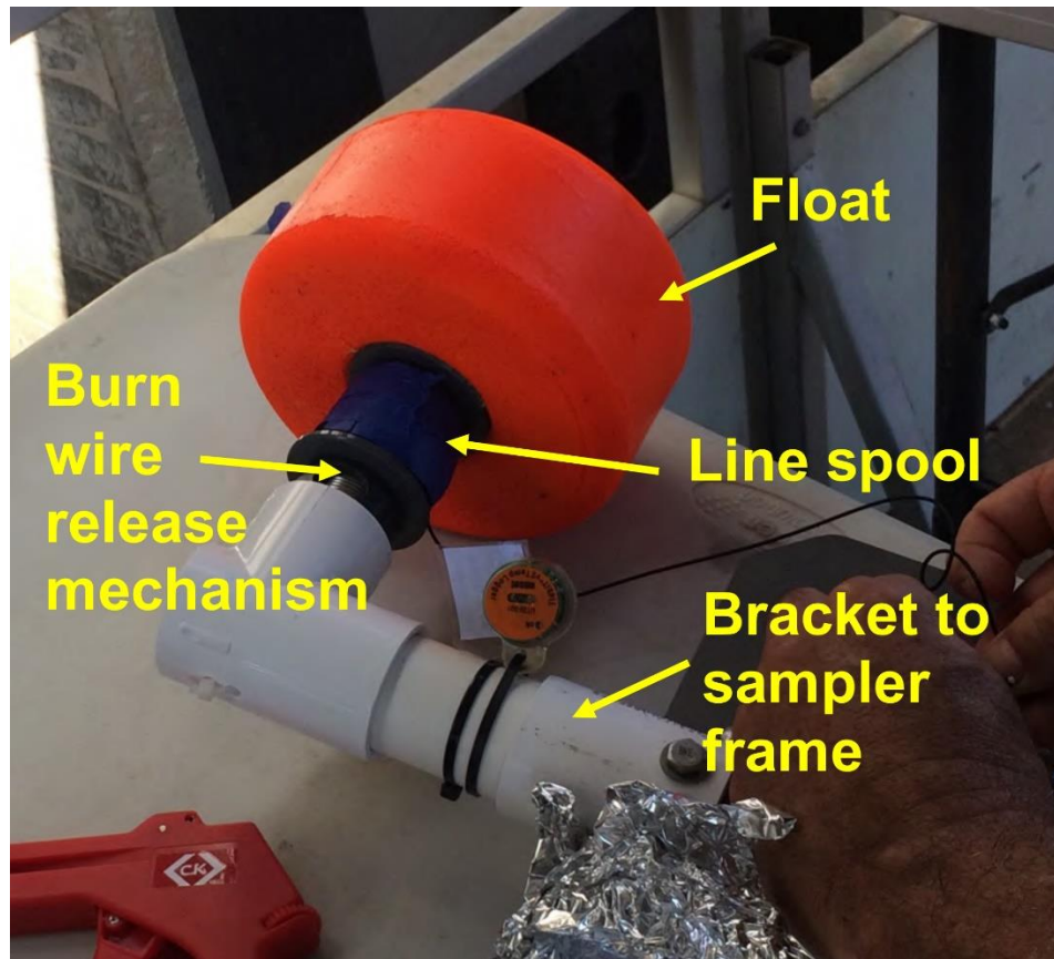
Figure 4 The timed-release retrieval float attached to a passive sampling frame.
