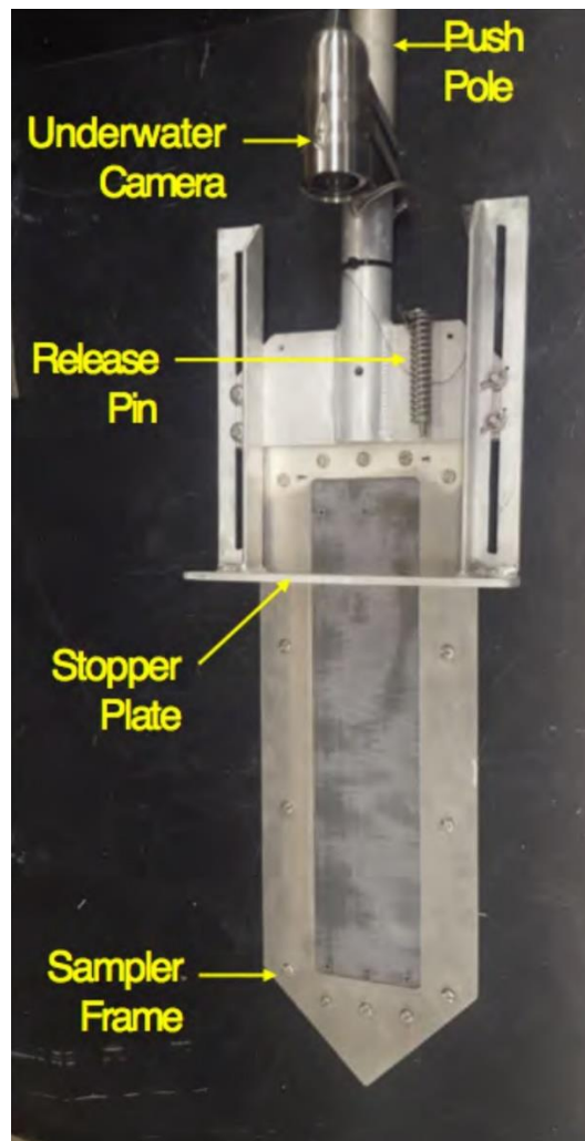
Figure 2 Push pole system.
