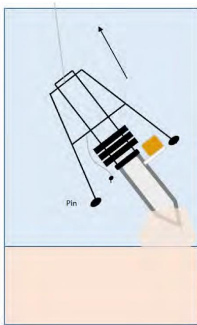
Figure 9 If the boat cannot maintain position over the sampler deployment location, the frame may be pulled back up at an angle, preventing the release of the sampler despite release of the cotter pin.
