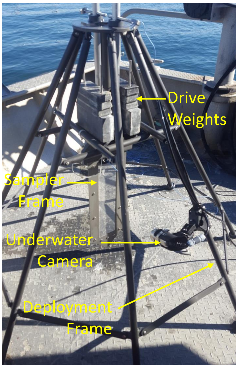
Figure C-3. Drive-frame system.
