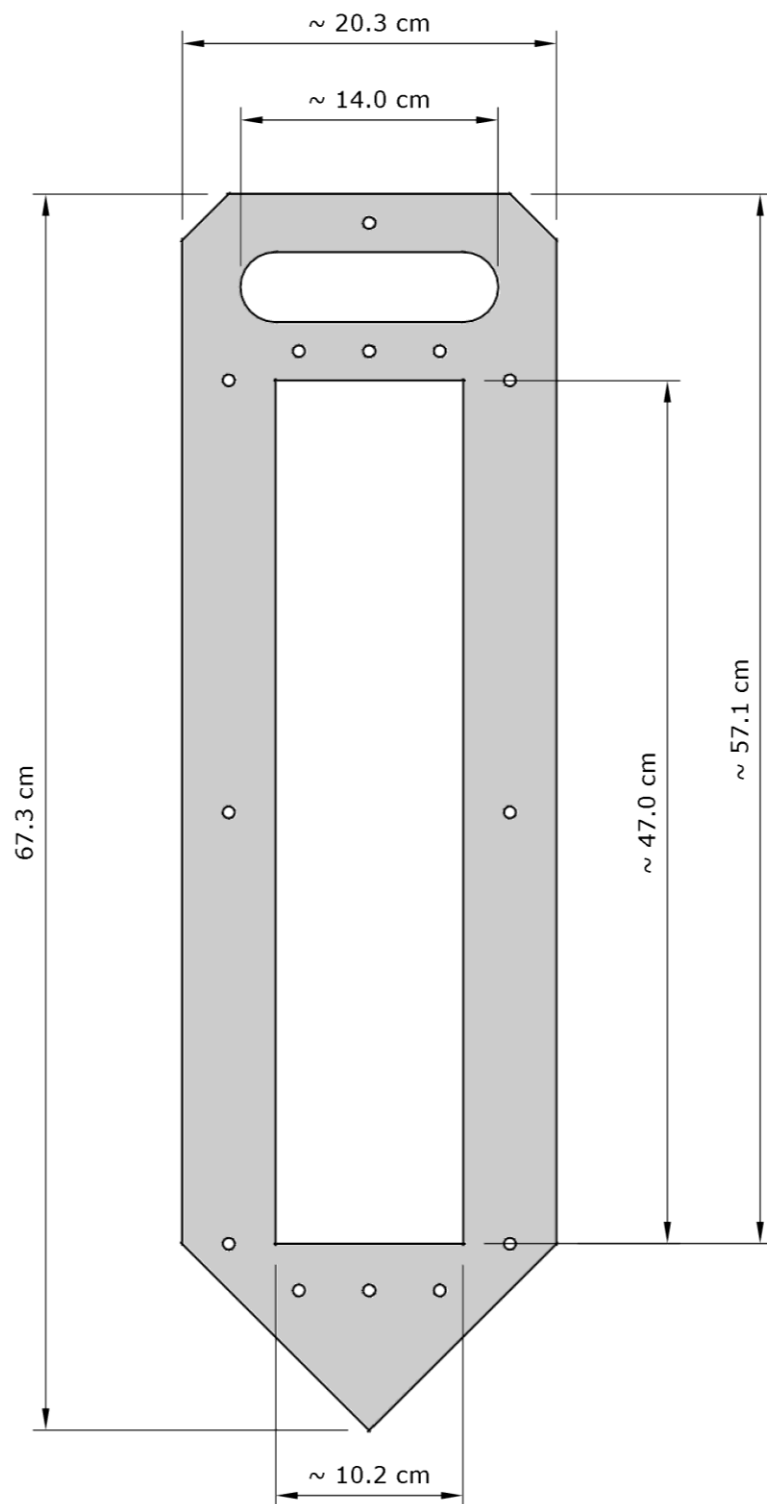
Figure C-1 Passive sampler frame.
