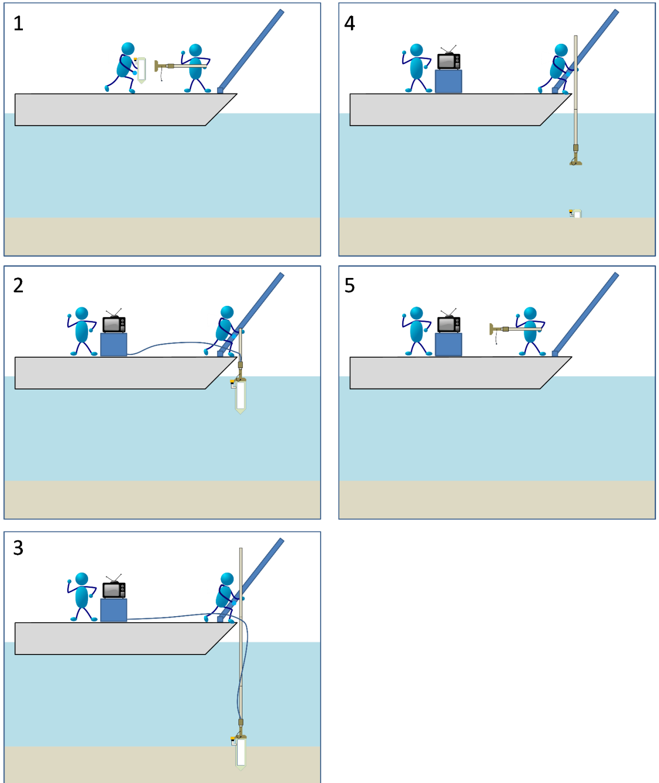
Figure 16 Deployment cartoon for the Passive Push push-pole deployment system.
