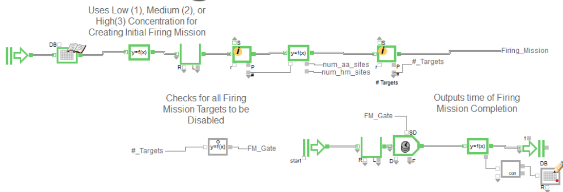
Figure 25. Creation of Initial Firing Mission with Ability to Output time of Completion
