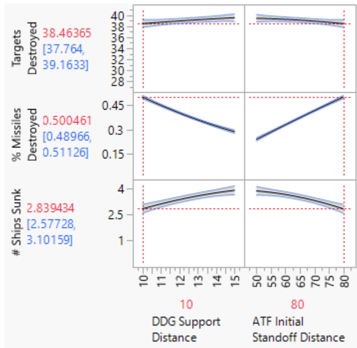
Figure 20. COA1 (Medium Enemy Concentration) Input Factor Prediction Profiler for Desired Responses
