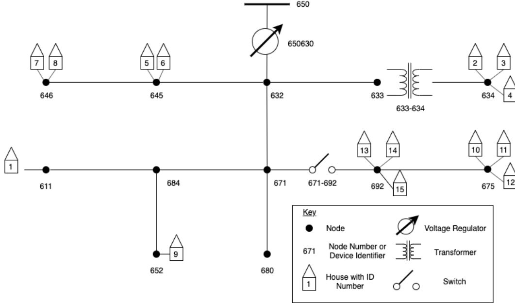
Figure 1. The IEEE 13-Node Model With Houses. Adapted from [47].
