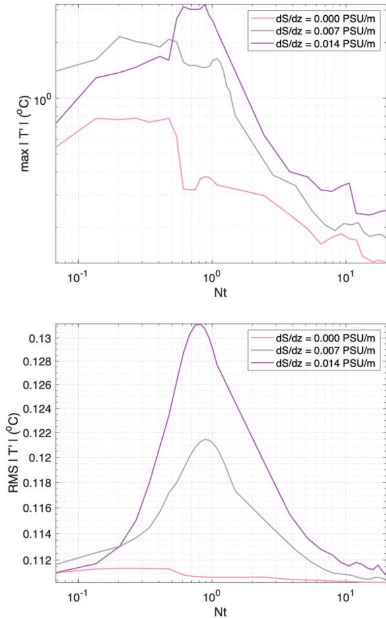
Figure 9. The top plot shows the maximum |T'| as a function of non-dimensional time, Nt , while the bottom plot compares the RMS |T'| as a function of non-dimensional time for various \frac{\partial \bar{s}}{\partial z} runs.
