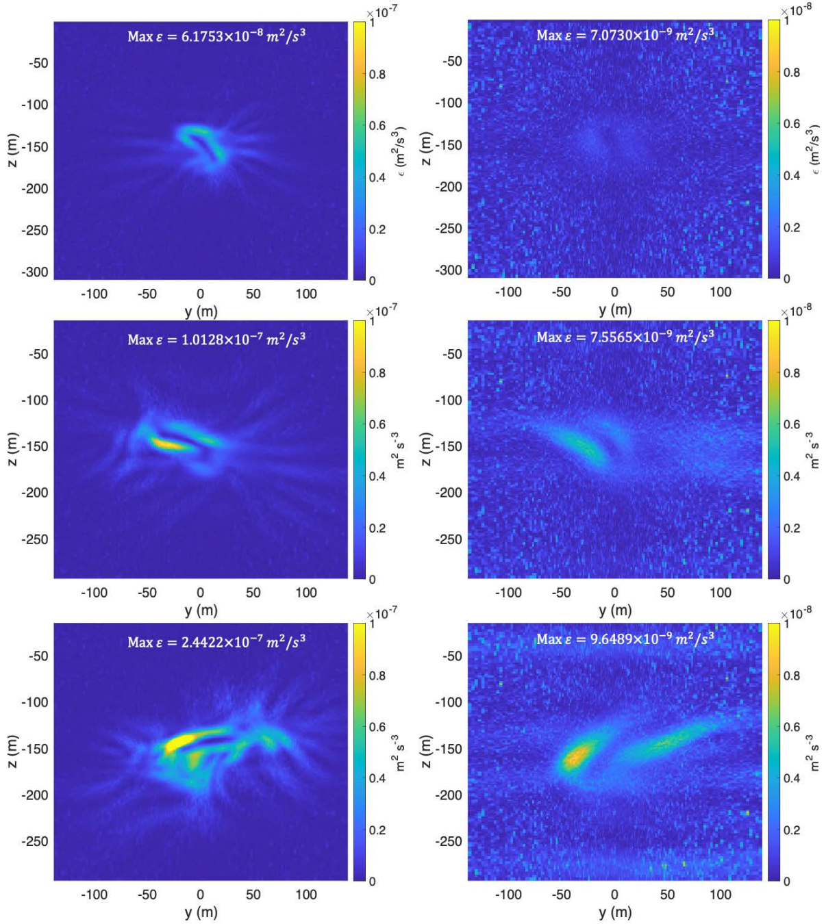
Figure 12. The left and right column show slices of \epsilon taken at Nt \sim 5 , and 20 , respectively. The top, middle and bottom rows are for Q of 0W , 2.2 \times 10^9 W and 4.4 \times 10^9 W , respectively.
