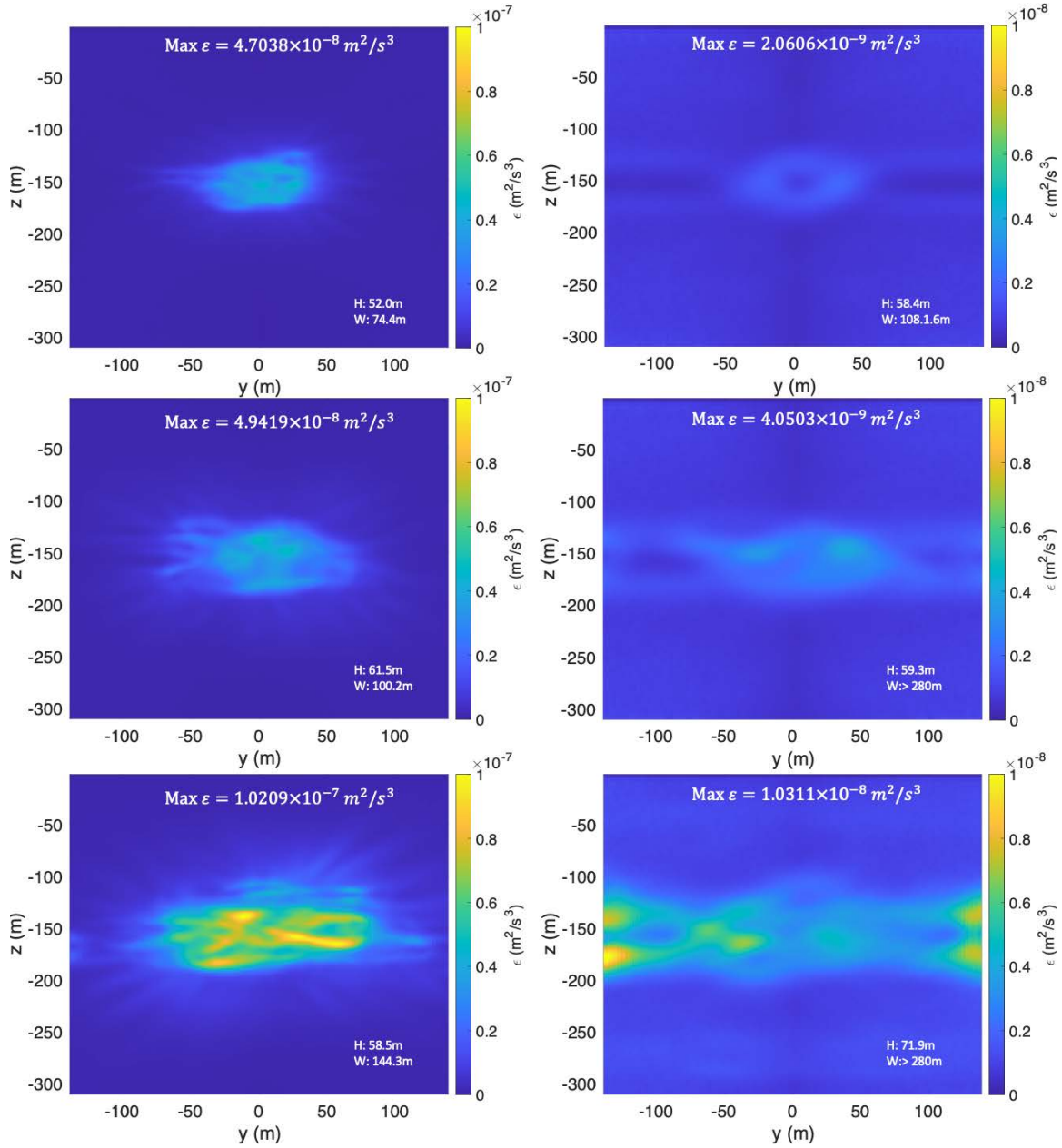
Figure 13. The left and right column show the \epsilon taken at Nt \sim 5 and Nt \sim 20 , respectively. The top, middle and bottom rows are for u_0 of 2.5m/s, 5.0m/s and 10m/s, respectively. The height and width of the area with elevated \epsilon is shown in bottom right of each plot.
