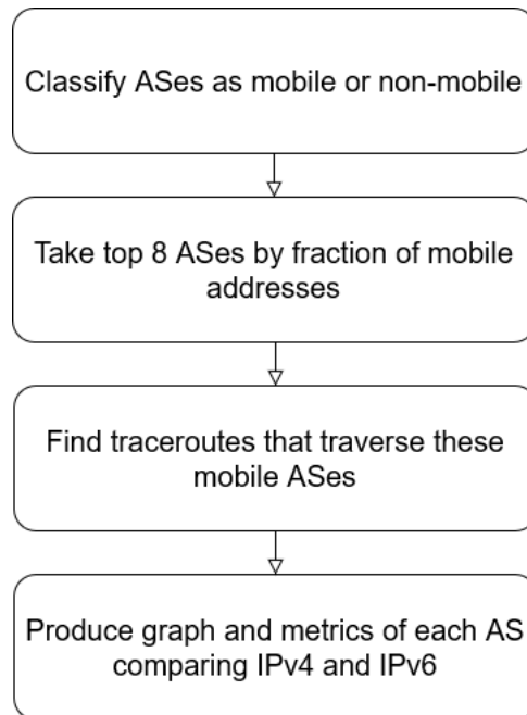
Figure 3.1. Methodology Flowchart.
