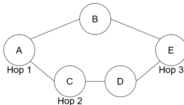
Figure 2.1. Traceroute Example.
