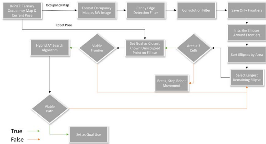
Figure 21. Frontier Search Algorithm
