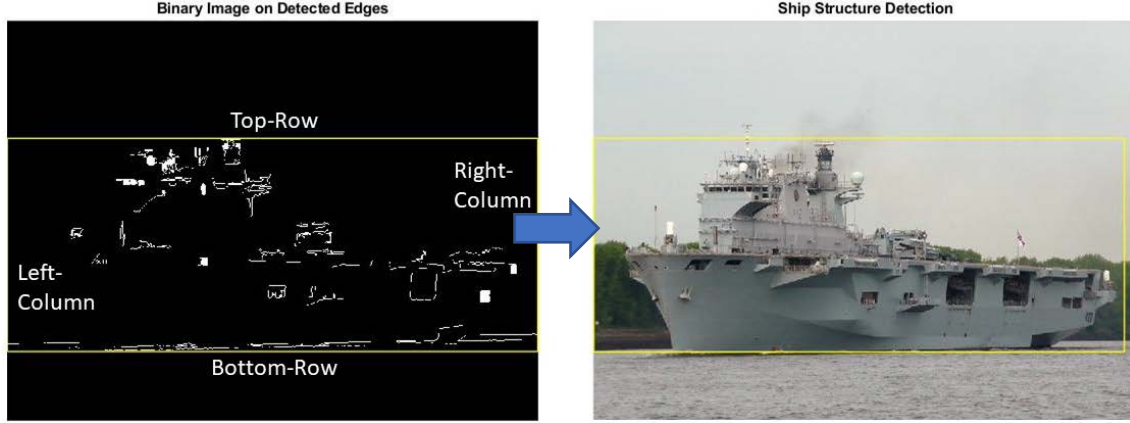
Figure 13. Estimated boundaries of ship structure
