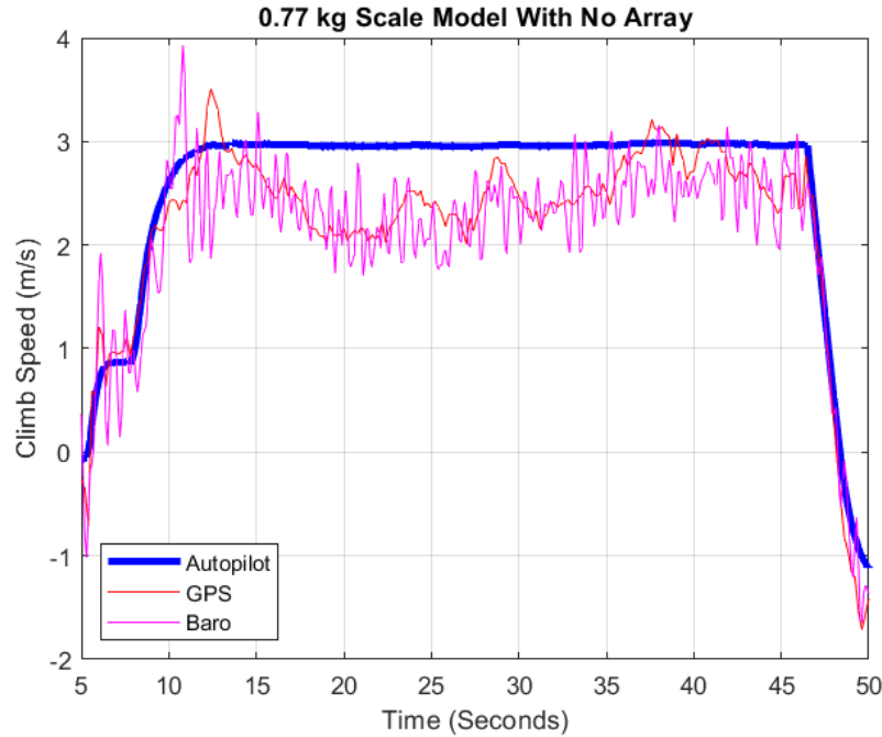
Figure 21. Speed Fluctuations for Commanded Constant-Speed Climb
