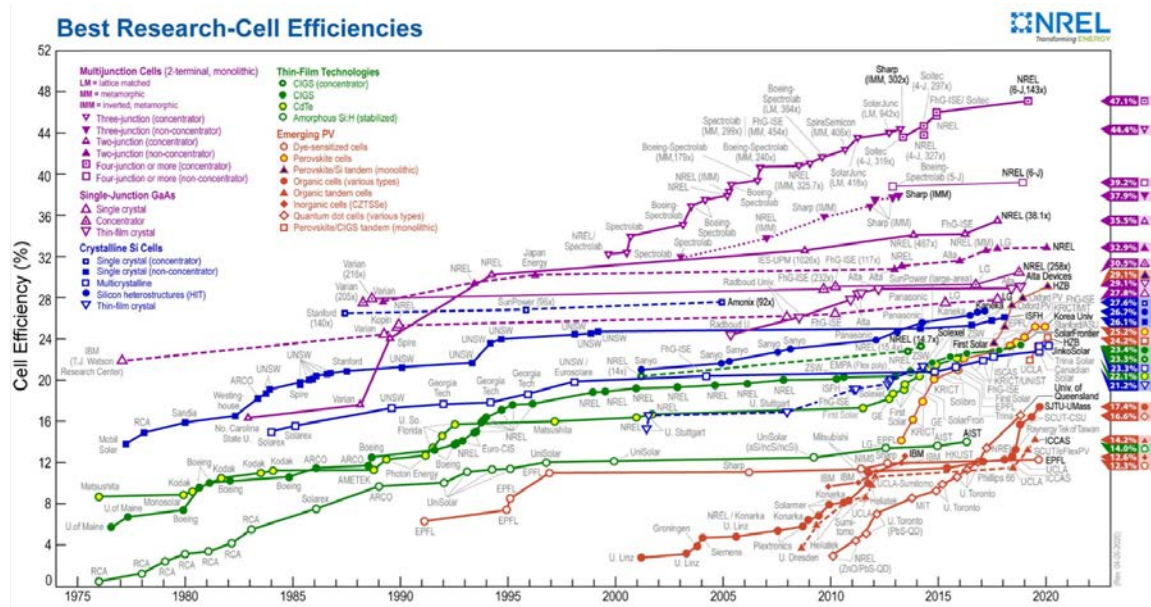
Figure 6. Improvements in Solar Cell Efficiency. Source: [9].
