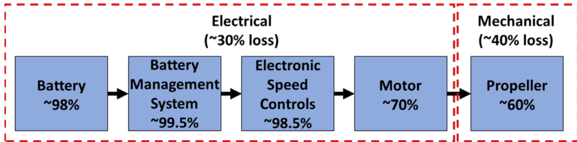
Figure 12. Aqua-Quad Energy Flow and Losses
