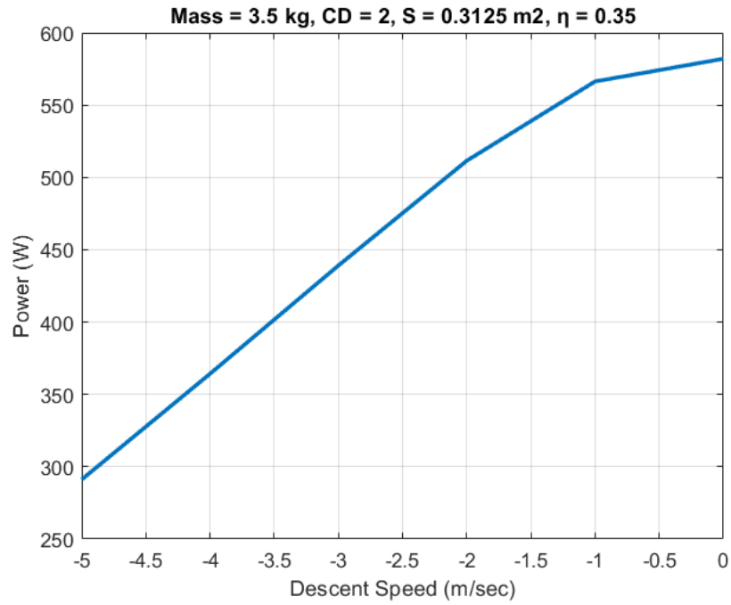
Figure 71. Descent Power Required for Aqua-Quad
