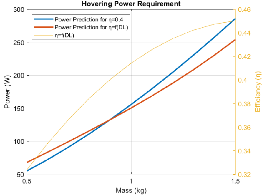
Figure 15. Hovering Power Profiles Corrected for Efficiency
