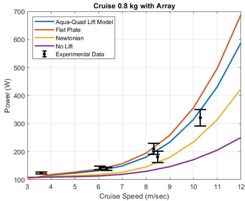
Figure 57. Comparison of Lift Models for Cruise Power Prediction
