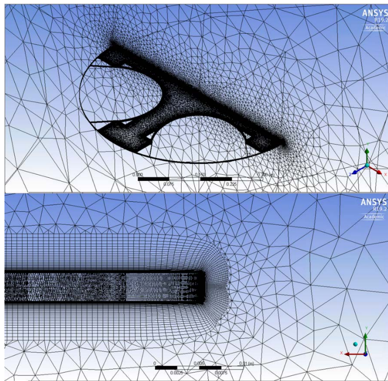
Figure 27. Mesh Generated in ANSYS CFX for Aqua-Quad Solar Array
