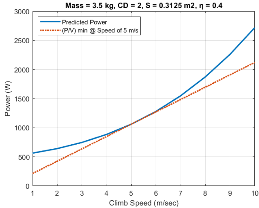
Figure 70. Climb Power Required for Aqua-Quad
