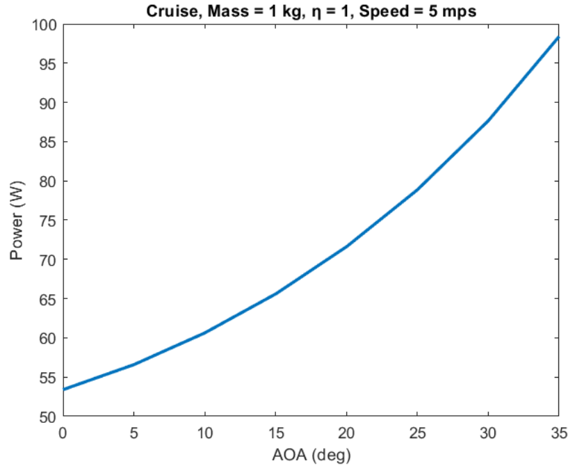
Figure 48. Angle of Attack Impact on Power for Constant Cruise Speed
