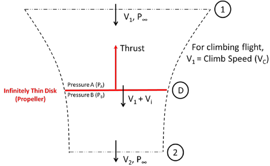
Figure 18. Control Volume for Actuator Disk Theory (Climbing Flight)
