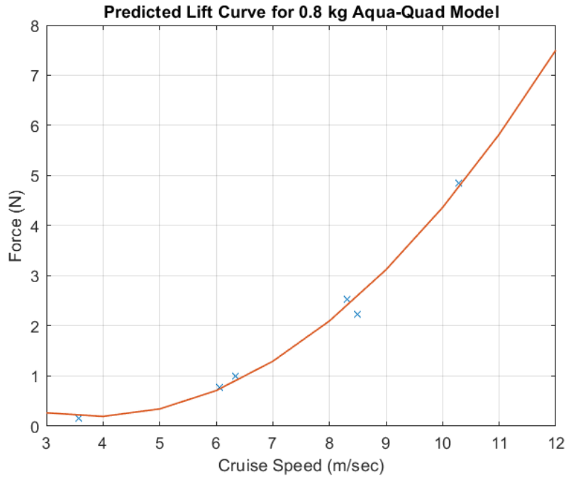
Figure 51. Predicted Lift for Scale Model Aqua-Quad
