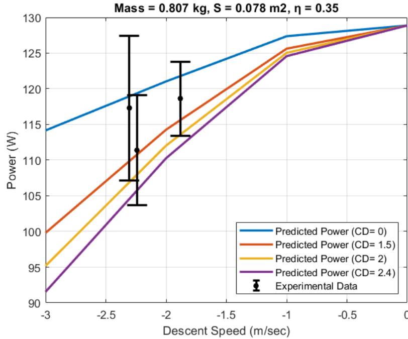
Figure 43. Theoretical Power Descent Model for Different Drag Coefficients Compared against Experimental Data
