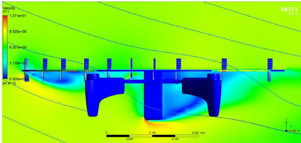
Figure 66. Side View of the CFD-simulated Velocity Field around the Detailed Aqua-Quad in Cruise
