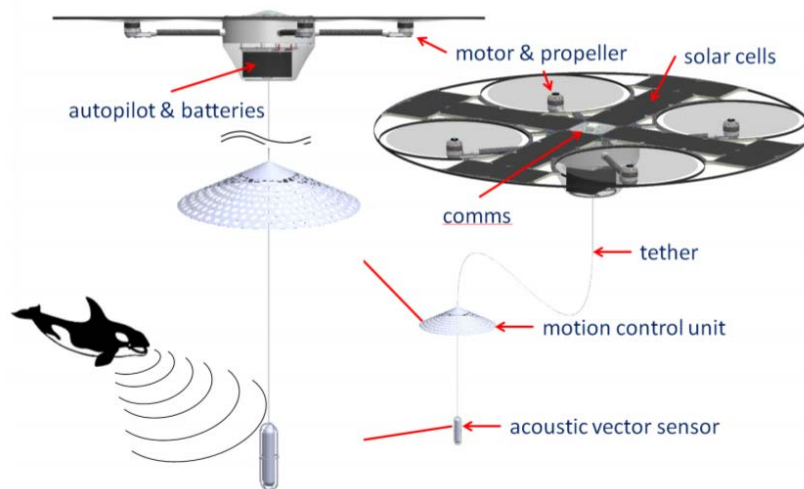
Figure 9. Aqua-Quad Conceptual Design. Source: [1].
