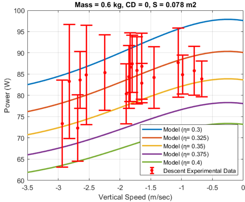
Figure 42. Estimating Efficiency during Quadrotor Descent
