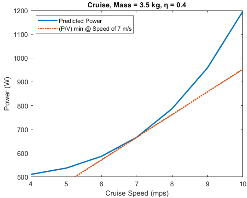
Figure 72. Cruise Power Required for Aqua-Quad
