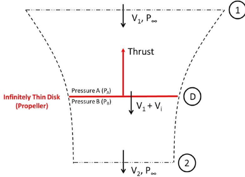
Figure 10. Control Volume for Actuator Disk Theory
