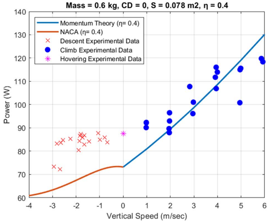
Figure 37. Theoretical Power Models for Descent Compared against Experimental Data
