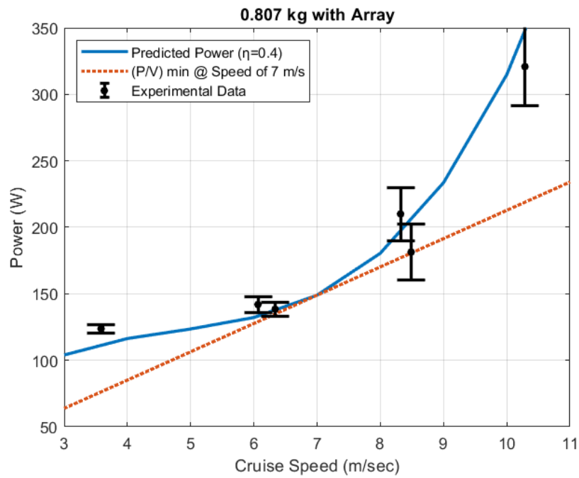
Figure 56. Cruise Power for 0.807 kg Aqua-Quad Model
