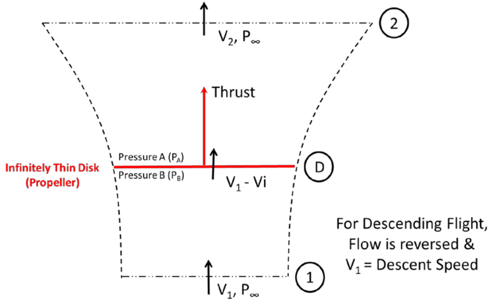
Figure 33. Control Volume for Actuator Disk Theory (Descending Flight)
