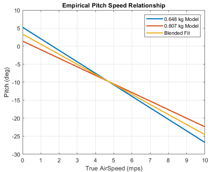
Figure 67. Empirical Relationship of Pitch and Speed
