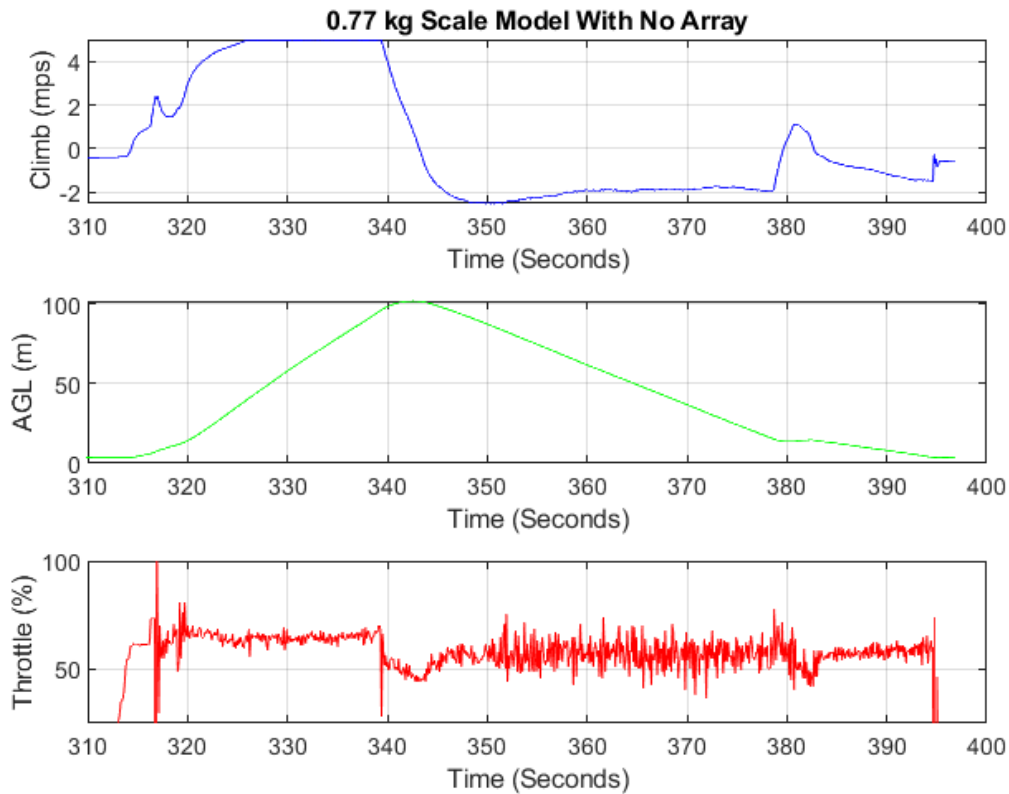
Figure 38. Throttle Response during Climb and Descent
