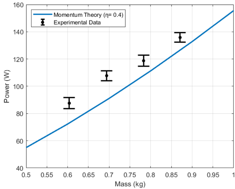
Figure 16. Hovering Power for Scale Model Aqua-Quad
