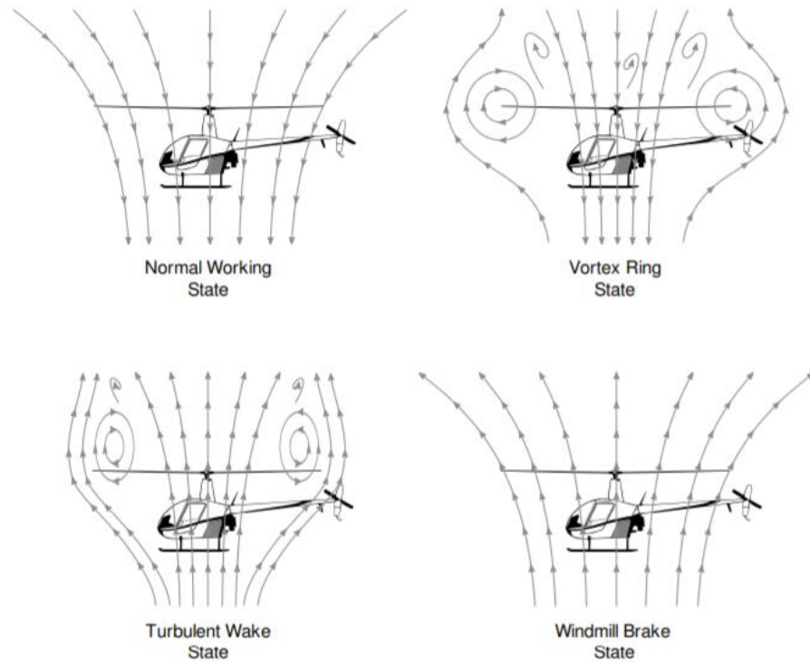
Figure 32. Illustration of Four Primary Operation States for a Helicopter Propeller. Source: [21].
