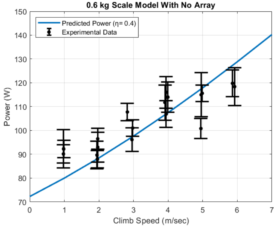
Figure 23. Climb Power Comparison for 0.6 kg Scale Model Aqua-Quad
