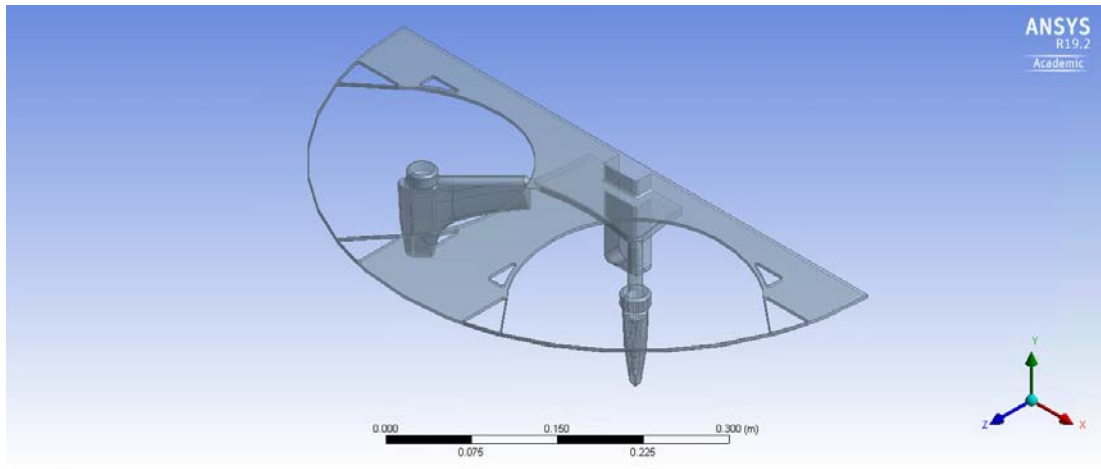
Figure 29. Detailed CAD Model of Aqua-Quad
