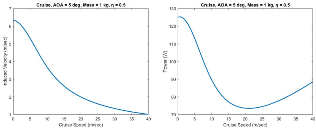
Figure 47. Actuator Disk Theory: Induced Velocity and Power for Cruise Flight at Constant Angle of Attack
