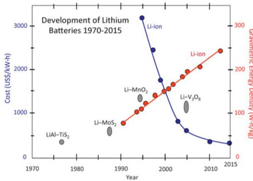
Figure 5. Lithium Ion Battery Improvements. Source: [7].
