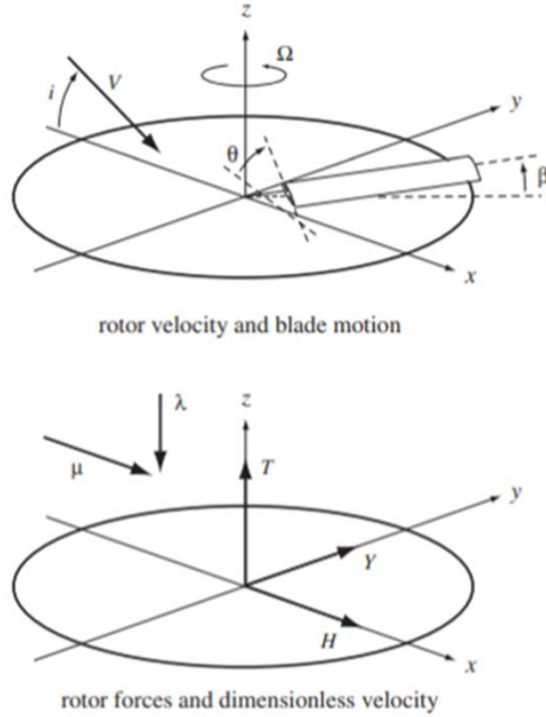
Figure 60. Rotor Forces in Cruise. Source: [19].
