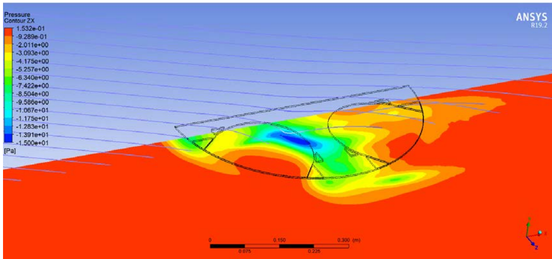
Figure 63. Overhead View of the CFD-simulated Pressure Field of the Simplified Aqua-Quad CFD in Cruise
