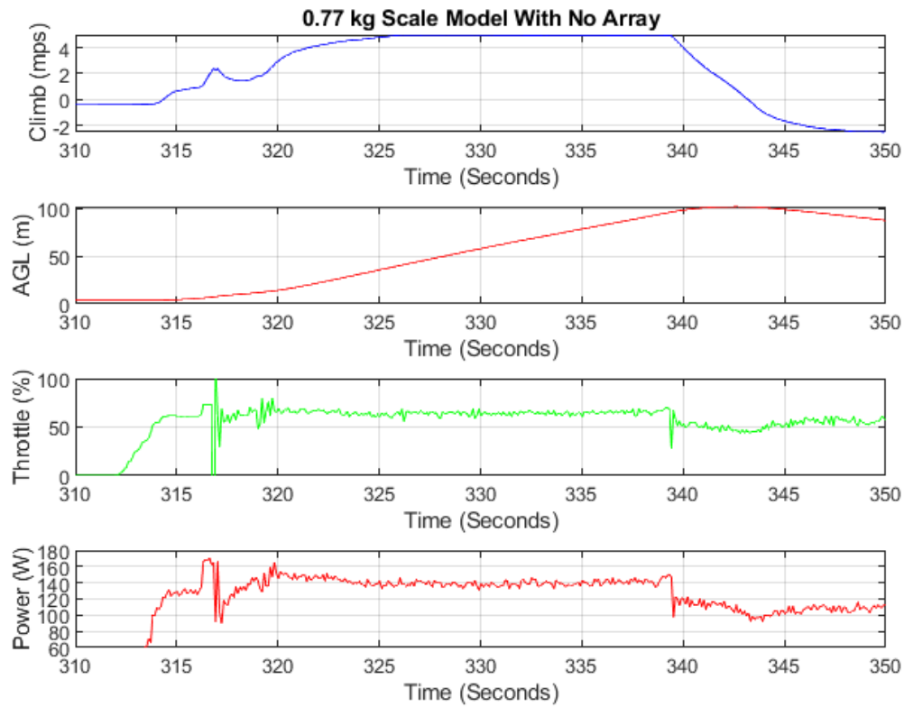
Figure 22. Throttle and Power Response for Constant Speed Climb
