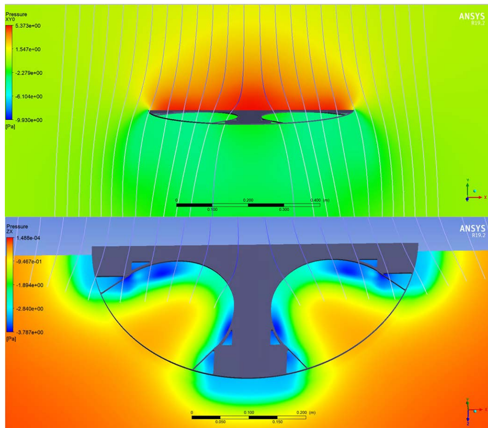
Figure 28. CFD-simulated Pressure Distribution around the Solar Array in Vertical Flight
