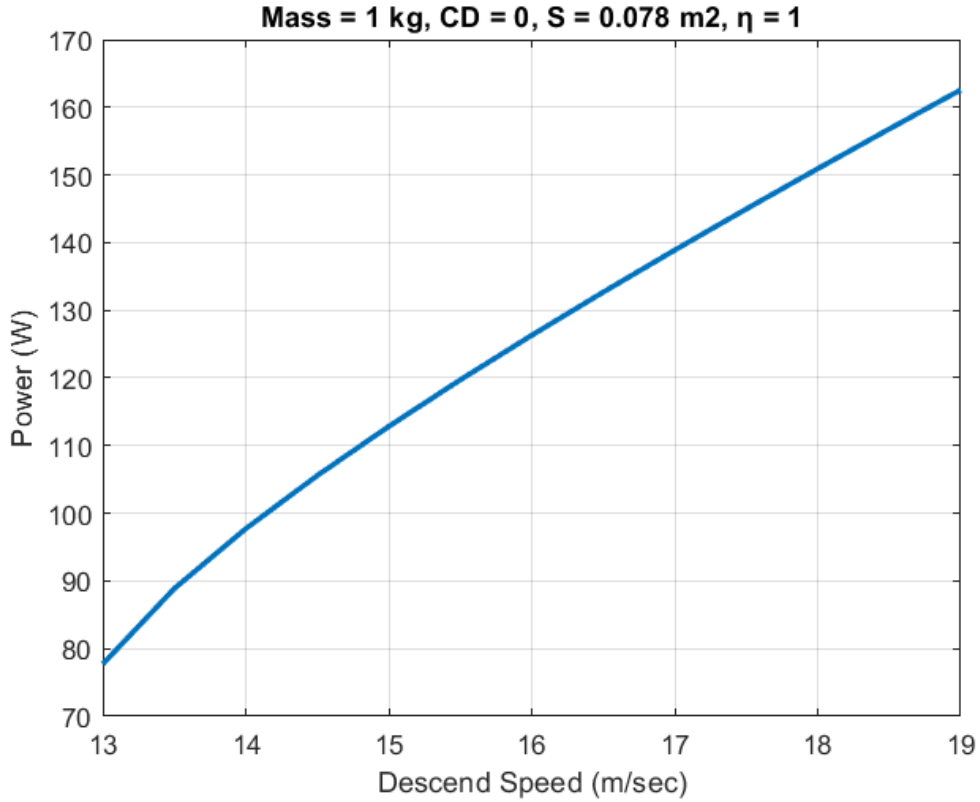
Figure 34. Power Extracted by the Propeller in Windmill Brake State
