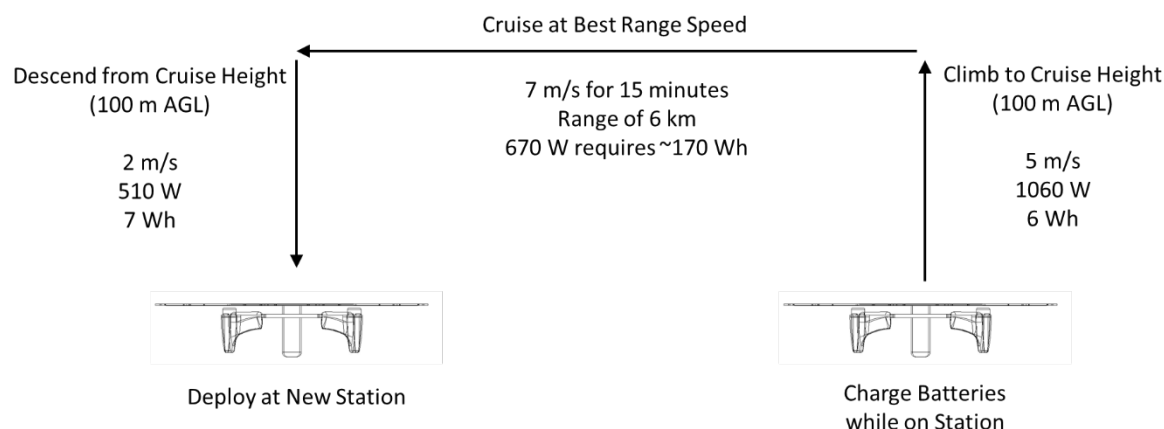
Figure 73. Power Demands during Aqua-Quad Flight Profile
