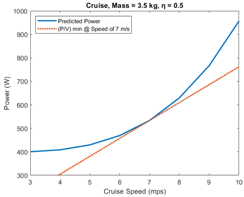
Figure 69. Cruise Power Required for Full-Scale Aqua-Quad (Efficiency Factor of 0.5)
