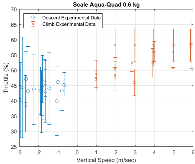
Figure 39. Throttle Mean and Standard Deviation for Various Vertical Speeds
