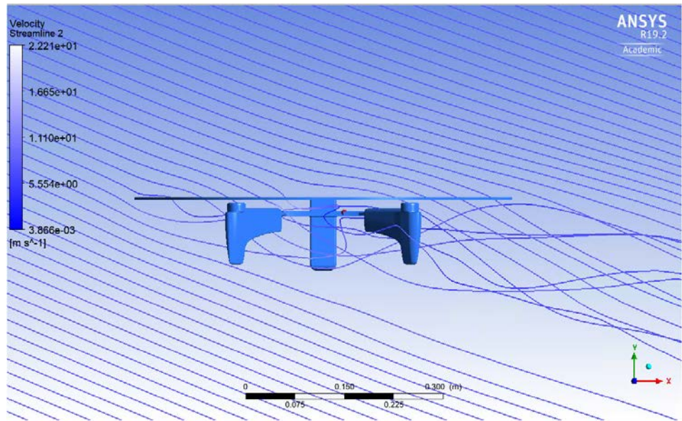
Figure 65. Side View of CFD-simulated Streamlines along the Detailed Aqua-Quad in Cruise
