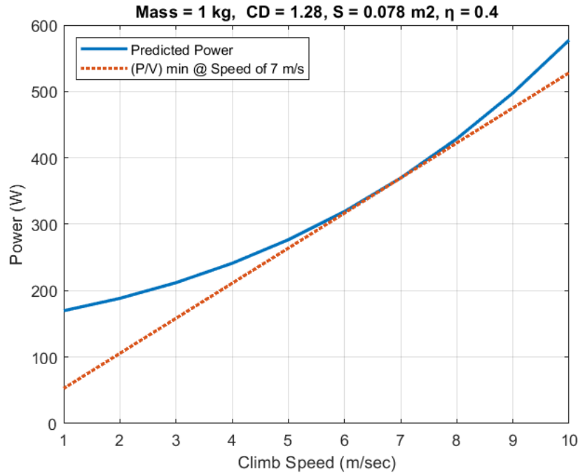
Figure 19. Climb Power for Scale Model of Aqua-Quad
