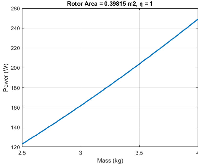
Figure 11. Example of Hovering Power Profile with an Efficiency Factor ( \eta ) of 1.0
