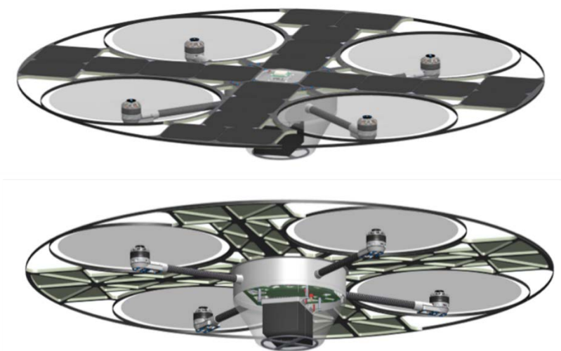
Figure 1. Aqua-Quad Quadrotor, Top and Bottom Views. Source: [1].
