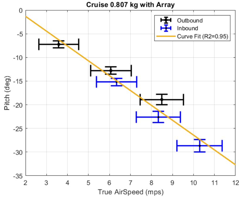
Figure 54. Pitch Angles for Different True Air Speeds
