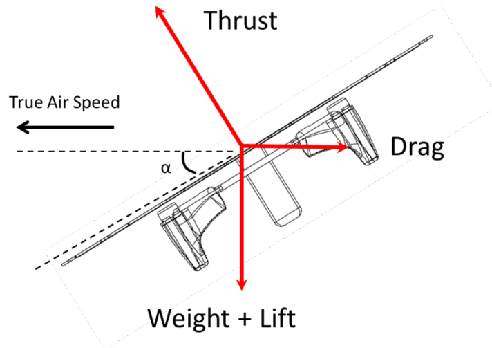
Figure 45. Force Balance of the Aqua-Quad in Cruise
