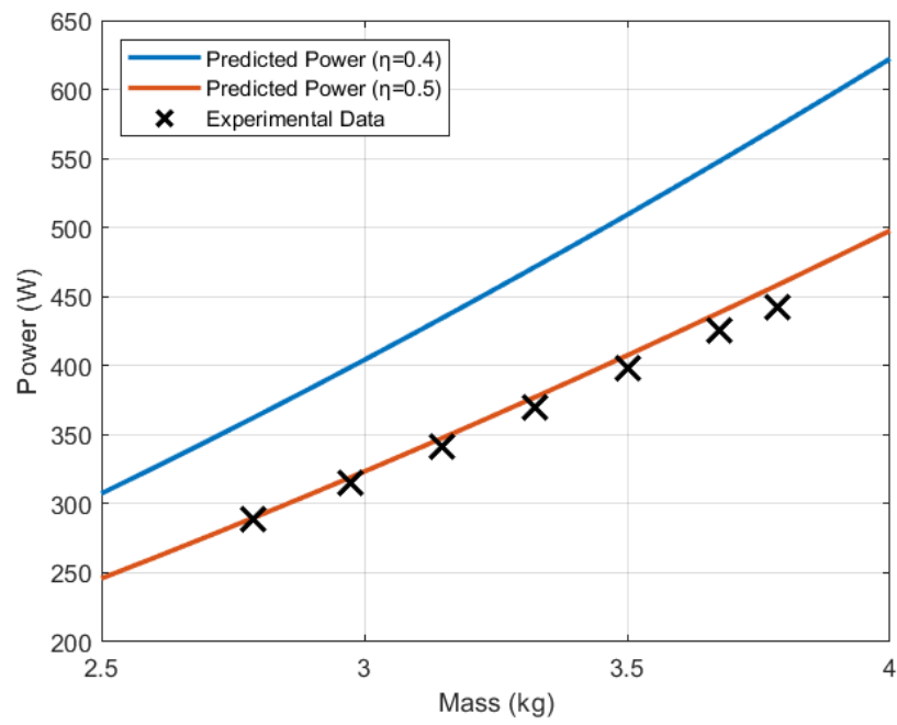
Figure 17. Hovering Power for Full-Sized Aqua-Quad Prototype
