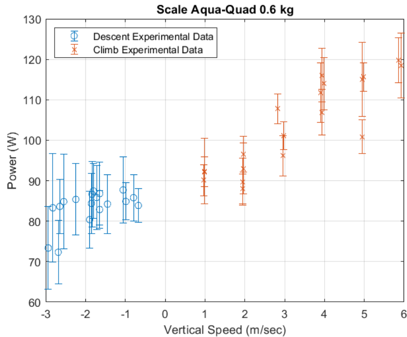
Figure 40. Power Mean and Standard Deviation during Commanded Constant Vertical Speeds
