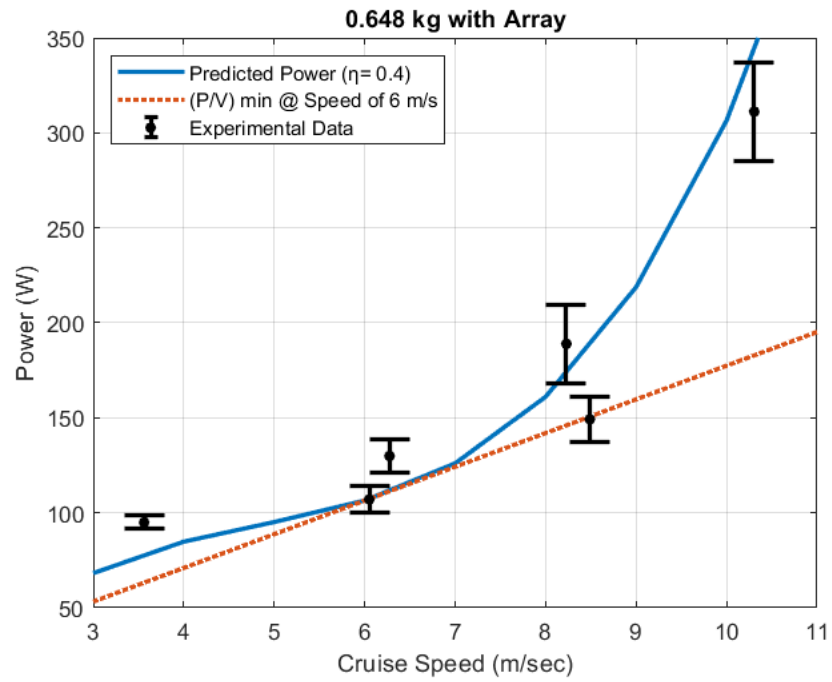
Figure 55. Cruise Power for 0.648 kg Aqua-Quad Model
