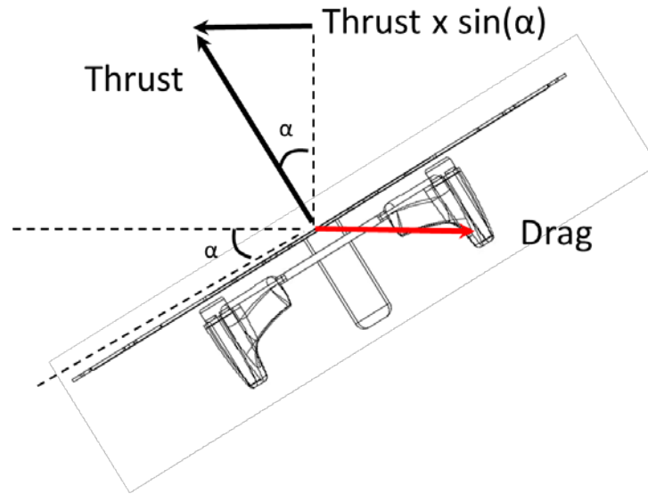
Figure 58. Force Balance during Cruise between Drag and Thrust
