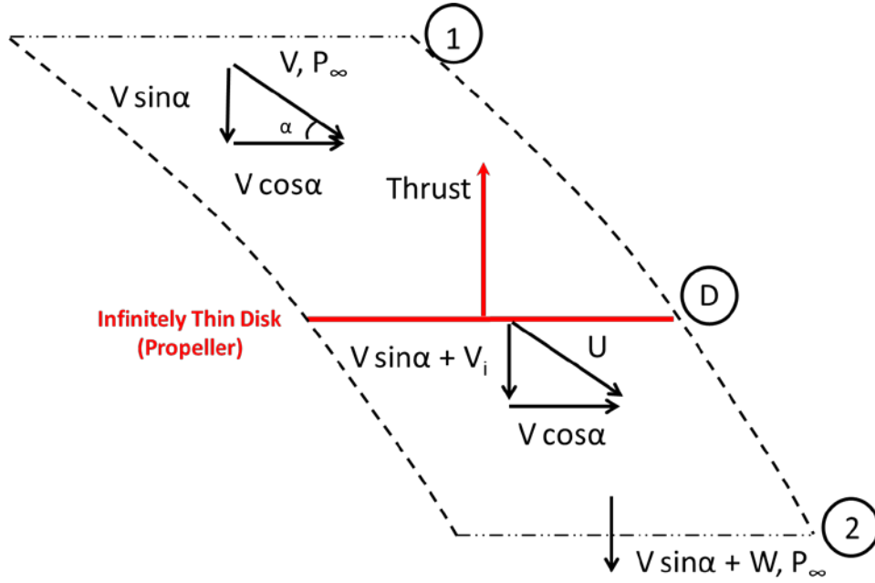
Figure 46. Control Volume for Actuator Disk Theory (Cruise Flight)
