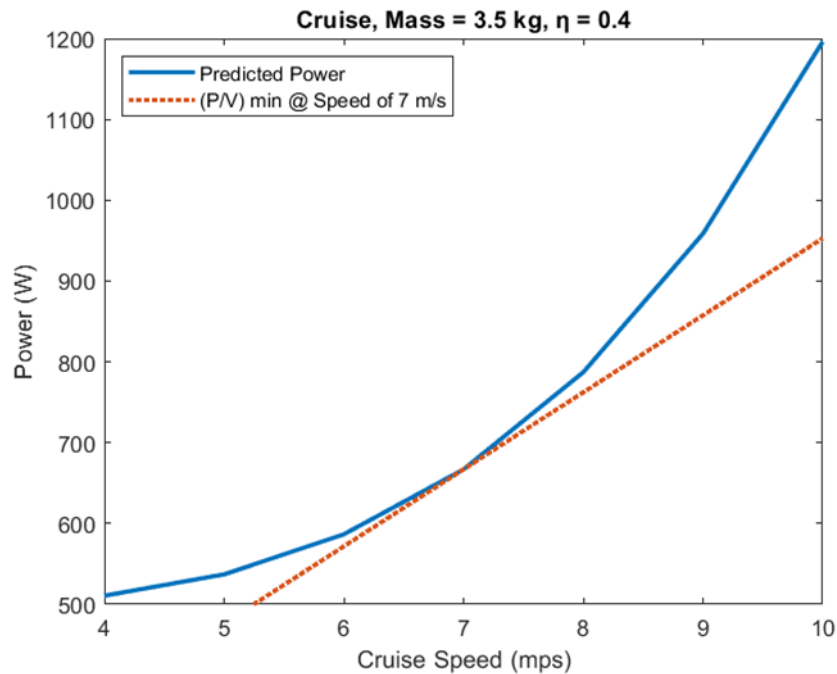
Figure 68. Cruise Power Required for Full-Scale Aqua-Quad (Efficiency Factor of 0.4)
