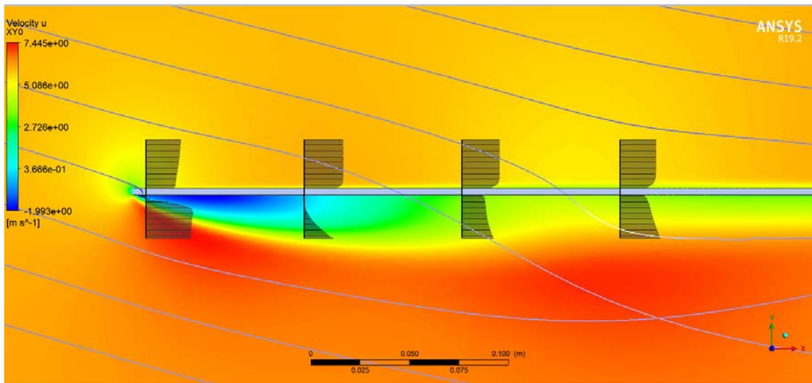
Figure 64. CFD-simulated Flow along the Solar Array in Cruise
