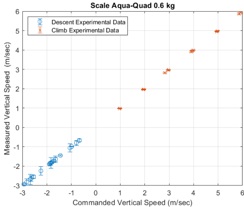
Figure 41. Speed Mean and Standard Deviation during Commanded Constant Vertical Speeds
