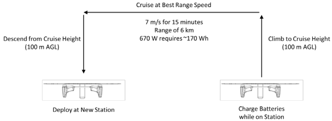
Figure 8. Aqua-Quad Flight Profile
