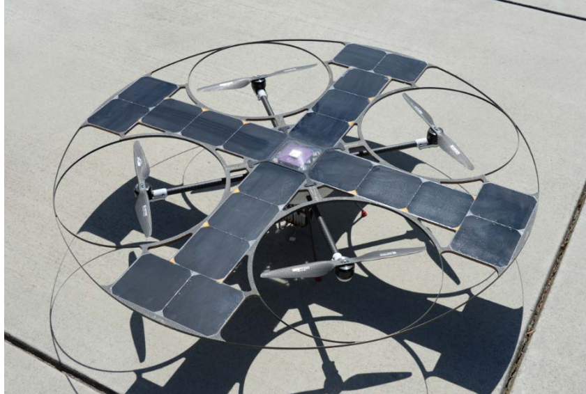
Figure 2. Aqua-Quad Quadrotor Prototype
