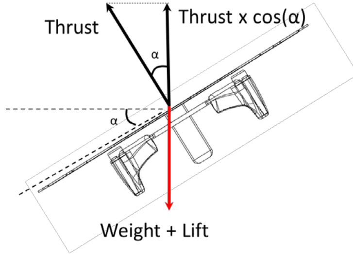
Figure 49. Thrust Required in Cruise
