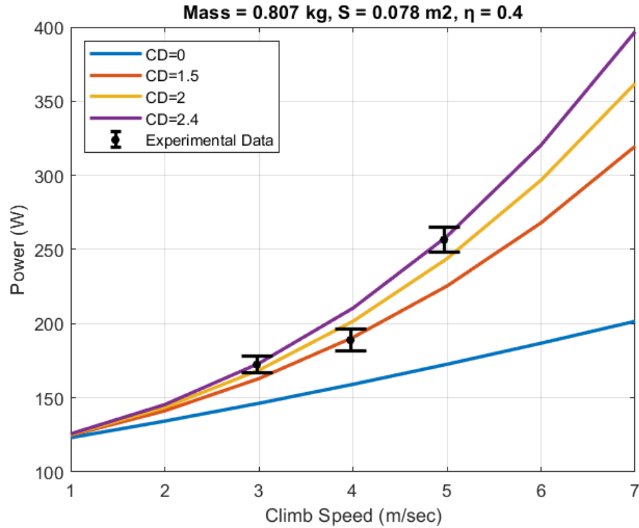
Figure 24. Climb Power Models for Different Drag Coefficients
