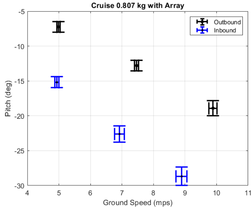
Figure 53. Pitch Angles for Different Commanded Ground Speeds
