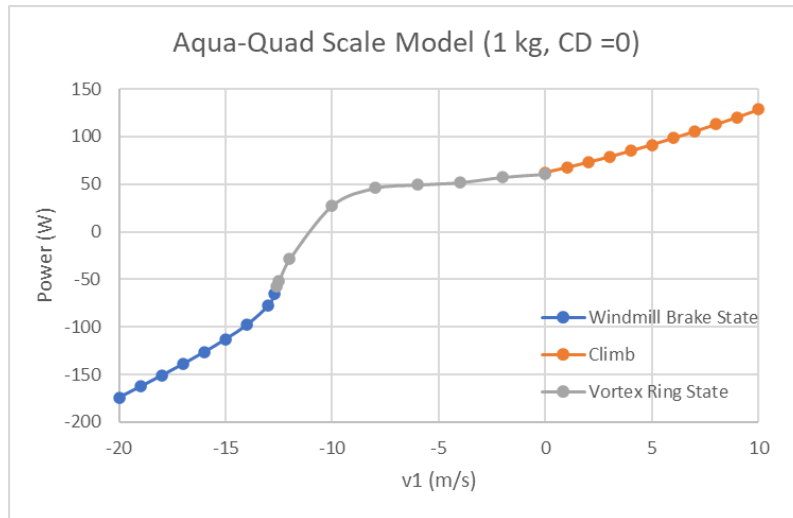
Figure 36. Example of Power Required in Vortex Ring State, Windmill Brake State, and Climb
