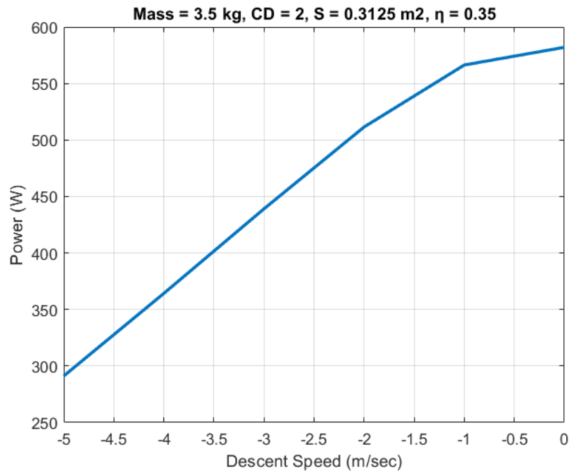
Figure 44. Descent Power Required for Full-scale Aqua-Quad
