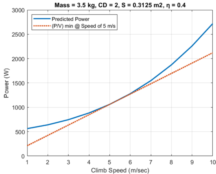
Figure 31. Climb Power Required for Full-scale Aqua-Quad
