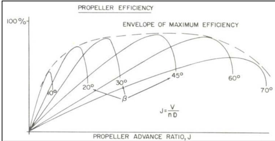
Figure 14. Advance Ratio, Blade Angles, and Propeller Efficiency. Source: [15].
