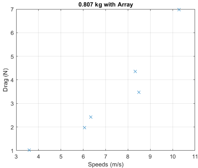
Figure 61. Drag Estimate Based on Experimental Data for 0.8 kg Model (With Solar Array)
