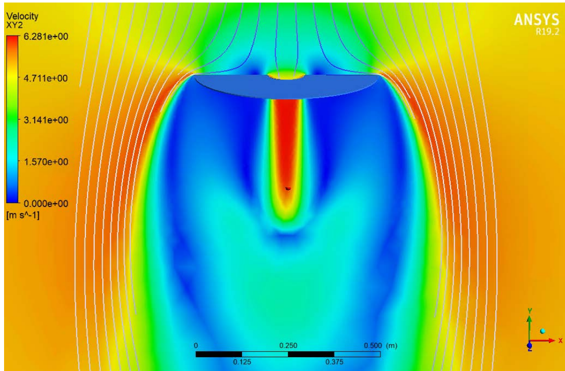
Figure 25. CFD-simulated Velocity Flow Field around a Ring
