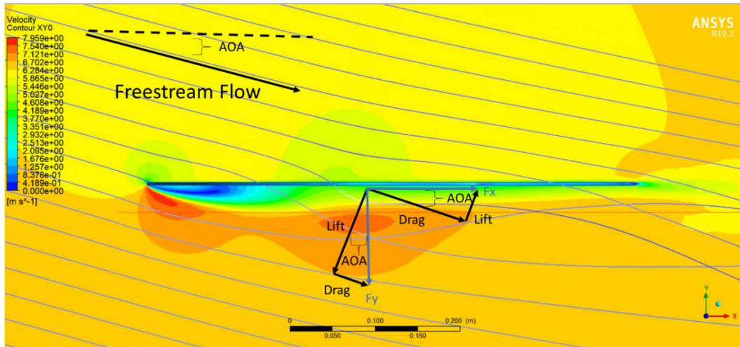
Figure 62. Side Profile of the CFD-simulated Velocity Field of the Simplified Aqua-Quad CFD in Cruise
