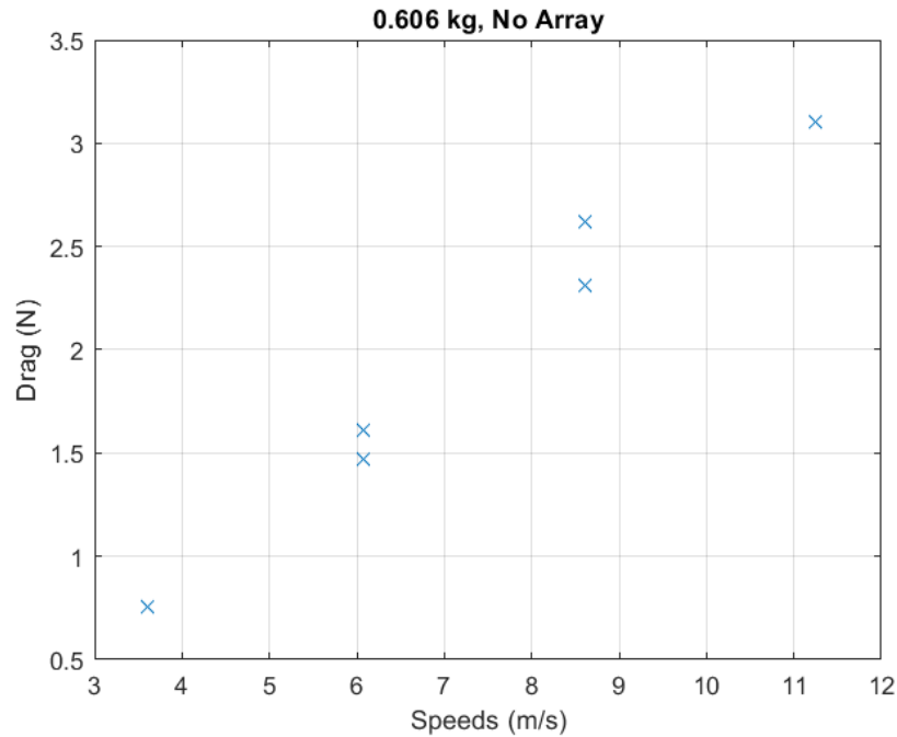
Figure 59. Drag Estimate Based on Experimental Data for 0.6 kg Model (Without Solar Array)
