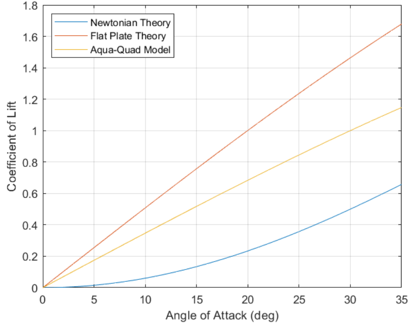
Figure 50. Coefficient of Lift for Different Models
