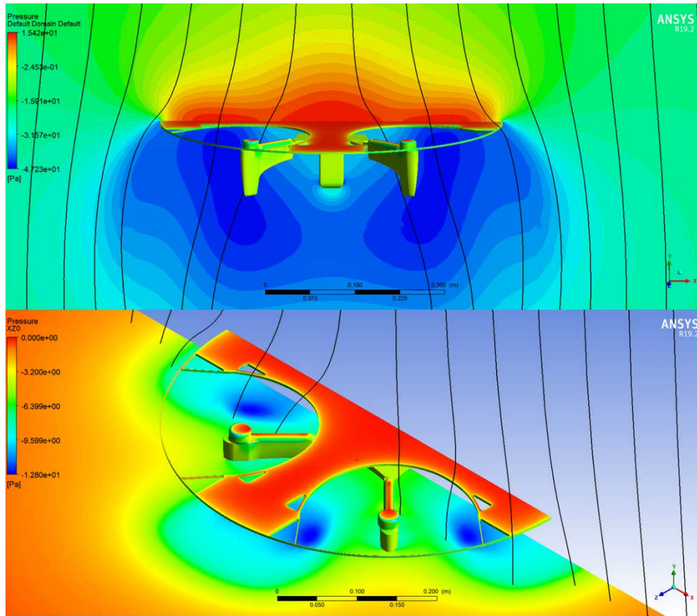
Figure 30. CFD-simulated Pressure Distribution around the Detailed Aqua-Quad Model in Vertical Flight
