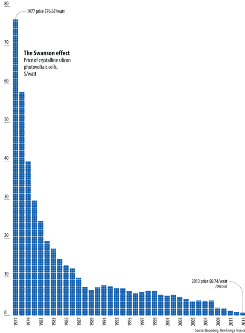
Figure 7. Drop in Price of Photovoltaic Cells. Source: [11].
