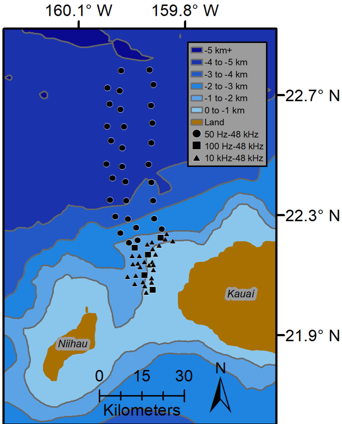
Figure 1. Hydrophone array configuration at PMRF's instrumented range.
