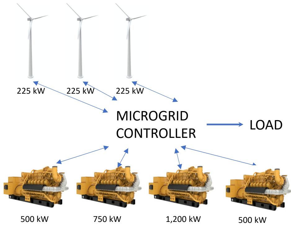
Figure 72. SCI's RE microgrid.
