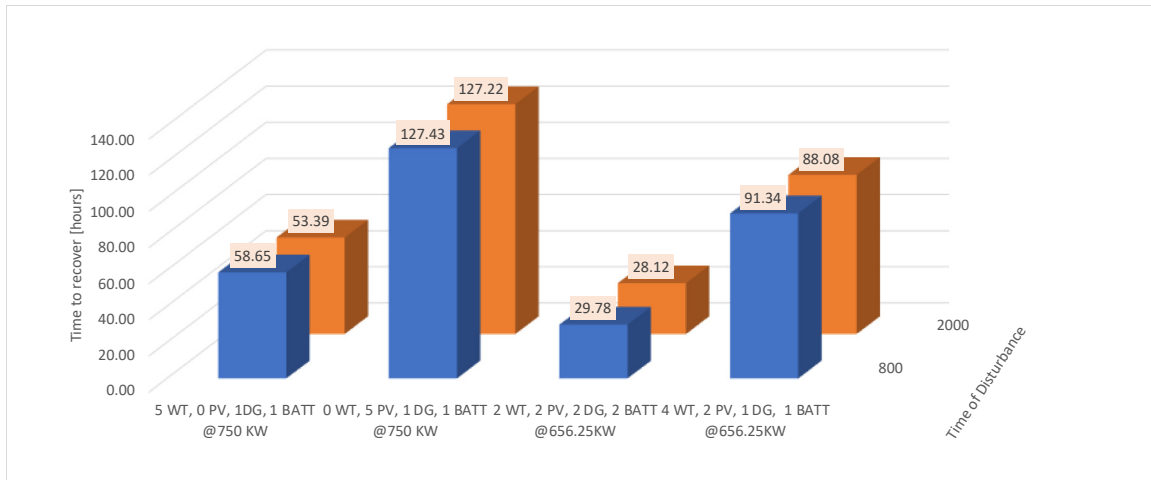
Figure 27. The sensitivity of time to recover to the time of disturbance and ratio of P^{WT}/P and P^{PV}/P .
