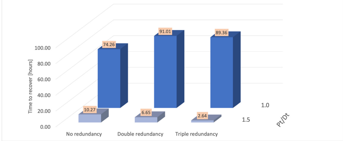
Figure 32. The sensitivity of time to recover to each microgrid ratio of power rating to demand and redundancy level.
