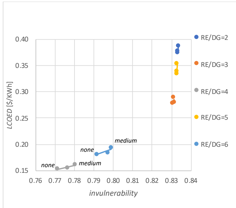
Figure 95. The effects of maintenance level and RE proportion on LCOED and invulnerability .
