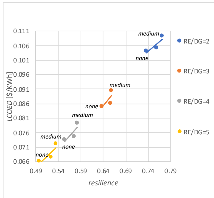
Figure 102. The effects of maintenance level and WT proportion on LCOED and resilience
