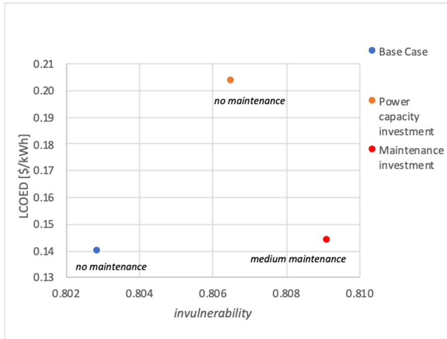
Figure 57. The effects of investing in power rating or maintenance on LCOED and invulnerability .
