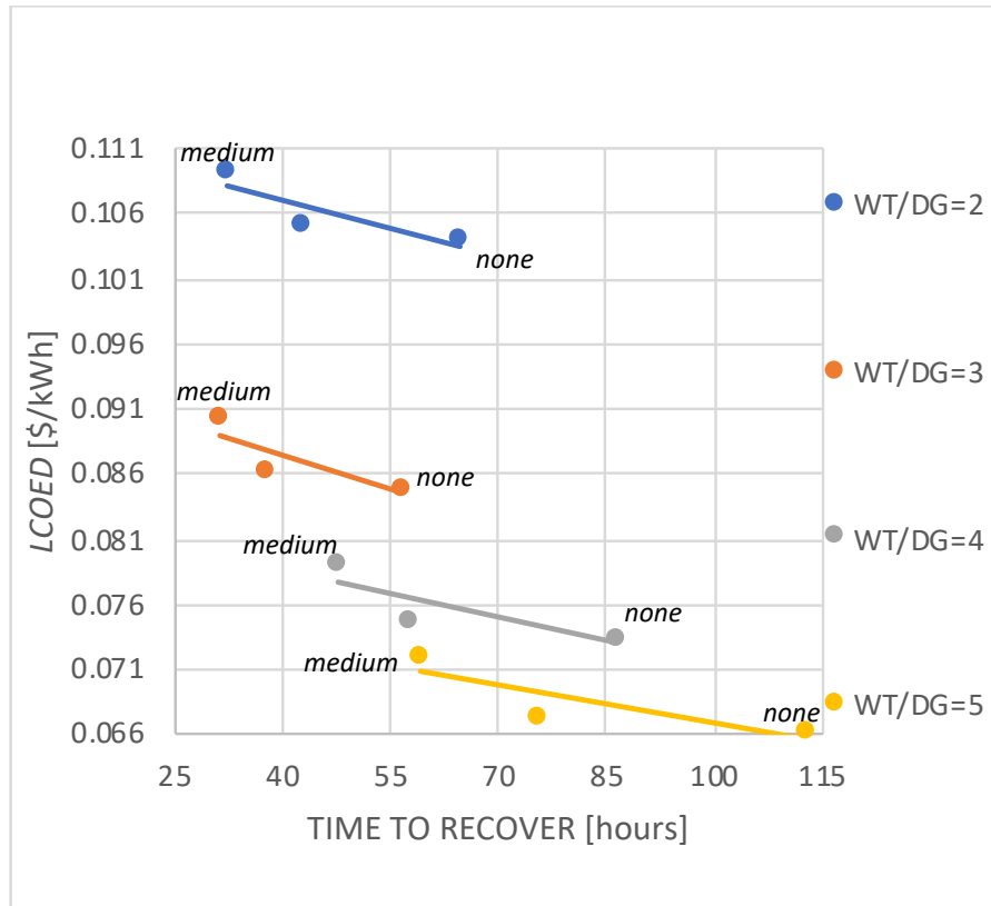
Figure 42. The effects of maintenance level and WT proportion on LCOE and time to recover.
