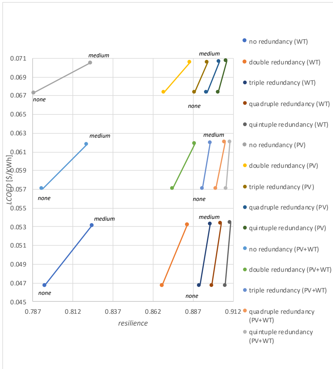
Figure 114. The effects of PV and WT redundancy on LCOE and resilience.
