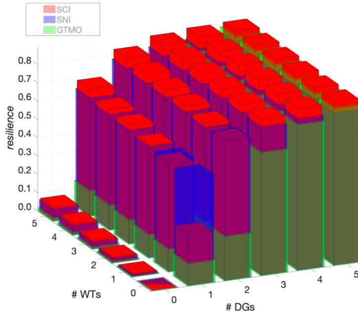
Figure 84. Resilience vs. # of WTs and DGs for SCI, SNI, and GTMO.
