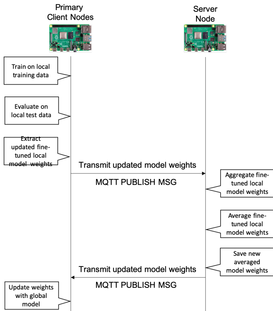
Figure 30. Federated Training Round Cycle for Experiments II-V.
