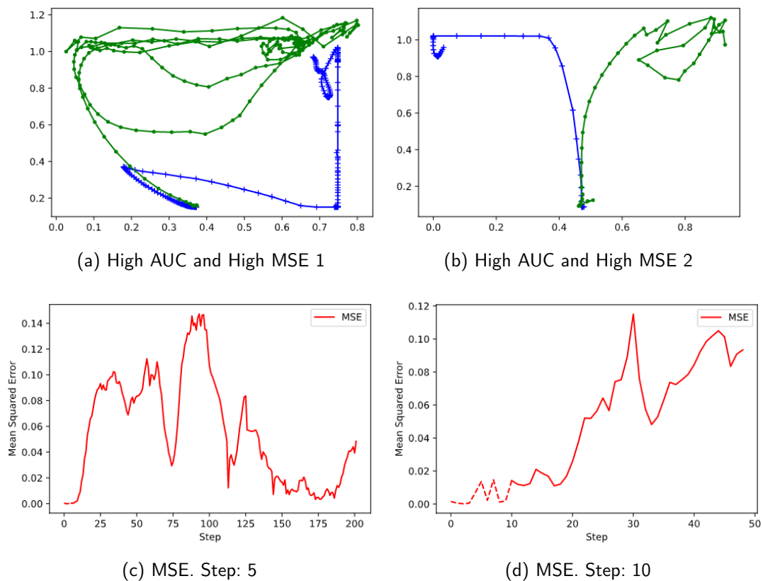
Figure 4.8. Example High AUC and High MSE Ground Truths And Predictions.
